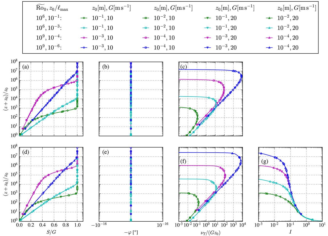
Figure 3. Reynolds number similarity of the proposed ABL model without wind veer for two turbulence closures. (a–c) Mixing-length model. (d–g) k-\epsilon model.
