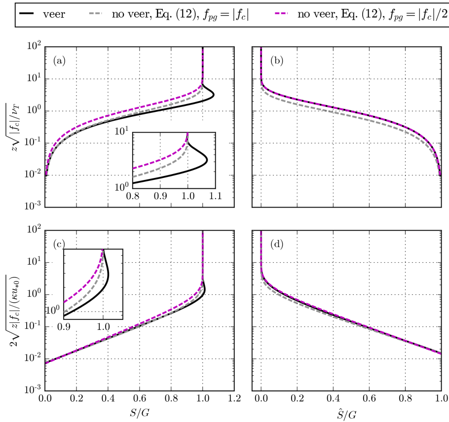
Figure 1. Analytic solutions with and without wind veer. (a, b) Constant v_T . (c, d) Linear v_T and Ro_0 = 10^5 . (a, c) Wind speed. (b, d) Ageostrophic wind speed.
