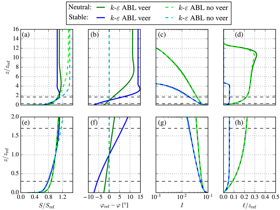
Figure 5. Comparison of k-\varepsilon ABL models (with and without wind veer) for stable and neutral conditions offshore using f_c \neq 2f_{pg} and parameters from Table 1. Bottom plots (e-h) are a magnified view of the top plots (a-d), focused around a 5 MW wind turbine rotor area, which is depicted as black dashed lines. (a, e) Wind speed. (b, f) Wind direction. (c, g) Turbulence intensity. (d, h) Turbulence length scale.
