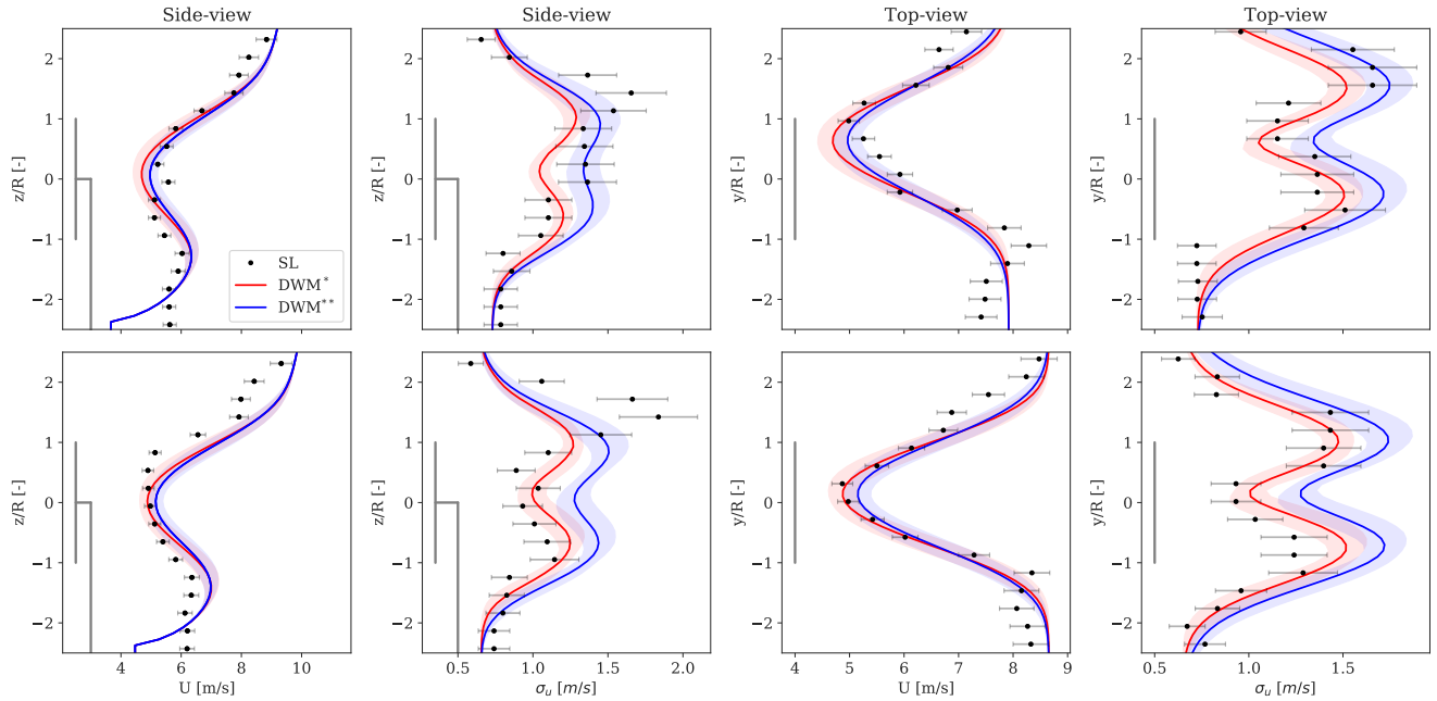
Figure 13. Comparisons between SpinnerLidar-measured (SL) and DWM model-predicted spatial distribution of the mean and standard deviation velocity computed in the FFor and obtained at 5D in the wake region for two 10-min periods. The predictive DWM model that incorporates the SpinnerLidar-tracked meandering time series are denoted by DWM* (red line), and that based on the meandering model complemented with measured inflow turbulence fluctuations from the mast and yaw offsets are denoted by DWM** (blue line). The solid lines represent the mean predictions, whereas the shaded areas indicate the 95% confidence intervals. The uncertainties in measurements are shown with errorbars. The top-view profiles are centered at hub height, whereas the side-view profiles along the vertical symmetry plane of the wake.
