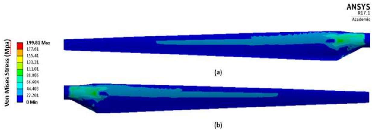
300 Figure 13: Contour plots showing the Von Mises (equivalent) stress from the FEA model of the full-scale wind turbine blade under the defined loading
