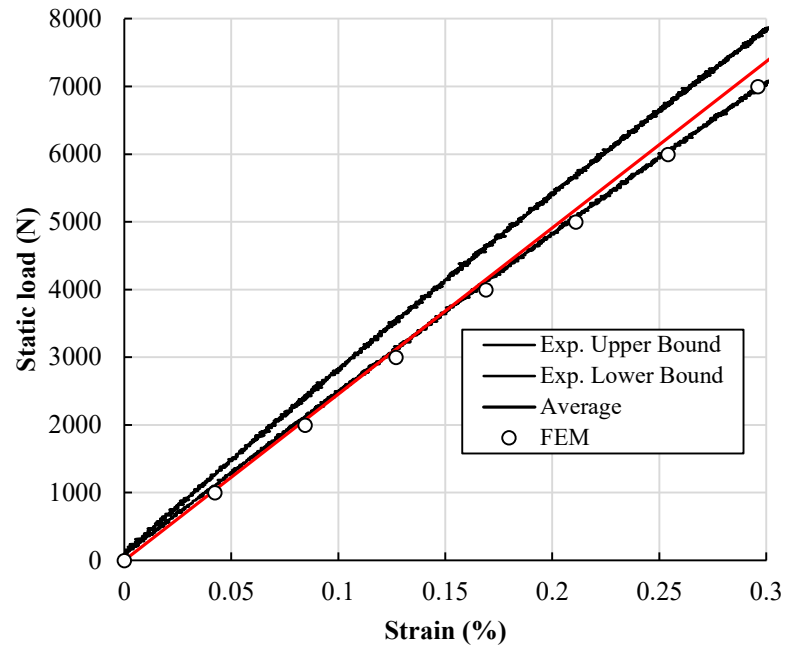
Figure 2: Experimental static testing of glass-fibre reinforced specimens, where (a) is the tests being performed and (b) is a comparison of the experimental static testing results with the results from the FEA model
