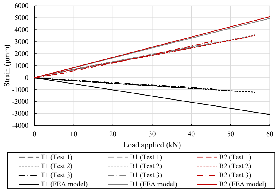
235 Figure 8: Strain recorded by the 3 linear strain gauges at the centre of the demonstrator during each test
