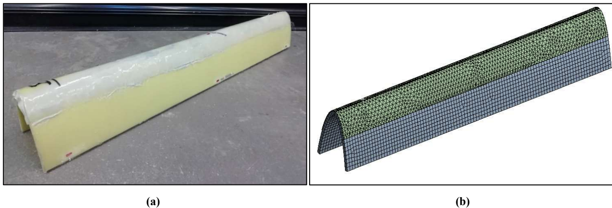
Figure 6: Leading edge demonstrator used for the validation study, showing (a) the physical model used for the experimental trials and (b) the meshed geometry used in the numerical FEA model
