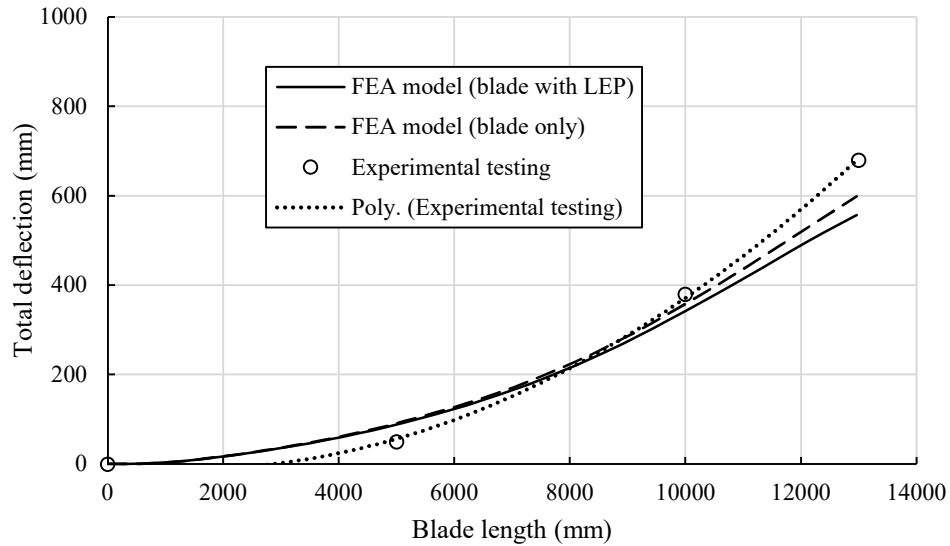
285 Figure 12: Comparison of the deflections from the FEA model of the full-scale wind turbine blade under the defined loading along the length of the blade with and without the LEP bonded and the experimental results (Fagan et al., 2017)
