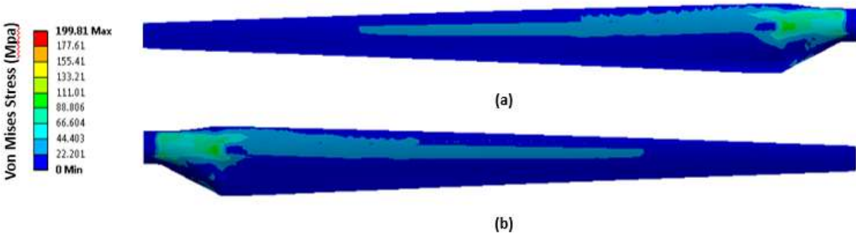
300 Figure 13: Contour plots showing the Von Mises (equivalent) stress from the FEA model of the full-scale wind turbine blade under the defined loading
