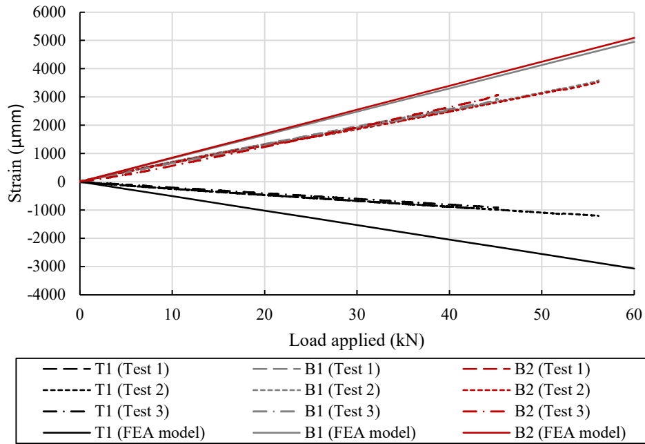
235 Figure 8: Strain recorded by the 3 linear strain gauges at the centre of the demonstrator during each test
