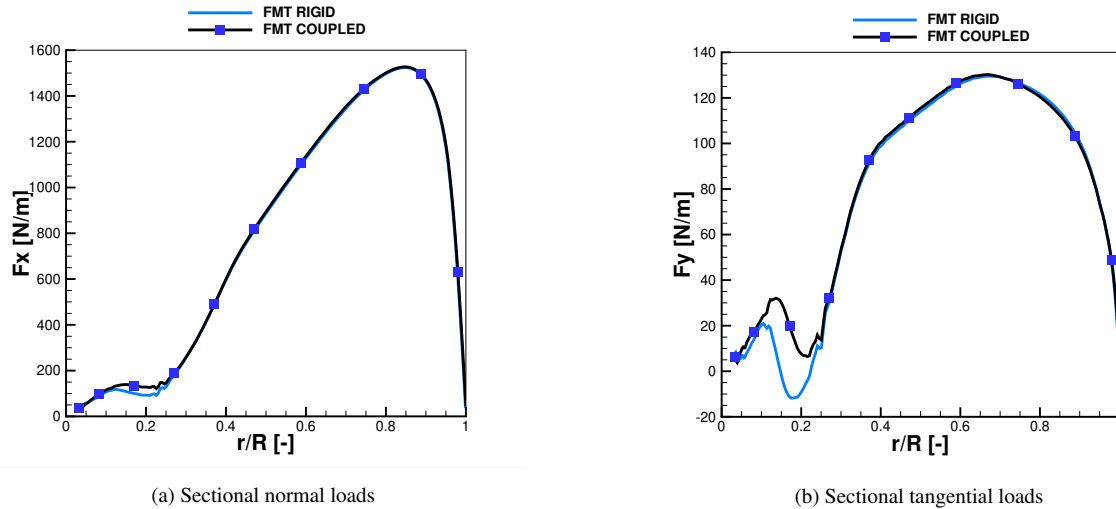
Figure 20. Sectional loads in FMT: comparison between rigid and coupled calculated with CFD.
