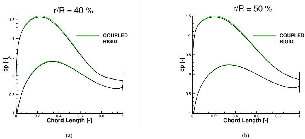
Figure 13. Pressure distributions for FMU rigid and coupled in comparison calculated with CFD at 6.1 m/s .
