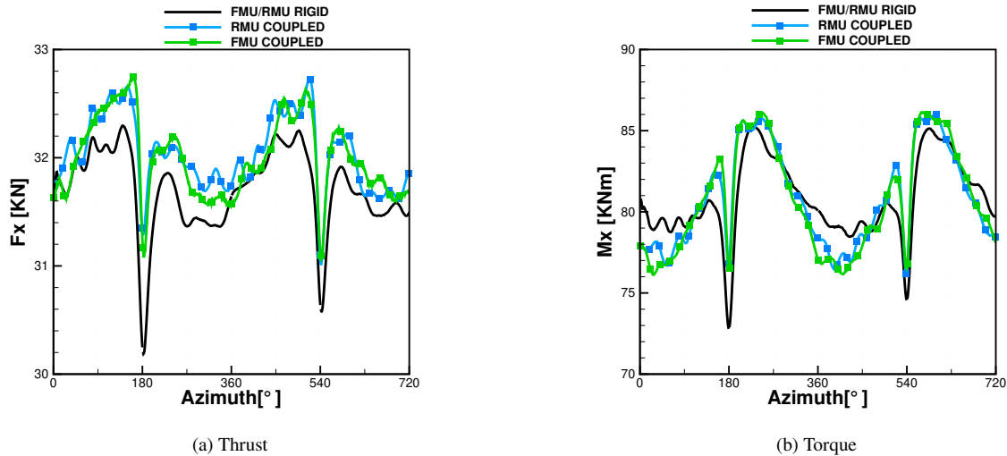
Figure 11. Thrust and torque calculated with CFD at 6.1 m/s in comparison RMU vs FMU, both rigid and coupled
