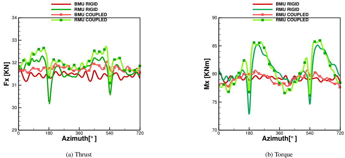
Figure 7. Thrust and torque calculated with CFD at 6.1 m/s in comparison BMU vs RMU, both rigid and coupled
