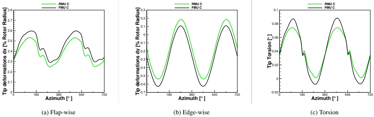
Figure 10. Tip deformations calculated with CFD at 6.1 m/s in comparison RMU vs FMU
