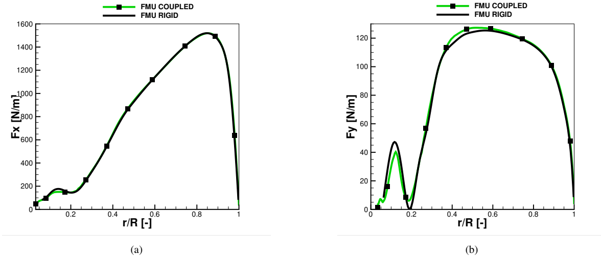
Figure 12. Sectional loads comparison in FMU both rigid and coupled calculated with CFD at 6.1 m/s .
