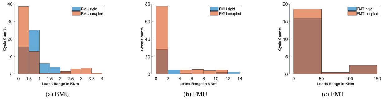
Figure 22. Comparison of number of cycle counts to load ranges using M_x from CFD as input
