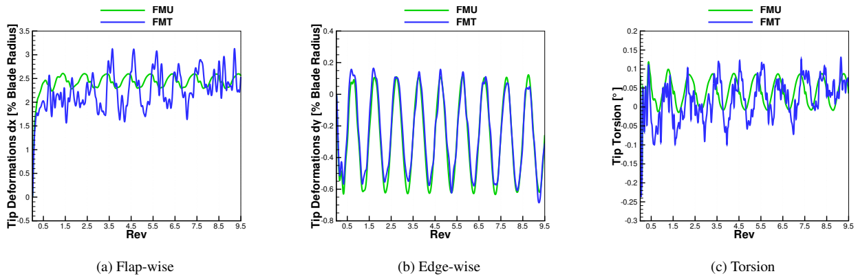
Figure 16. Tip deformations in comparison FMU vs FMT calculated with CFD.
