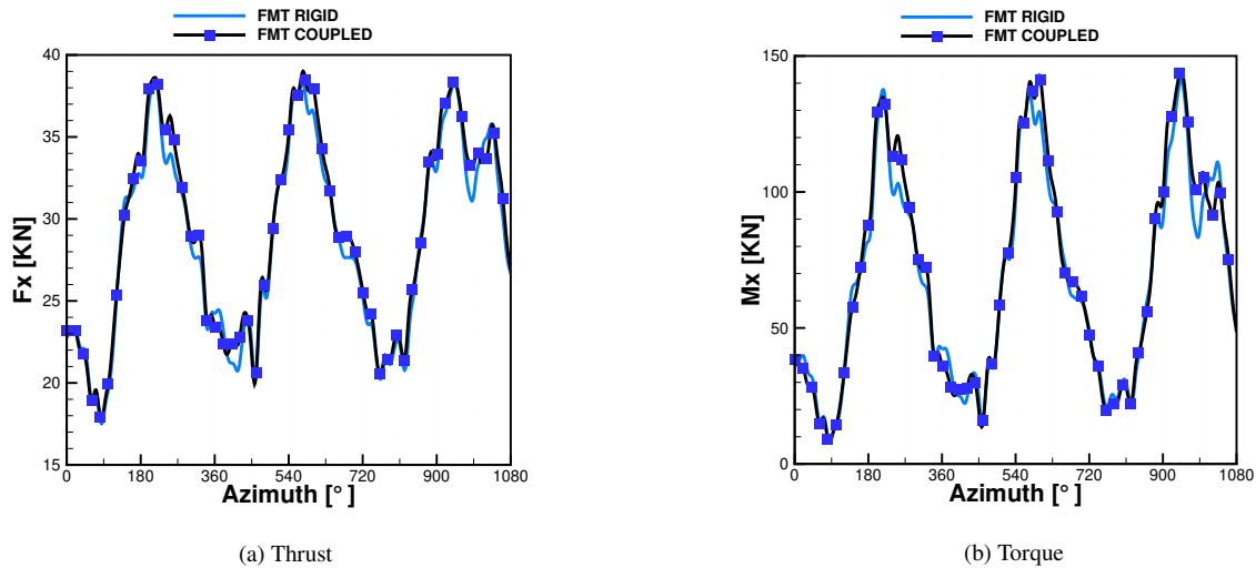
Figure 19. Global loads in FMT: comparison between rigid and coupled calculated with CFD.
