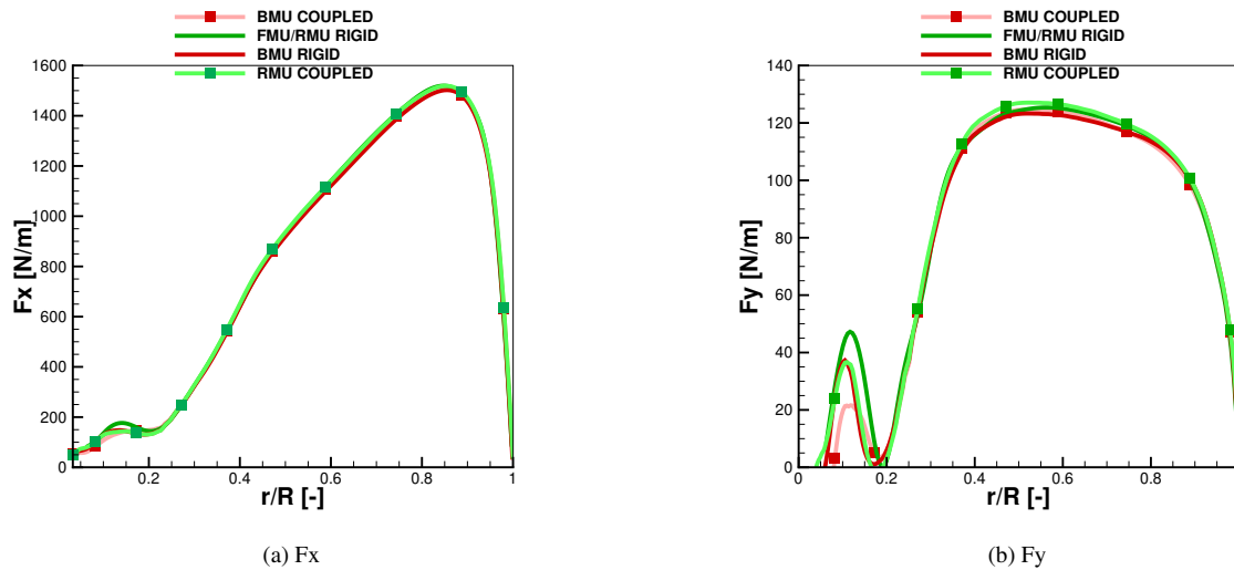
Figure 8. Normal and tangential time averaged sectional loads calculated with CFD at 6.1 \text{ m/s} in comparison BMU vs RMU, both rigid and coupled
