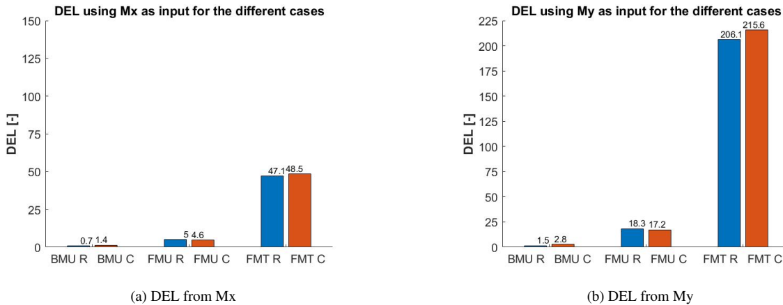
Figure 21. DEL calculation based on CFD for the different cases using in (a) M_x and in (b) M_y ; R and C stays for "rigid" and "coupled"
