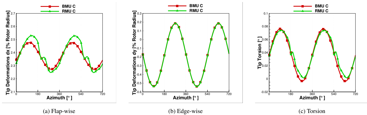
Figure 6. Tip deformations calculated with CFD at 6.1 \text{ m/s} in comparison: BMU coupled (C) vs RMU coupled (C). Out-of-plane deformation in (a), in-plane deformation in (b) and torsion in (c).
