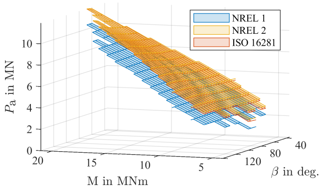
Figure 10. Equivalent loads P_a for a fixed pitch angle of \theta = 10^\circ at operating points from the aeroelastic simulations.
