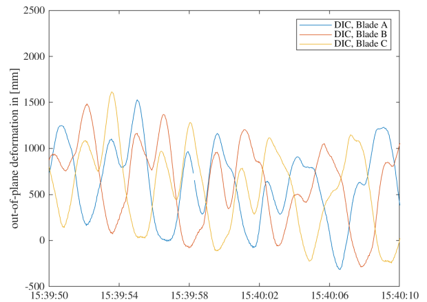
Figure 15. OoP DIC signal of all blades - Zoom
