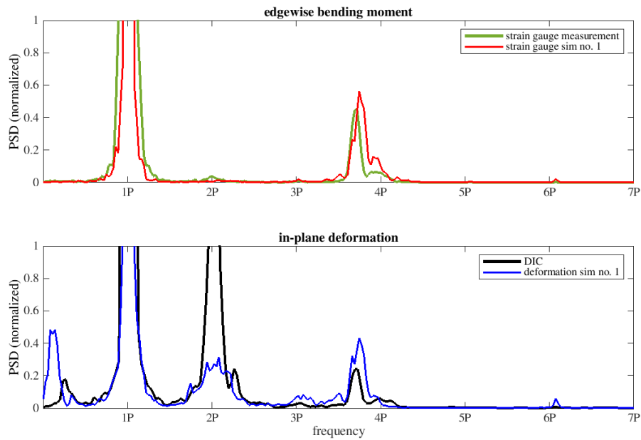
Figure 30. Comparison of PSD extracted with the Welch’s method for edgewise/IP signals of Blade B
