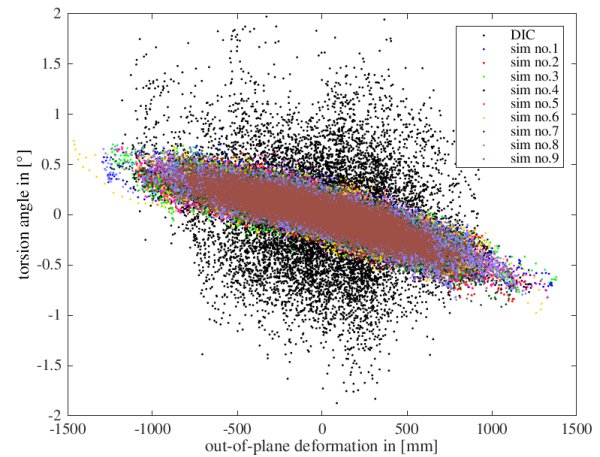
Figure 28. Coupling of rotor blade torsion and OoP deformation
