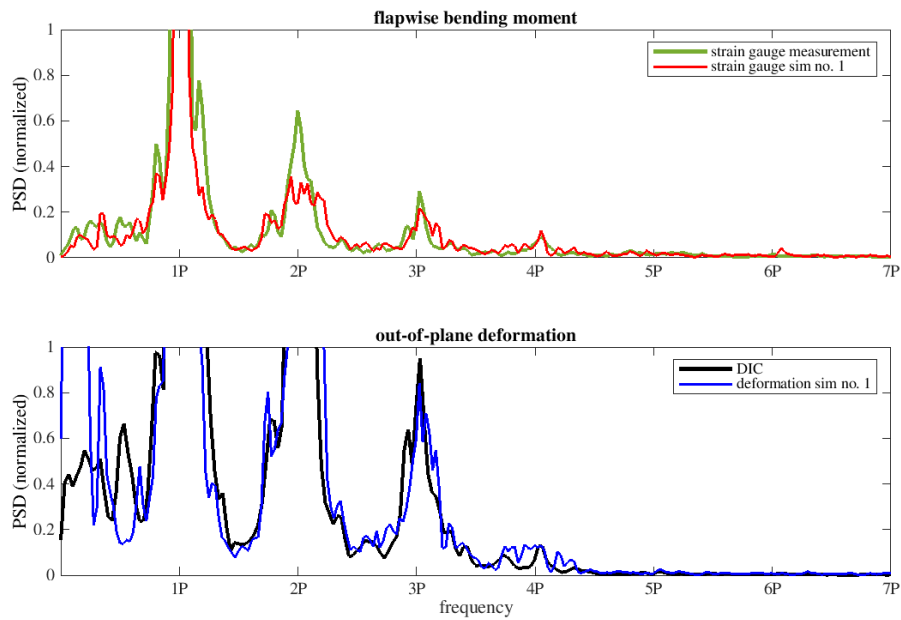
Figure 29. Comparison of PSD extracted with the Welch’s method for flapwise/OoP signals of Blade B
