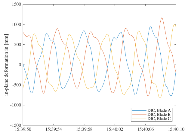
Figure 17. IP DIC signal of all blades - Zoom
