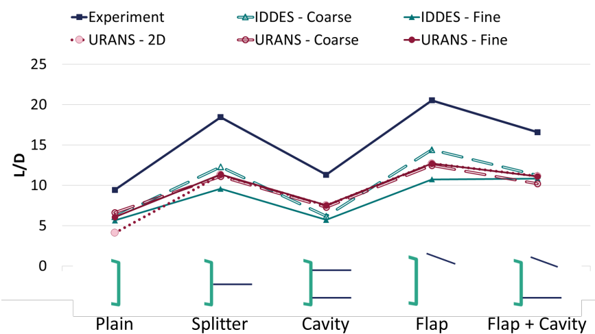
170 Figure 5: Lift to Drag ratio for the Plain airfoil and the airfoil with different TE devices. Comparison between Experiments, IDDES and URANS simulations.
