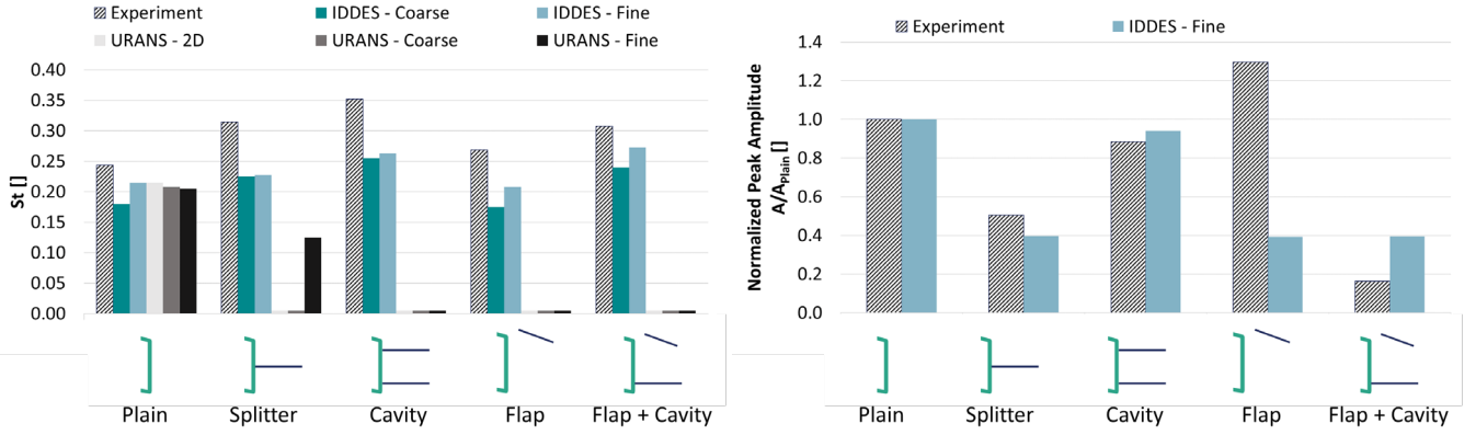
210 Figure 7: Left: Strouhal number ( St = fh_{TE}/V_{\infty} ) values for the Plain airfoil and the airfoil with different TE devices. Comparison between Experiments, IDDES and URANS simulations. Right: Normalized peak amplitude of the frequency spectrum Comparison between Experiments and Fine IDDES simulations.
