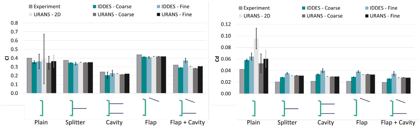
165 Figure 4: Lift (left) and drag coefficient (right) values for the Plain airfoil and the airfoil with different TE devices. Comparison between Experiments, IDDES and URANS simulations. Error bars in the numerical predictions are equal to the standard deviation of the force coefficient.
