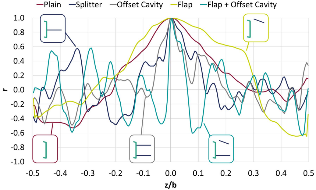
Figure 15. Pearson correlation coefficient of the lift coefficient ( C_l ) time-series with respect with the midsection (placed at z/b=0 ) for the various configurations. High positive values indicate strong positive correlation and highly negative values suggest a strong negative correlation.
