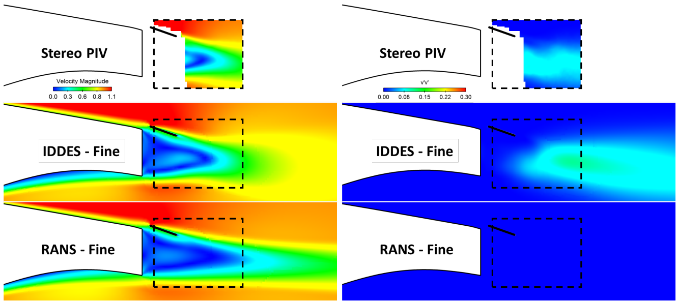
260 Figure 11: Flap case. Normalized velocity magnitude contours, V/V_\infty , (left) and \overline{v'v'}/V_\infty^2 normal Reynolds stress contours (right). Comparison between Stereo PIV, RANS and IDDES results. The Fine mesh (25M cells) was used in the calculations.
