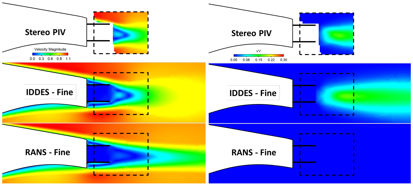
255 Figure 10: Offset Cavity case. Normalized velocity magnitude contours, V/V_\infty , (left) and \overline{v'v'}/V_\infty^2 normal Reynolds stress contours (right). Comparison between Stereo PIV, RANS and IDDES results. The Fine mesh (25M cells) was used in the calculations.
