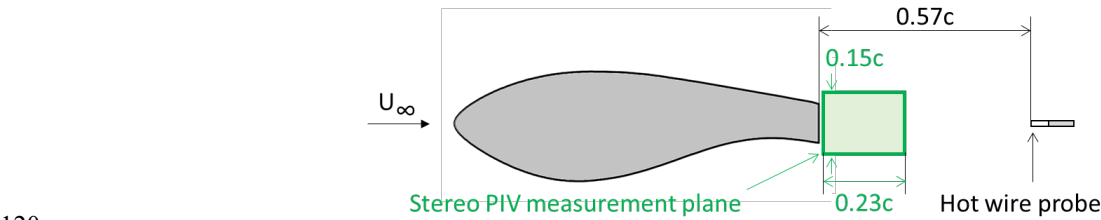
120 Figure 2: Schematic of the experimental set-up, showing the flatback airfoil under investigation, LI30-FB10, the location of the hot wire probe in the wake and size of the Stereo PIV measurement plane.
