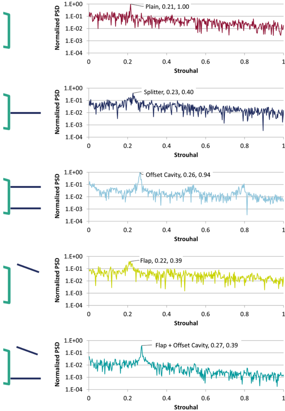
205 Figure 6: Normalized Power Spectral Density of the velocity time series for the Plain airfoil and all the TE device cases from Fine IDDES simulations. The vertical velocity is considered at (x, y) = (1.57c, 0) see also Figure 2. Strouhal number is defined based on the trailing edge thickness, St = fh_{TE}/V_\infty
