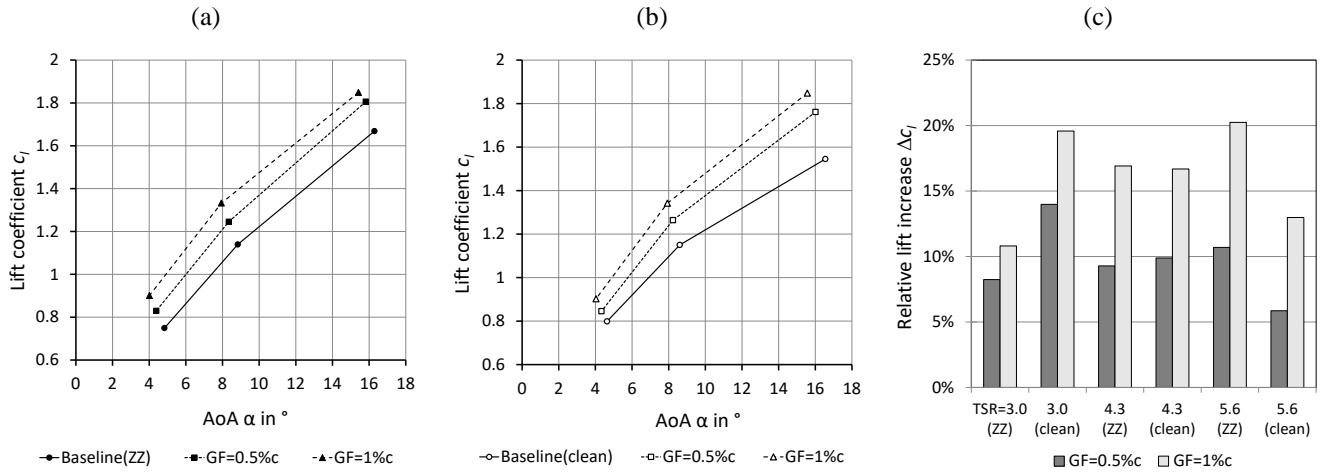
Figure 11. Lift coefficients over angles-of-attack at r = 0.45R and \varphi = 270^\circ . (a) Tripped case. (b) Clean case. (c) Relative lift increase of Gurney flap configurations in relation to the corresponding baseline.
