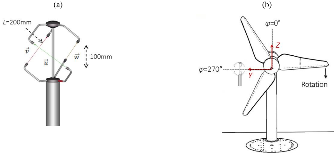
Figure 5. (a) Ultrasonic Anemometer, reproduced and modified from Thies CLIMA. (b) Definition of the azimuthal blade positions looking downstream.
