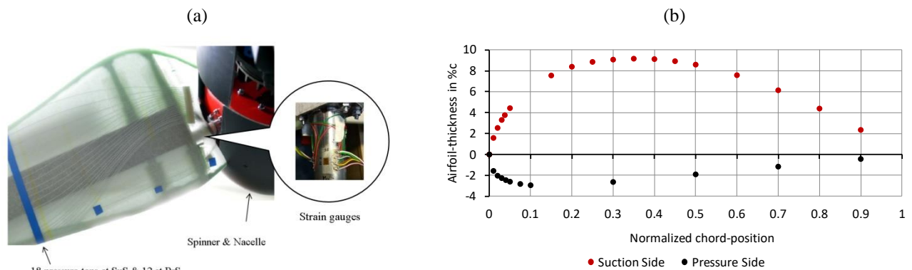
Figure 6. (a) BeRT blade and pressure taps, reproduced and modified from Fischer (2015). (b) Chord-wise position of pressure taps at r = 0.45R .
