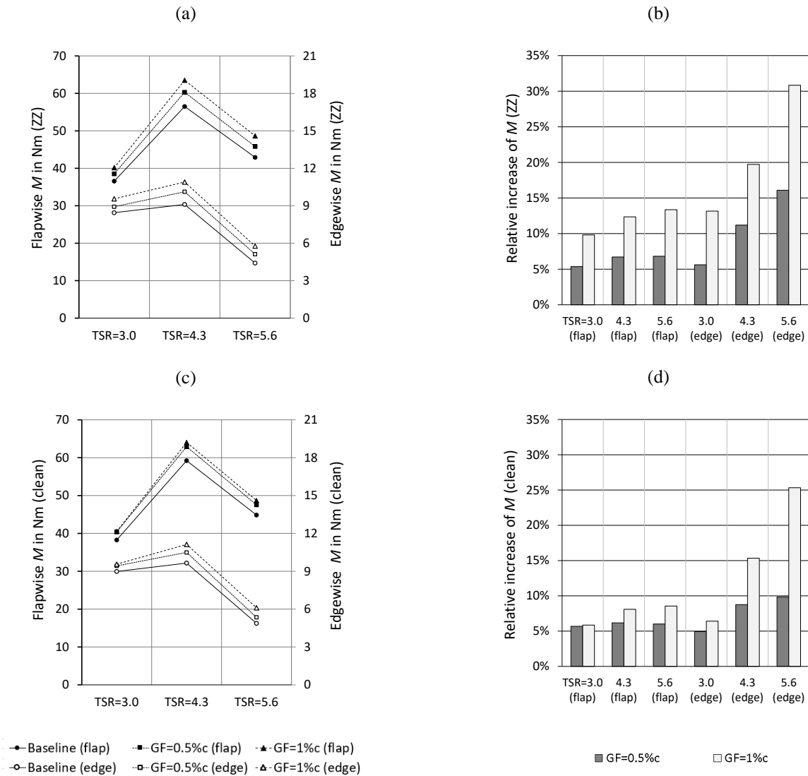
Figure 15. Flapwise (flap) and edgewise (edge) root bending moments. (a) Tripped case. (b) Relative increase to tripped baseline. (c) Clean case. (d) Relative increase to clean baseline.
