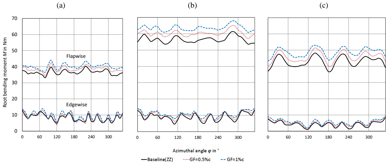
Figure 14. Flapwise and edgewise root bending moments in the tripped case. (a) TSR = 3.0 . (b) TSR = 4.3 . (c) TSR = 5.6 .
