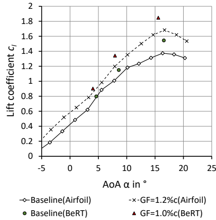
Figure 12. Lift coefficients of the Clark-Y airfoil including Gurney flap, reproduced and modified from Kheir-Aldeen (2014).
