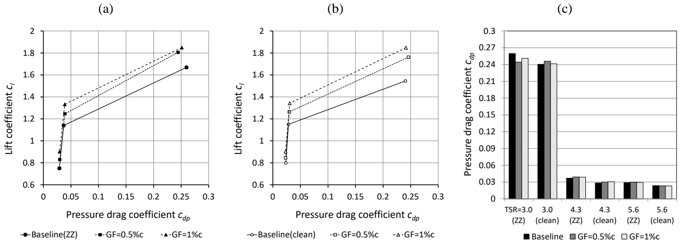
Figure 13. Lift over pressure drag coefficients at r = 0.45R and \phi = 270^\circ . (a) Tripped case. (b) Clean case. (c) Pressure drag coefficients in relation to the corresponding baseline.
