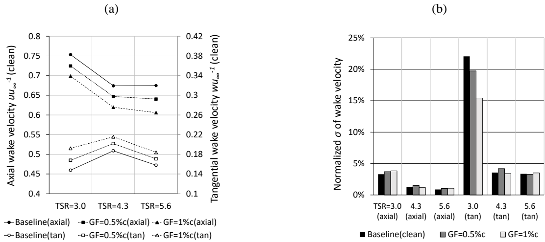
435 Figure A 1. Clean case at r = 0.56R and \phi = 270^\circ . (a) Axial and tangential (tan) wake velocity normalized by the inflow velocity. (b) Standard deviation of the wake velocity normalized by the average wake velocity.
