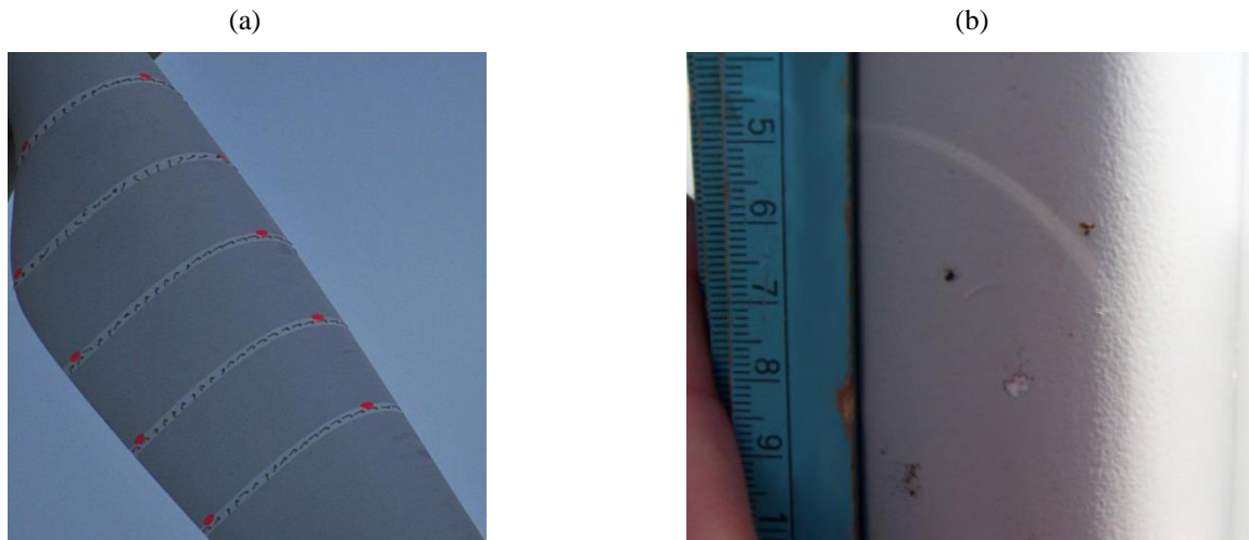
35 Figure 1. Rotor blades of utility scale wind turbines. (a) Flow indicators to detect early separation in the inner blade region, reproduced from Pechlivanoglou et al. (2013). (b) Leading edge roughness, reproduced from Pechlivanoglou et al. (2010).
