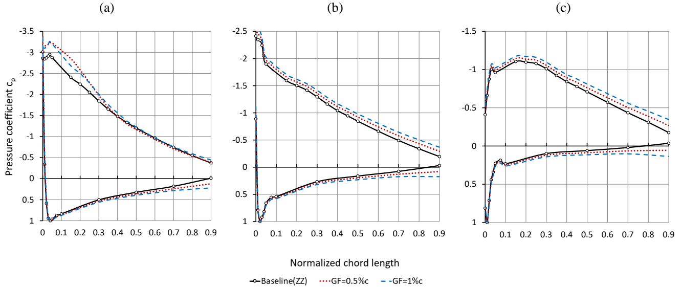
Figure 10. Pressure coefficients in the tripped case with respect to different scales at r = 0.45R and \varphi = 270^\circ . (a) TSR = 3.0 . (b) TSR = 4.3 . (c) TSR = 5.6 .
