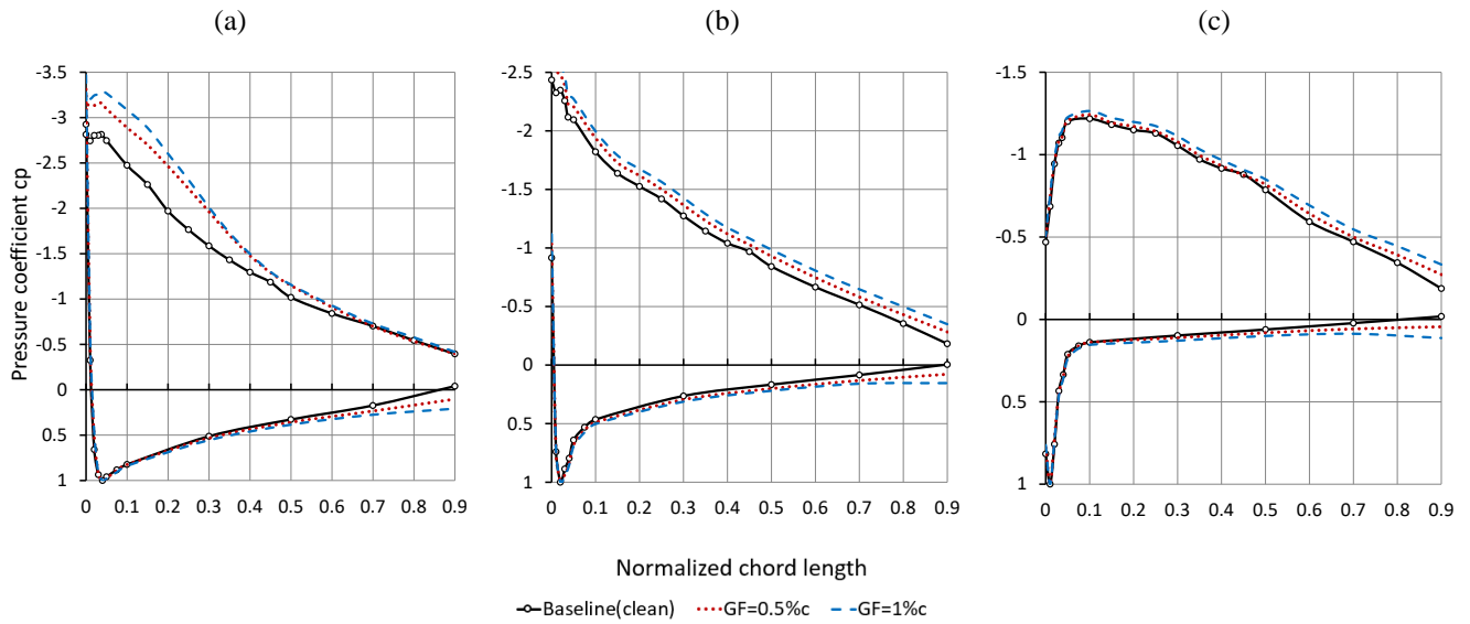
440 Figure A 3. Pressure coefficients in the clean case with respect to different scales at r = 0.45R and \varphi = 270^\circ . (a) TSR = 3.0 . (b) TSR = 4.3 . (c) TSR = 5.6 .
