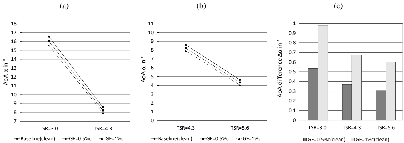
Figure A 2. Angles-of-attack in the clean case at r = 0.56R and \phi = 270^\circ . (a) Stall and rated conditions (b) Rated and feather conditions (c) AoA difference between Gurney flap configuration and the baseline.
