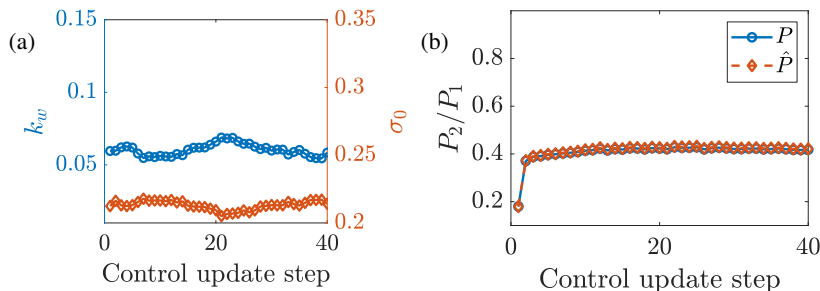
Figure F3. Two wind turbine model uniform inflow LES (a) k_w and \sigma_0 for the upwind turbine and (b) \hat{P} and P for the downwind turbine.
