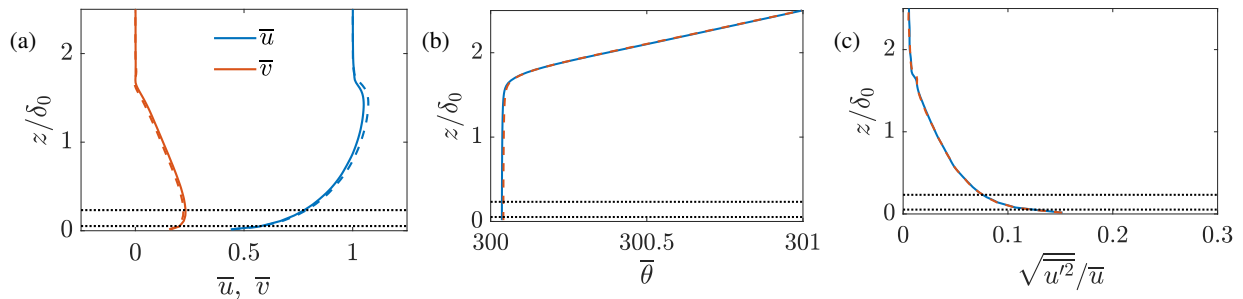
Figure 4. Horizontally averaged concurrent precursor conventionally neutral ABL LES (a) velocity, (b) potential temperature in Kelvins, and (c) turbulence intensity. Horizontally averaged profiles from two different time instances are shown with solid (early) and dashed (late) lines, qualitatively demonstrating that the flow is statistically quasi-stationary (see further discussion by Howland et al., 2020a). Dashed-dotted lines show the extents of the turbine rotor area.
