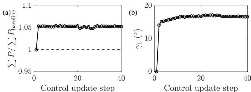
Figure F2. Two wind turbine model uniform inflow LES (a) power production. (b) The yaw misalignment angle \gamma for the upwind turbine. The downwind turbine remains yaw aligned during the simulation.
