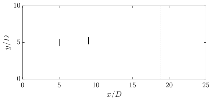
Figure F1. Uniform inflow LES simulation actuator disk model layout. The fringe region is represented by the dashed black line and the wind turbines are shown as solid black lines.
