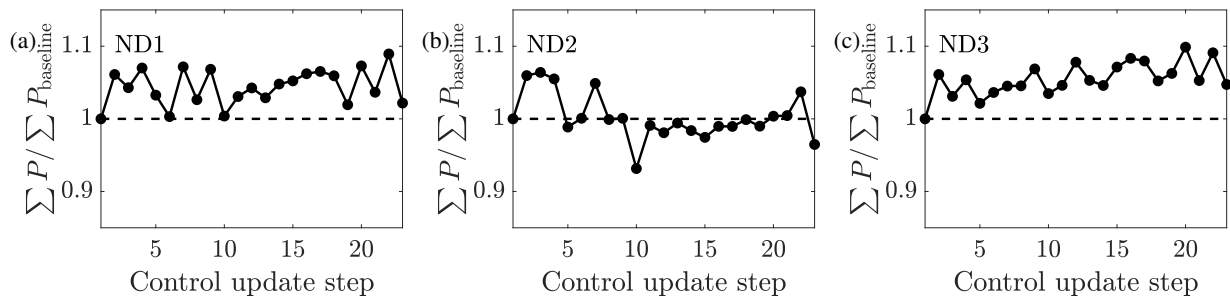
Figure 11. Time averaged wind farm power production as a function of the control update steps for (a) online control using the initial parameters to initialize the next state (ND1), (b) online control using the previous optimal parameters to initialize the next state (ND2), and (c) and the static state estimation control (ND3). The wind farm power is normalized by the power production of the aligned wind farm case.
