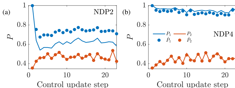
Figure 19. Time averaged power production for the first and second wind turbines in the wind farm as a function of the control update steps for online control using the initial parameters to initialize the next state and (a) \hat{P}_p = 2 (NDP2) and (b) \hat{P}_p = 4 (NDP4). The LES power production is given by P and the wake model state estimation is given by \hat{P} .
