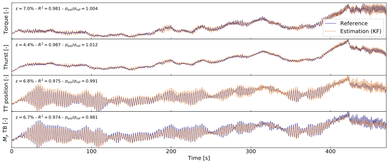
Figure 6. Comparison of signals simulated by OpenFAST (reference) compared with the ones estimated with the Kalman filter model. From top to bottom, dimensionless time series of: aerodynamic torque, aerodynamic thrust, tower-top displacement, and fore-aft tower-bottom moment.
