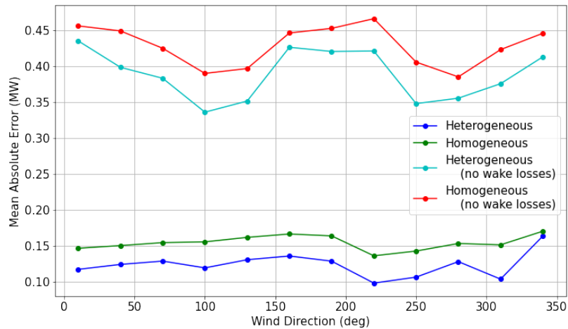
Figure 15. Average absolute error of individual turbine power output predictions calculated using the homogeneous and heterogeneous FLORIS models, with and without wake losses.
