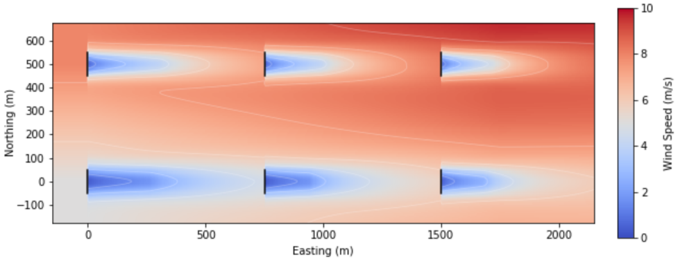
(a) Horizontal plane of the FLORIS simulation, taken at the turbine hub height (90m).
