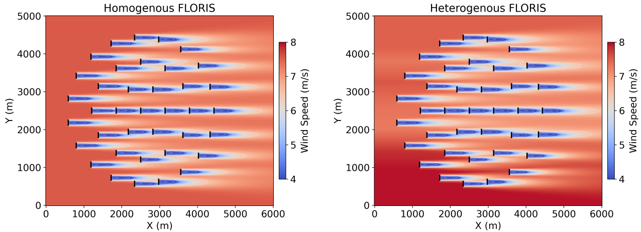
Figure 12. Horizontal cut-planes of the FLORIS simulations with wind direction at 270 degrees. Wake losses were calculated using the homogenous FLORIS model (left) and heterogenous FLORIS model (right). Turbine rotors are indicated by black lines.
