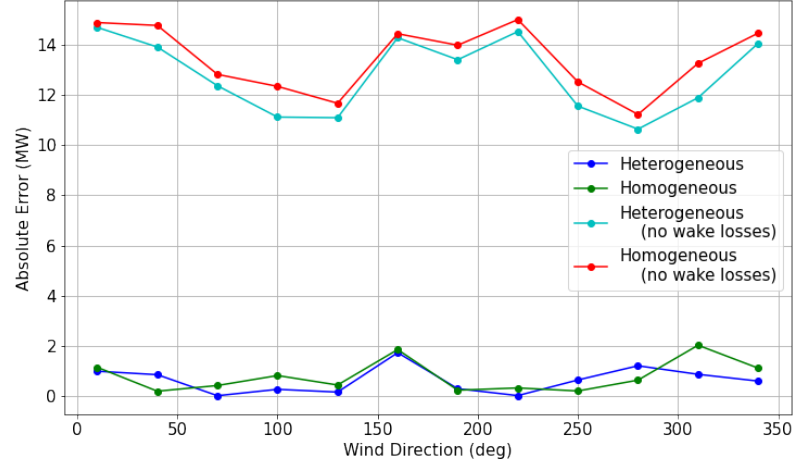
Figure 14. Absolute error in total farm power output calculated using the homogeneous and heterogeneous FLORIS models, with and without wake losses.
