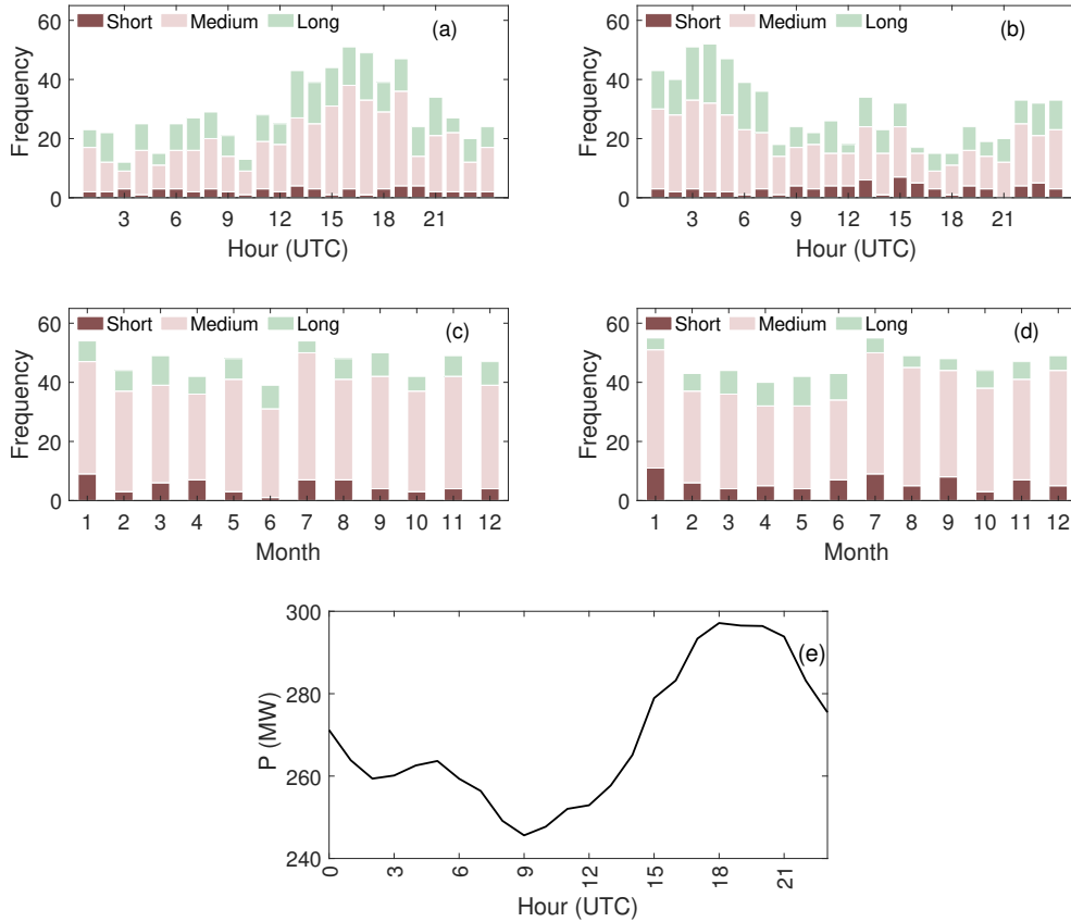
Figure 8. Diurnal and monthly frequency ramps events for short, medium and long duration: (a) diurnal ramp-up events; (b) diurnal ramp-down events; (c) monthly ramp-up events; (d) monthly ramp-down events; (e) diurnal variation of wind power.
