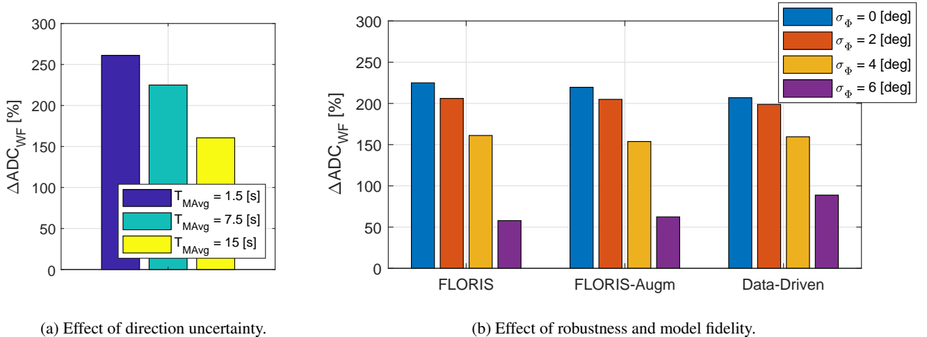
Figure 17. Change in wind farm yaw ADC with respect to the greedy case. Left: non-robust LUT for the baseline FLORIS model and varying T_{\text{MAvg}} . Right: LUTs for the three models and increasing robustness, for a wind direction signal filtered with T_{\text{MAvg}} = 7.5 s.
