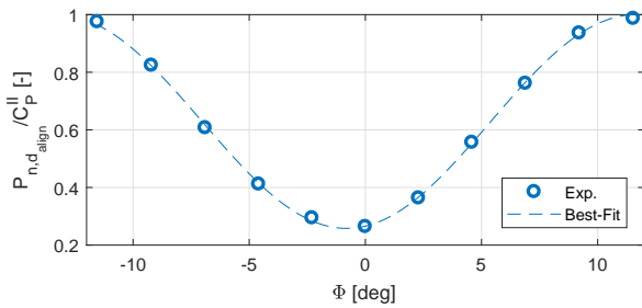
(a) Normalized power of WT2—the downstream turbine in a two-turbine cluster vs. \Phi for \gamma_1 = \gamma_2 = 0 \gamma_u = \gamma_d = 0 .
