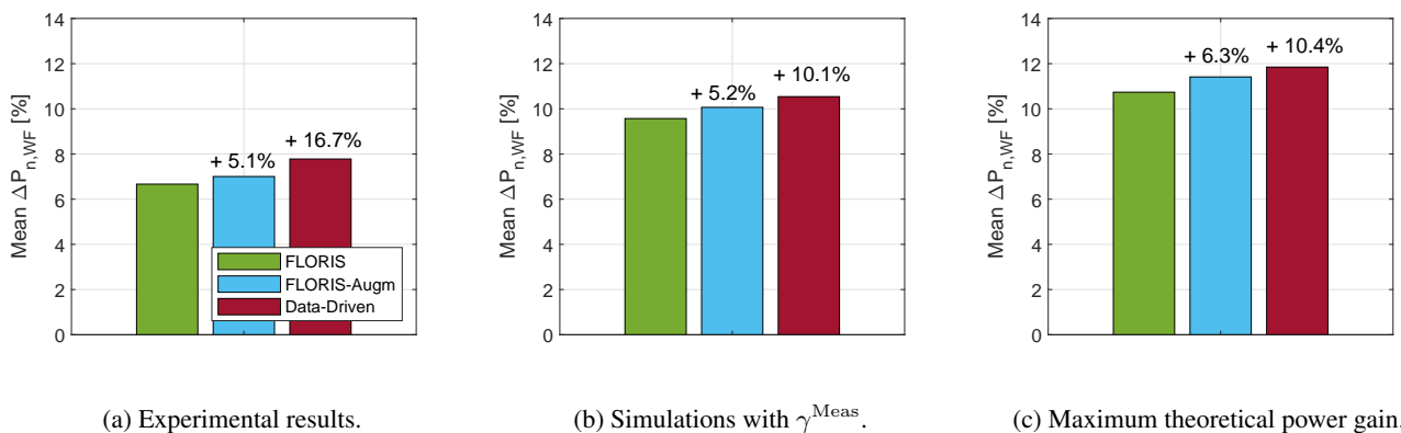
Figure 14. Normalized wind farm power gains for the three models of different fidelity.
