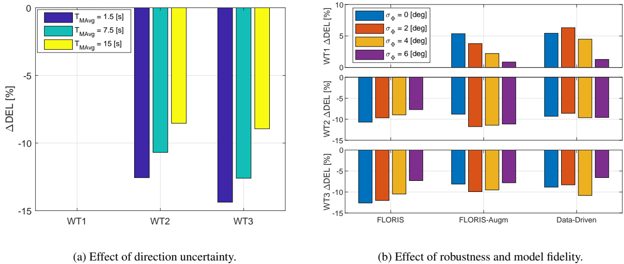
Figure 18. Change in combined rotating shaft DELs with respect to the greedy case. Left: non-robust LUT for the baseline FLORIS model and varying T_{\text{MAvg}} . Right: LUTs for the three models and increasing robustness, for a wind direction signal filtered with T_{\text{MAvg}} = 7.5 s.
