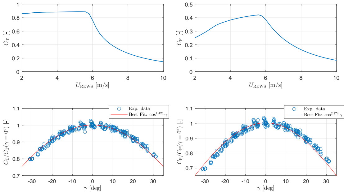
Figure 2. Top: C_T (left) and C_P (right) vs. rotor-equivalent wind speed U_{REWS} . Bottom: C_T (left) and C_P (right) vs. misalignment angle \gamma .
