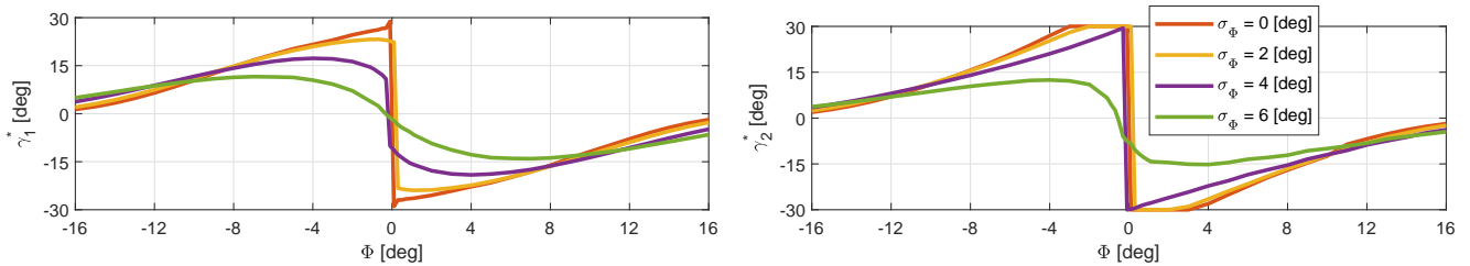
(a) FLORIS LUTs for different uncertainty levels. \gamma_1^* for WT1 on the left, \gamma_2^* for WT2 on the right.
