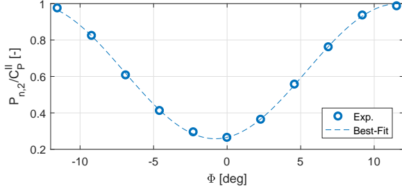
(a) Normalized power of WT2 vs. \Phi for \gamma_1 = \gamma_2 = 0 .
