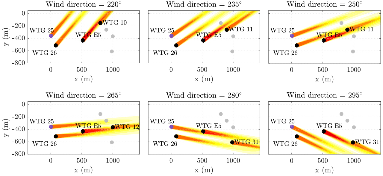
Figure 3. Predicted flow fields for various wind directions in baseline operation. To maximize the benefits of wake steering, only three turbines are considered at a time, depending on the ambient wind direction. The considered turbines are WTG 26, WTG E5, and one of the downstream turbines (operated without yaw misalignment). The schedule of which turbines are considered is listed in Table 2. Note that this figure is shown for explanatory purposes and therefore the simulation setup is not described in detail.
