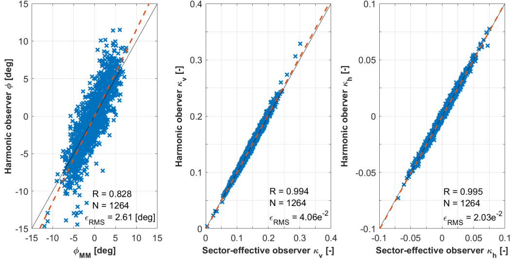
Figure 8. Correlation of 1-min averages between estimated parameters ( y axis) and their reference quantities ( x axis) for V \geq 8 \text{ ms}^{-1} . From left to right: yaw misalignment angle, vertical linear shear, horizontal linear shear. Red dashed line: linear best fit; black dashed line: ideal match; R : Pearson's correlation coefficient; N : number of data points; \epsilon_{\text{RMS}} : root mean square error.
