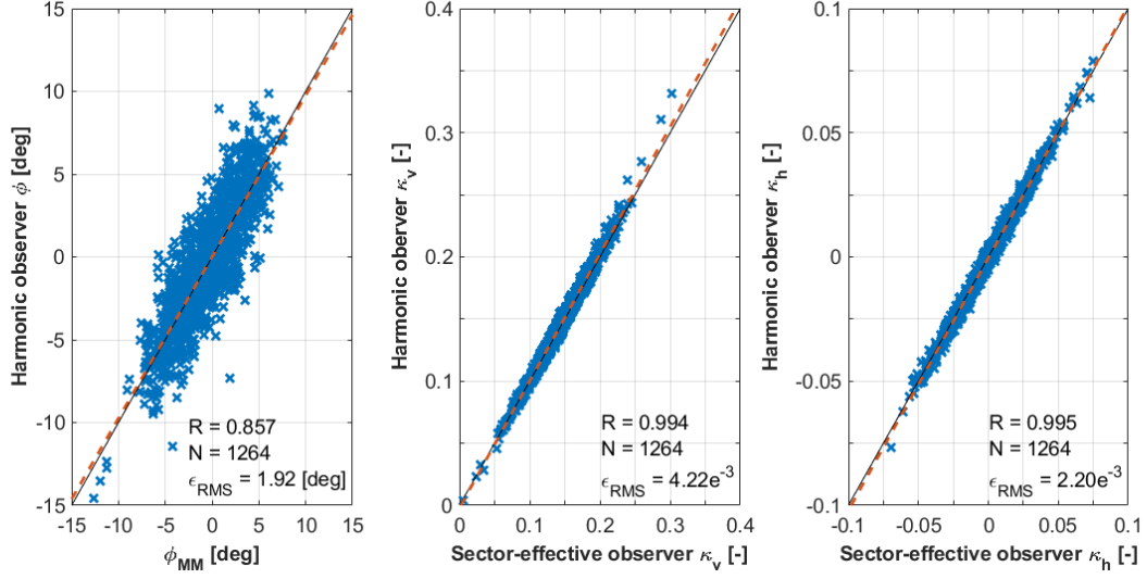
Figure 7. Correlation of 10-min averages between estimated parameters ( y axis) and their reference quantities ( x axis) for V \geq 8 \text{ ms}^{-1} . From left to right: yaw misalignment angle, vertical linear shear, horizontal linear shear. Red dashed line: linear best fit; black dashed line: ideal match; R : Pearson's correlation coefficient; N : number of data points; \epsilon_{\text{RMS}} : root mean square error.
