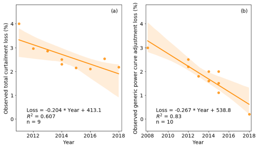
250 Figure 8: Trend in observed energy-production loss: (a) total curtailment loss and (b) generic power curve adjustment loss. The annotations correspond to those in Fig. 3, where the orange solid line represents simple linear regression, the light orange cone illustrates the 95% confidence interval, R^2 is the coefficient of determination, and n is sample size.
