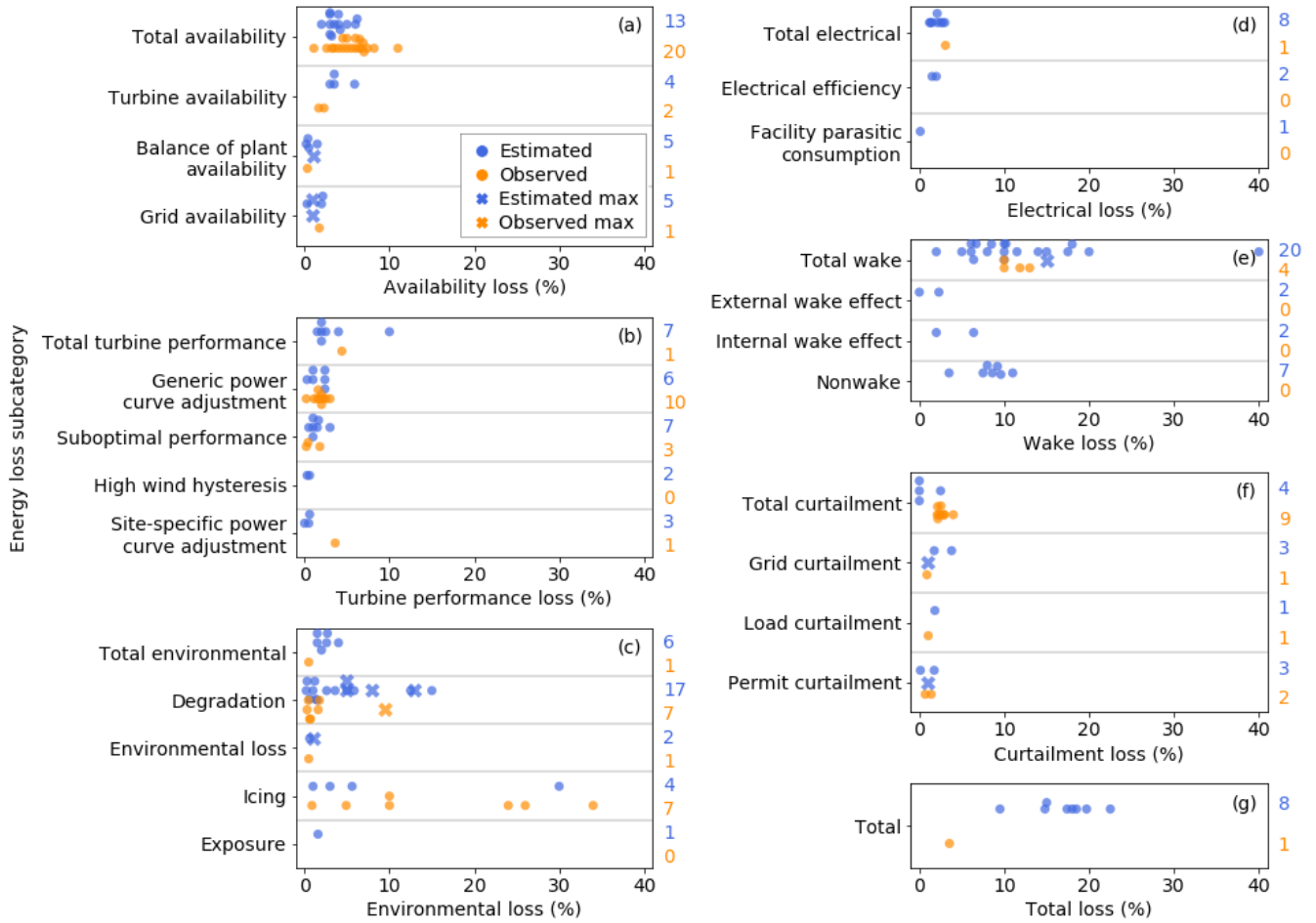
Figure 6: Ranges of energy-production losses in different categories and subcategories, according to the proposed framework of the IEC 61400-15 standard, except for nonwake in (e), which is an extra subcategory summarizing other nonwake categories. Each blue and orange dot, respectively, represent the mean estimated loss and mean observed loss documented in each independent study. The blue and orange crosses, respectively, indicate the maximum of estimated loss and the maximum of observed loss reported, where the minima are not reported, and thus the averages cannot be calculated. The losses are expressed as percentage of AEP. The column of numbers on the right denotes the estimated and observed sample sizes in blue and orange, respectively, in each subcategory, and such sample size represents all the instances in that subcategory that recorded either the mean or the maximum loss values. For clarity, the grey horizontal lines separate data from each subcategory. Table B3 catalogs the categorical and subcategorical losses plotted herein.
