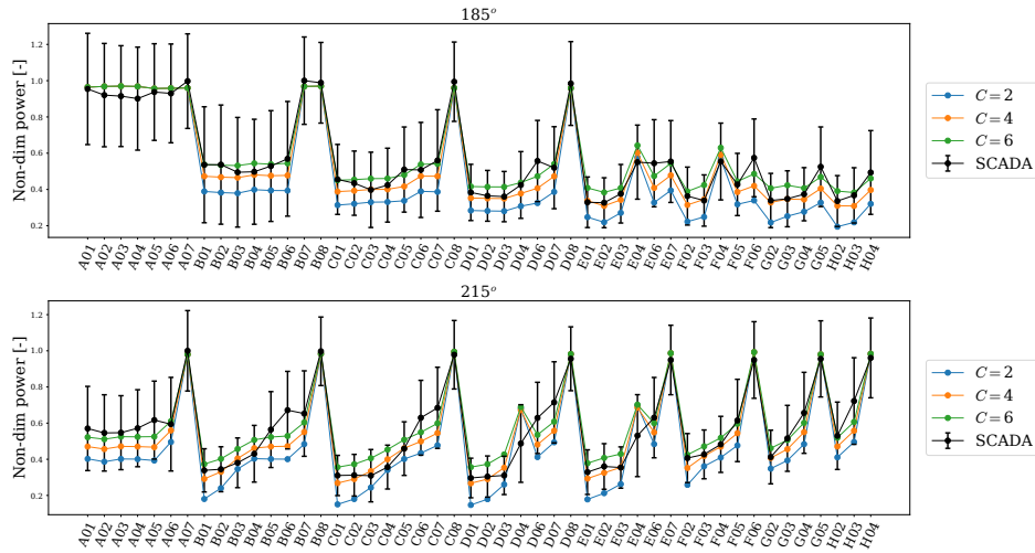
Figure A1. Comparison of turbine power versus SCADA data for the Lillgrund Wind Plant for cases at two different wind directions (185°, 215°). Different lines denote values of the constant C used to scale the viscous term in the solver.
