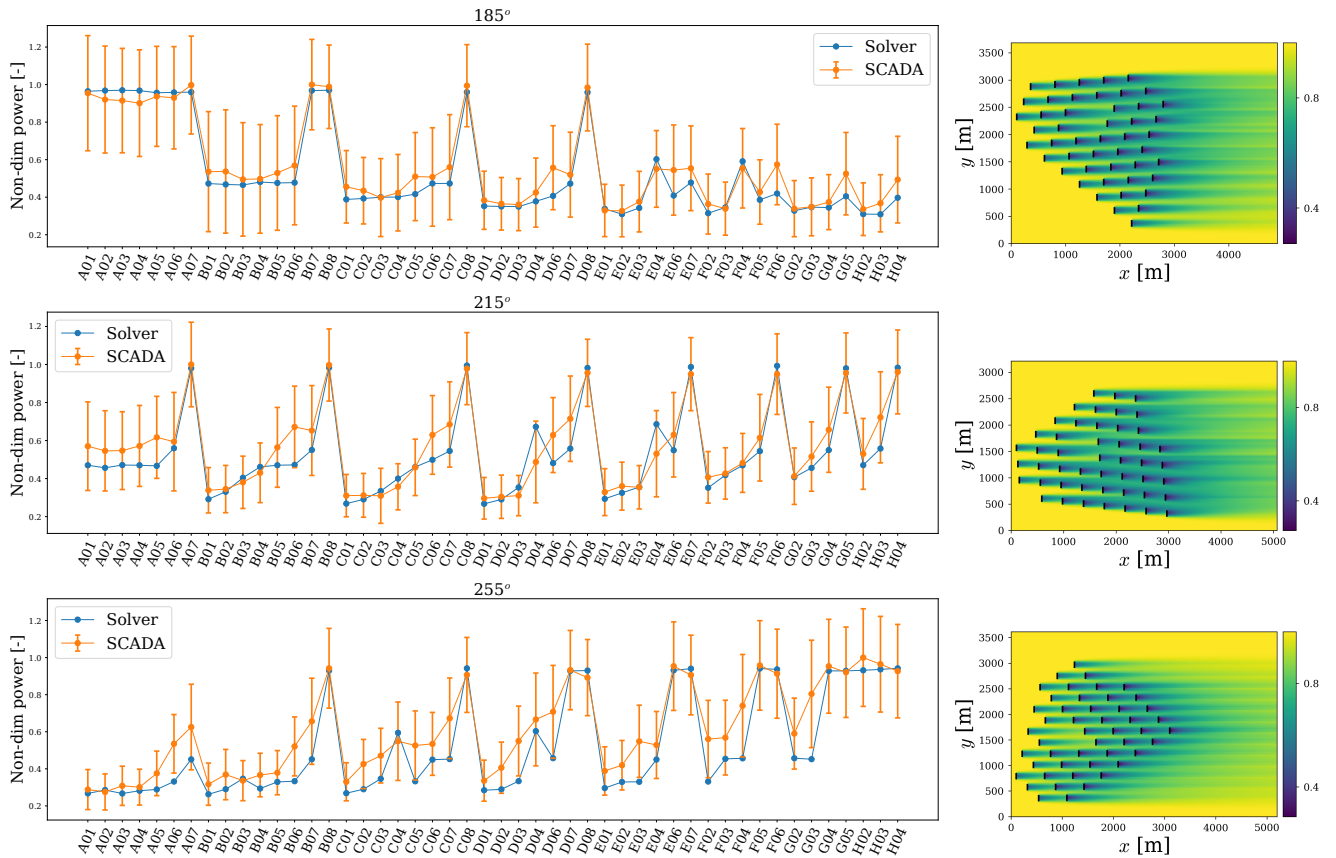
Figure 5. Comparison of turbine power versus SCADA data for the Lillgrund Wind Plant for cases at three different wind directions (185°, 215°, 255°). Streamwise velocity contours at hub height are shown for all cases with the wind plant aligned with the flow direction.
