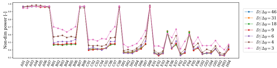
Figure C1. Comparison of turbine power for all turbines using different number of grid points across the turbine diameter for the Lillgrund wind plant for cases at wind direction of 185°.
