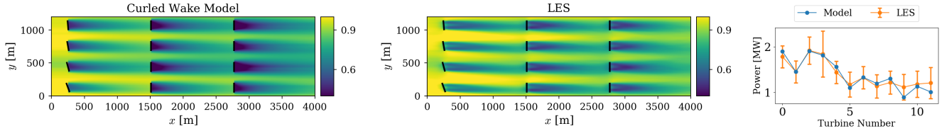
Figure 7. Velocity at hub height normalized by average speed at hub height from the model proposed and from LES and power output for each turbine from the model proposed compared to results from LES. Simulations of a 4-by-3 turbine array. The bars in the LES power denote one standard deviation of the power. Turbine numbering is from bottom to top and left to right.
