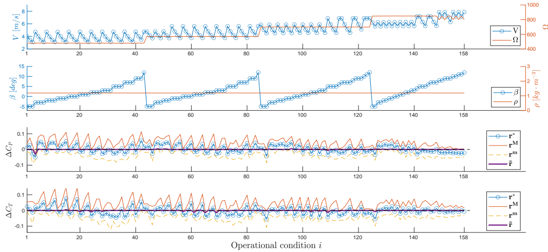
Figure 3. Top two plots: nominal model inputs V , \Omega , \beta , \rho . Bottom two plots: nominal, maximal, minimal and filtered residuals for the two outputs \Delta C_P and \Delta C_T . All quantities are plotted for each one of the 158 operating conditions in the measurement set.
