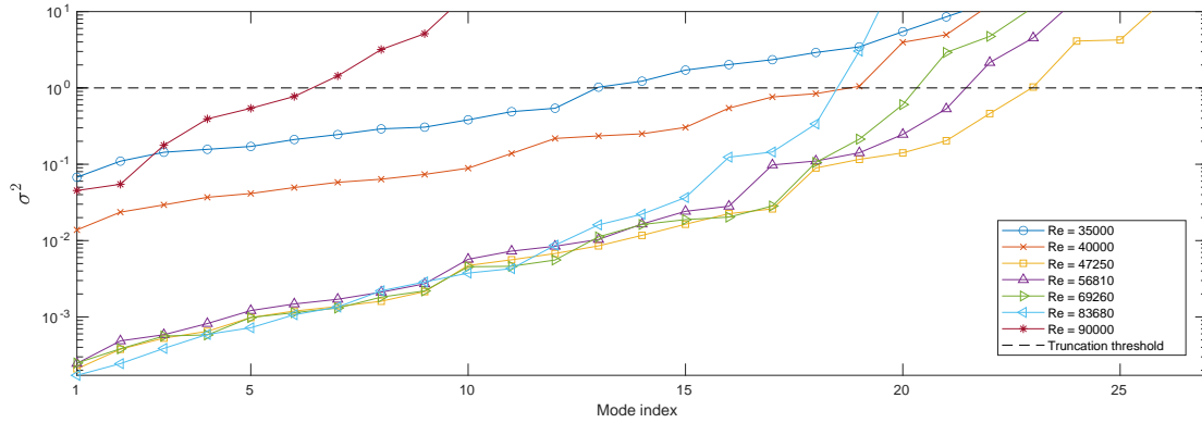
Figure 2. Variance of the lowest 25 modes modes for varying Reynolds.
