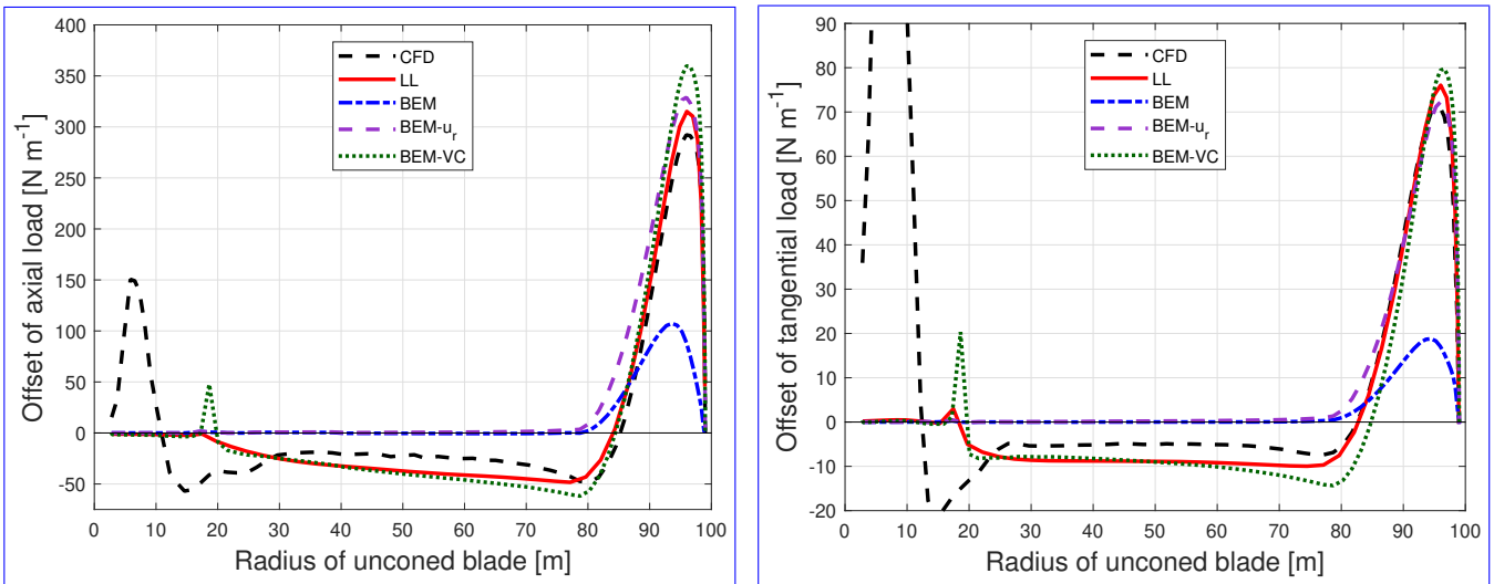
Figure B9. Comparison of the difference of the out-of-plane axial load (left) and in-plane tangential load (right) of the dihedral blade W-4 with 15° of cone downwind compared to the baseline blade with the same cone calculated from different aerodynamic models.
