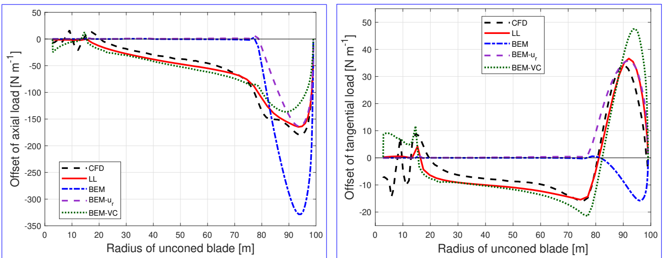
Figure B5. Comparison of the difference of the out-of-plane axial load (left) and in-plane tangential load (right) of the dihedral blade W-3 with 15° of cone upwind compared to the baseline blade with the same cone calculated from different aerodynamic models.
