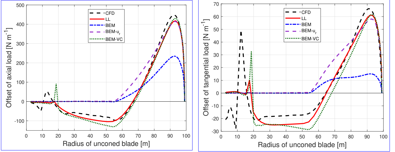
Figure 16. Comparison of the difference of the out-of-plane axial load (left) and in-plane tangential load (right) of the upwind dihedral blade W-1 with 15° of cone downwind compared to the baseline blade with the same cone calculated from CFD, lifting-line method (LL), BEM method, BEM with radial induction (BEM- u_r ) and the proposed BEM-VC method.
