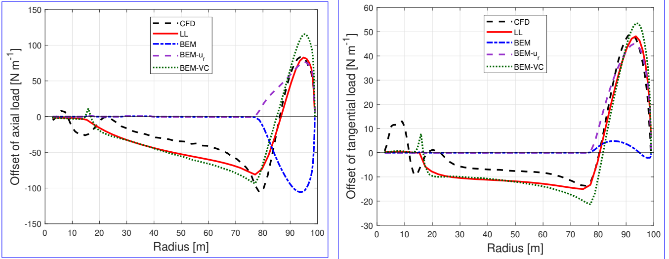
Figure B2. Comparison of the difference of the out-of-plane axial load (left) and in-plane tangential load (right) of the dihedral blade W-3 compared to the baseline blade calculated from different aerodynamic models.
