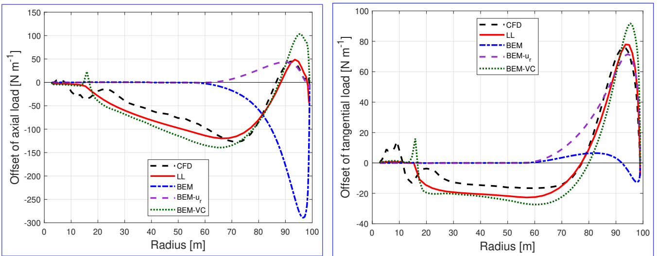
Figure B1. Comparison of the difference of the out-of-plane axial load (left) and in-plane tangential load (right) of the dihedral blade W-2 compared to the baseline blade calculated from CFD, lifting-line method (LL), BEM method, BEM with radial induction (BEM- u_r ) and the proposed BEM-VC method.
