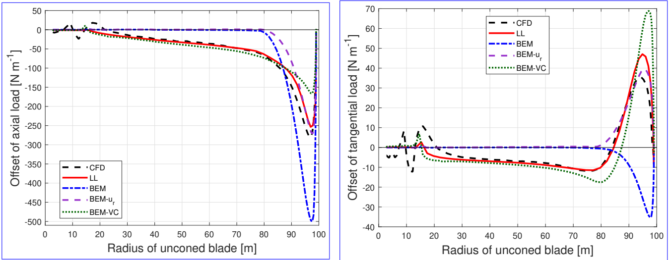
Figure B6. Comparison of the difference of the out-of-plane axial load (left) and in-plane tangential load (right) of the dihedral blade W-4 with 15° of cone upwind compared to the baseline blade with the same cone calculated from different aerodynamic models.
