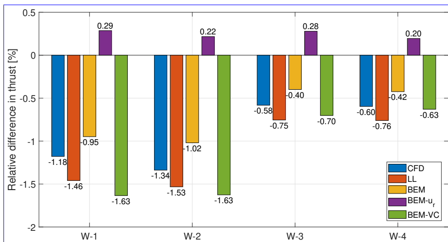
Figure 18. The relative difference of thrust the dihedral blades without cone compared to the baseline straight blade. The operational condition is with uniform wind speed of 8 \text{ m s}^{-1} , rotational speed 0.855 \text{ rad s}^{-1} and zero cone angle.
