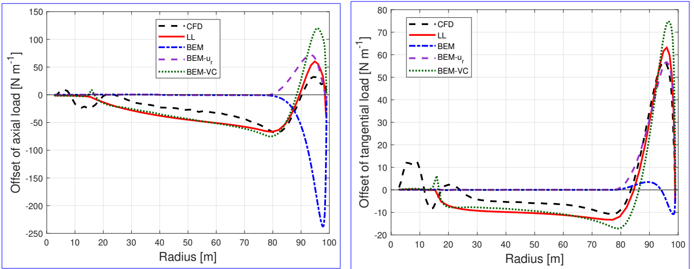
Figure B3. Comparison of the difference of the out-of-plane axial load (left) and in-plane tangential load (right) of the dihedral blade W-4 compared to the baseline blade calculated from different aerodynamic models.
