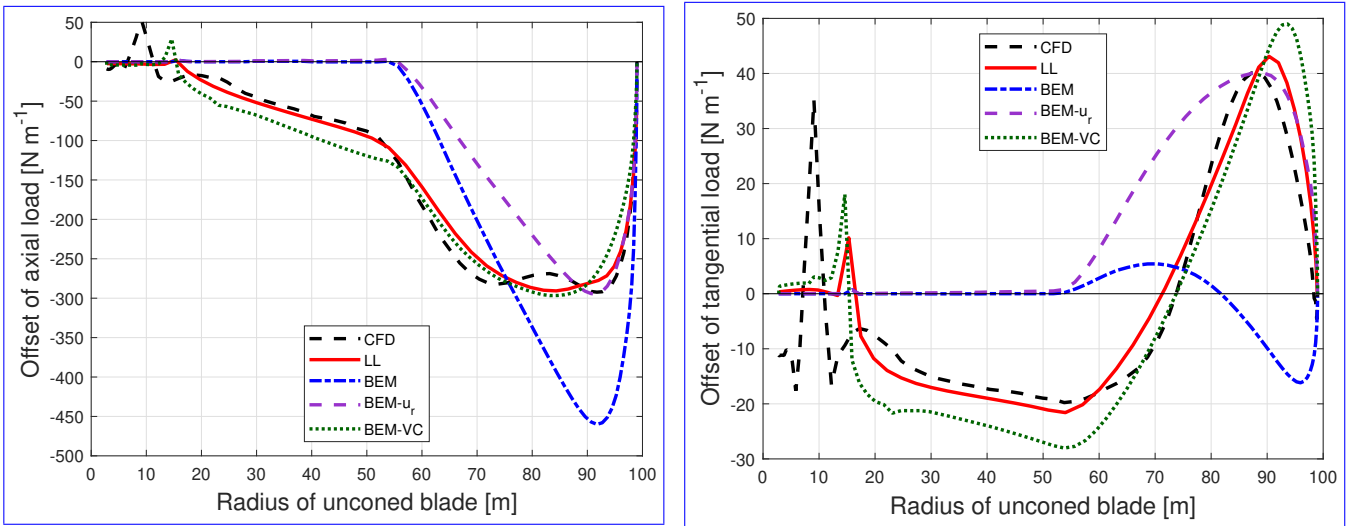
Figure 14. Comparison of the difference of the out-of-plane axial load (left) and in-plane tangential load (right) of the dihedral blade W-1 with 15^\circ of cone upwind compared to the baseline blade with the same cone calculated from CFD, lifting-line method (LL), BEM method, BEM with radial induction (BEM- u_r ) and the proposed BEM-VC method.
