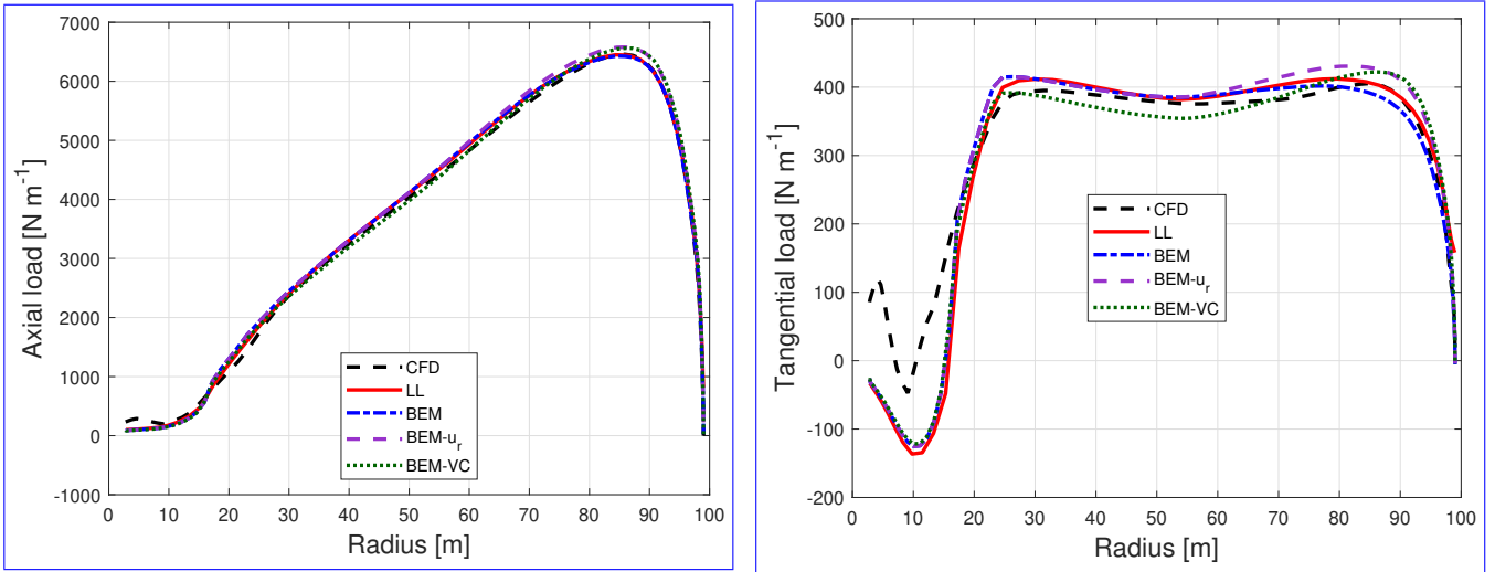
Figure 11. Comparison of out-of-plane axial load (left) and in-plane tangential load (right) of the dihedral blade W-1 calculated from CFD, lifting-line method (LL), BEM method, BEM with radial induction (BEM- u_r ) and the proposed BEM-VC method.
