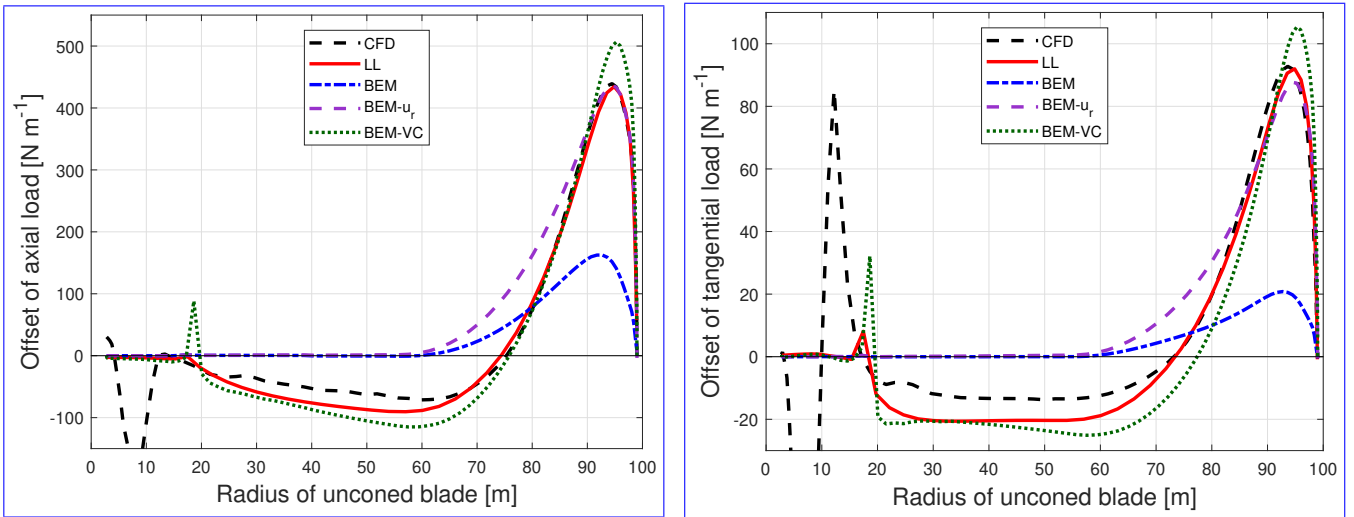
Figure B7. Comparison of the difference of the out-of-plane axial load (left) and in-plane tangential load (right) of the dihedral blade W-2 with 15° of cone downwind compared to the baseline blade with the same cone calculated from CFD, lifting-line method (LL), BEM method, BEM with radial induction (BEM- u_r ) and the proposed BEM-VC method.
