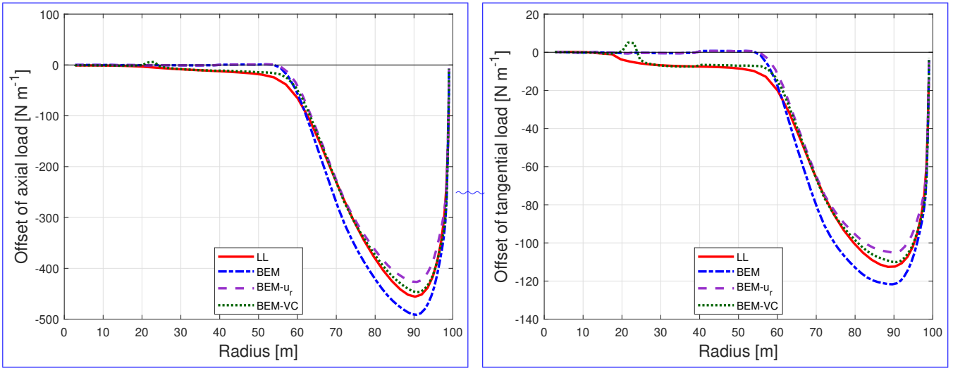
Figure 21. Comparison of the difference of the axial load (left) and tangential load (right) of the dihedral blade W-1-U15 compared to the baseline blade calculated from different models. The wind speed is 20 \text{ m s}^{-1} , the tip-speed-ratio is 4.5 and the additional twist angle \theta_p is 18.51^\circ .
