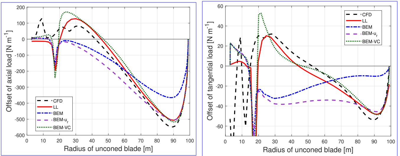
Figure 15. Comparison of the difference of the out-of-plane axial load (left) and in-plane tangential load (right) of the baseline blade with 15^\circ of cone downwind compared to the baseline blade without cone calculated from CFD, lifting-line method (LL), BEM method, BEM with radial induction (BEM- u_r ) and the proposed BEM-VC method.
