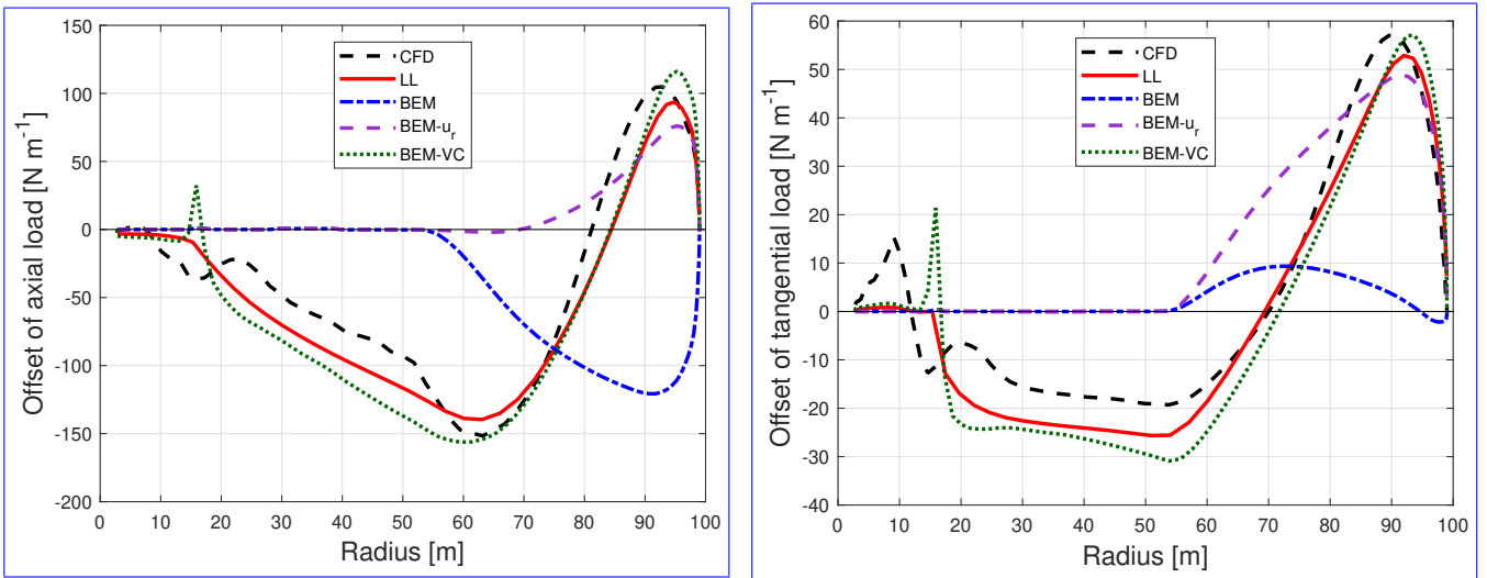
Figure 12. Comparison of the difference of the out-of-plane axial load (left) and in-plane tangential load (right) of the dihedral blade W-1 compared to the baseline blade calculated from CFD, lifting-line method (LL), BEM method, BEM with radial induction (BEM- u_r ) and the proposed BEM-VC method.
