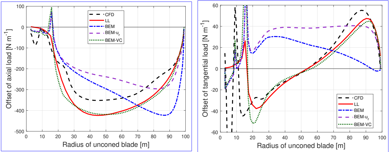
Figure 13. Comparison of the difference of the out-of-plane axial load (left) and in-plane tangential load (right) of the baseline blade with 15^\circ of cone upwind compared to the baseline blade without cone calculated from CFD, lifting-line method (LL), BEM method, BEM with radial induction (BEM- u_r ) and the proposed BEM-VC method.
