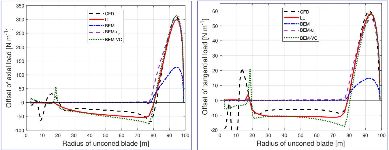
Figure B8. Comparison of the difference of the out-of-plane axial load (left) and in-plane tangential load (right) of the dihedral blade W-3 with 15° of cone downwind compared to the baseline blade with the same cone calculated from different aerodynamic models.
