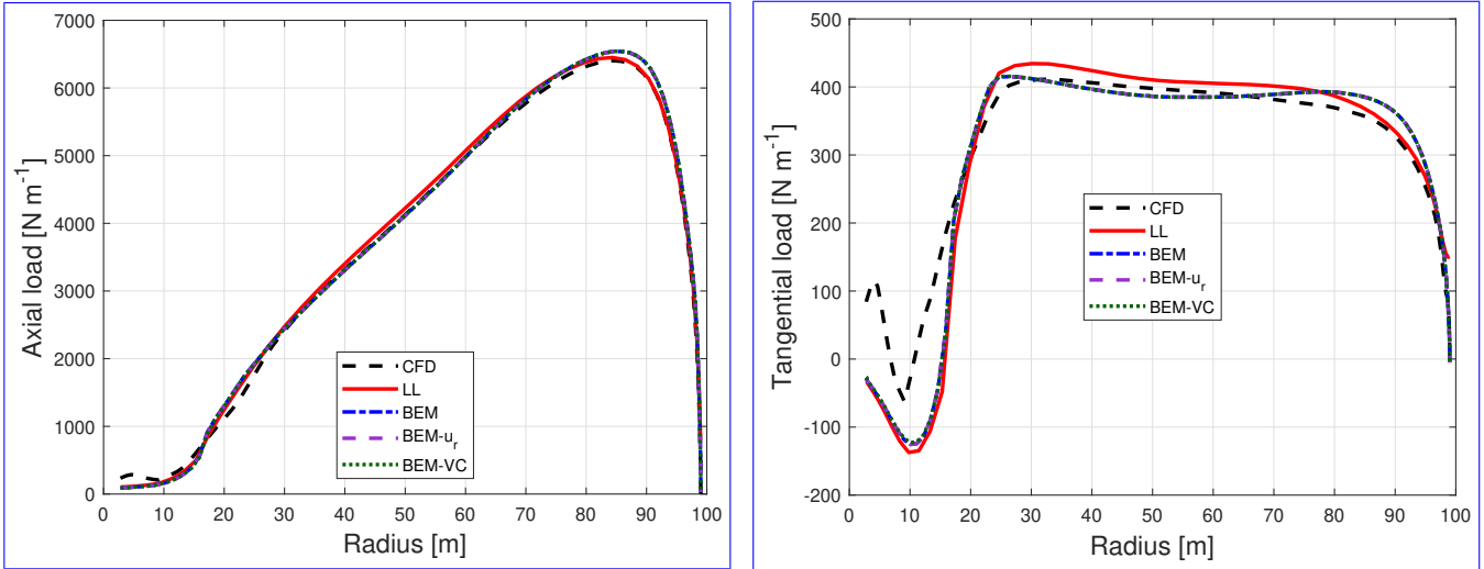
Figure 10. Comparison of out-of-plane axial load (left) and in-plane tangential load (right) of the baseline straight blade calculated from CFD, lifting-line method (LL), BEM method, BEM with radial induction (BEM- u_r ) and the proposed BEM-VC method. The results from three BEM variants coincide with each other as expected.
