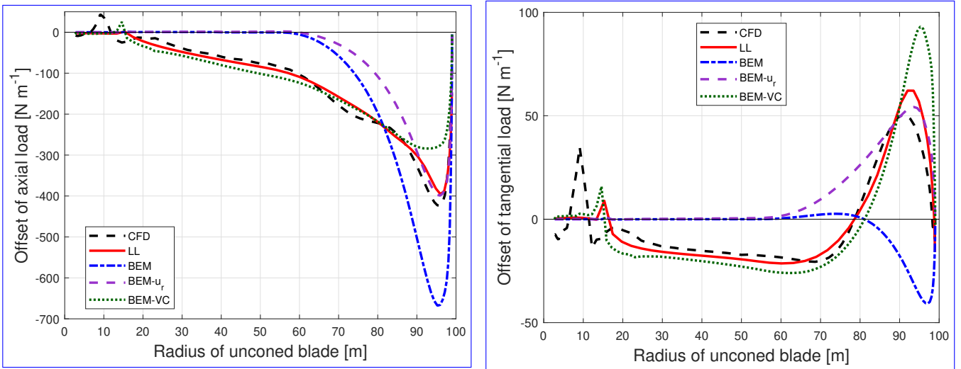
Figure B4. Comparison of the difference of the out-of-plane axial load (left) and in-plane tangential load (right) of the dihedral blade W-2 with 15° of cone upwind compared to the baseline blade with the same cone calculated from CFD, lifting-line method (LL), BEM method, BEM with radial induction (BEM- u_r ) and the proposed BEM-VC method.
