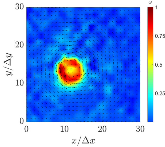
Figure 17. Instantaneous vorticity magnitude with the central differentiation scheme and quiver lines of the velocity field. RC1.5 The colorbar was added
