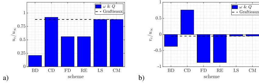
Figure 10. Average convection velocities. a) steamwise velocity. b) lateral velocity. RC1.3 Plots were updated using bar notation instead of a continuous line
