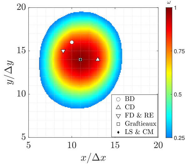
Figure 9. Vortex center locations for different differentiation schemes. The vorticity magnitude contour based on the least squares scheme is shown. The colorbar was added
