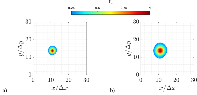
Figure 6. \Gamma_1 magnitude on the area of interest, where the methodology is applied after removing the average velocity from the field of view. a) 8-points. b) 24-points.
