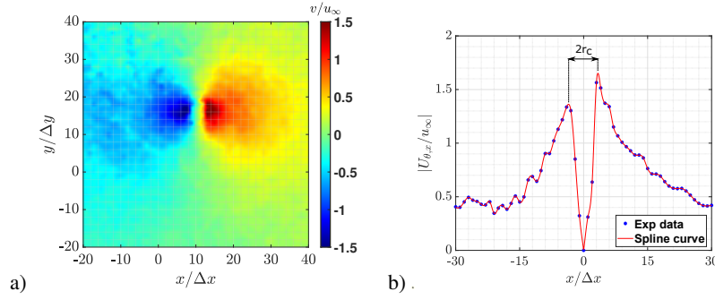
Figure 5. a) RC2.7: Induced velocity field v'(x, y) . b) Swirling velocity with the x-axis shifted to the corresponding vortex center.
