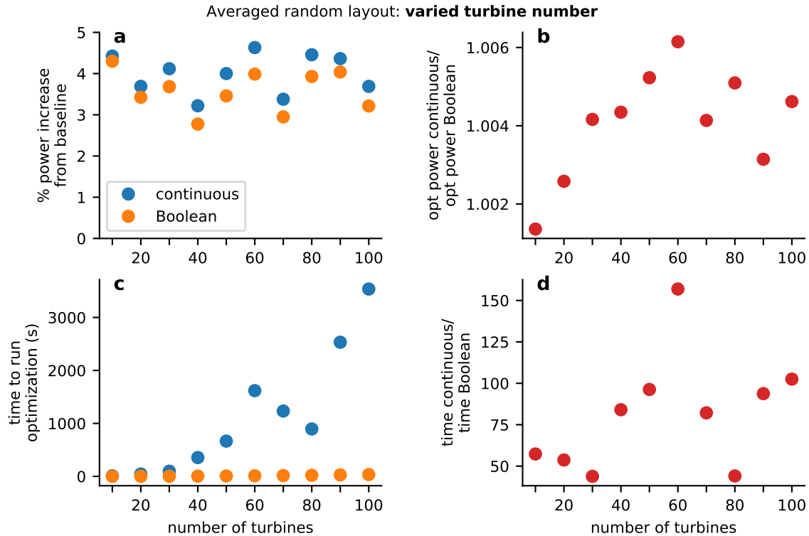
Figure 10. Comparison of a wind plant optimized with a traditional continuous approach compared to our novel Boolean optimization. The results in this figure are the averaged results for 7 randomly generated wind turbine layouts for plants with different numbers of turbines. For the purposes of this figure, the average spacing was constant at 5 rotor diameters while each subfigure shows different metrics as a function of the number of wind turbines. Figure 9a shows the absolute percent increase in power over the nonyawed baseline for the continuous and Boolean optimizations. Figure 9b shows the ratio of the optimized power with the continuous approach to the optimized power with the Boolean approach. Figure 9c shows the absolute time required to run each optimization, again for the continuous and Boolean optimizations. Figure 9d shows the ratio of the time required to optimize with the continuous approach to the time required to optimize with the Boolean approach.
