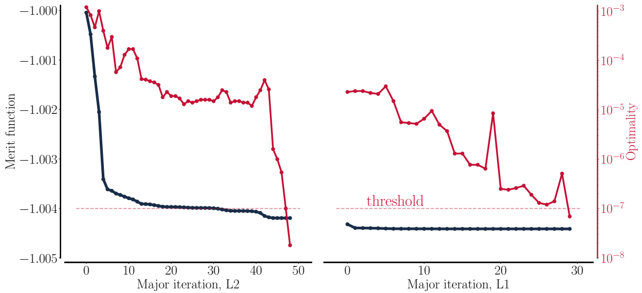
Figure 12. Full optimization procedure using grid sequencing: The result from grid level L2 (left) is used as a starting point on grid level L1 (right) to save time. The optimizations are called SPL2e3cb and SPL1e3hb and also figure both in Tab. 6 and in Fig. 10.
