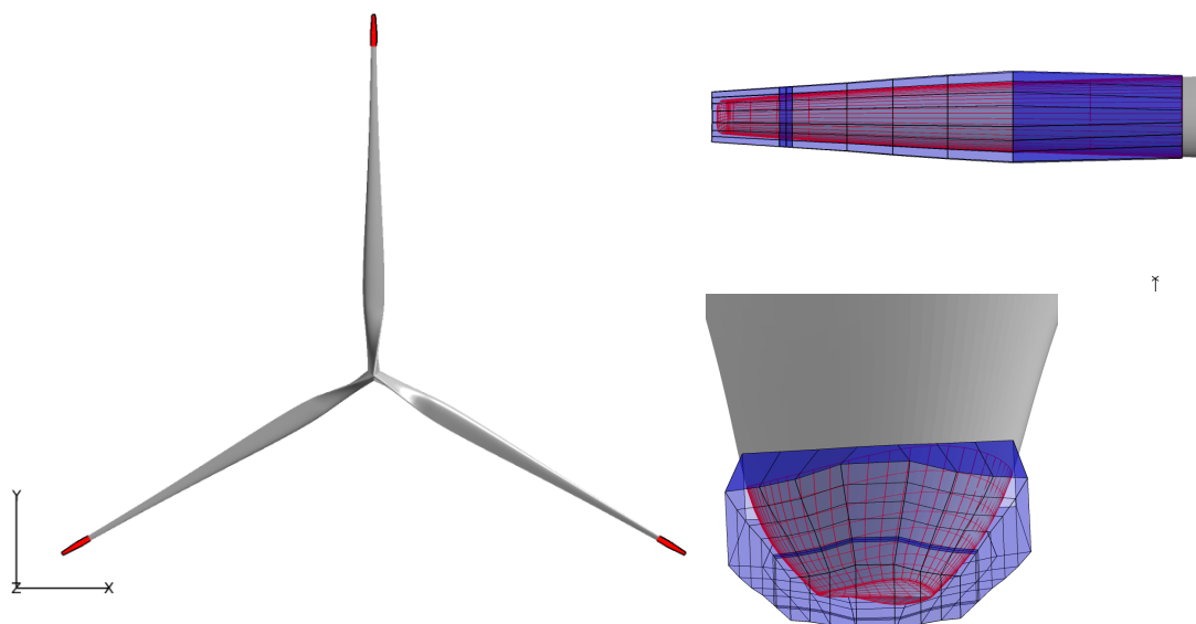
Figure 7. Overview of baseline rotor (gray), deformable tip region (red), and FFD boxes (blue). Grid level 3 is used to visualize mesh lines.
