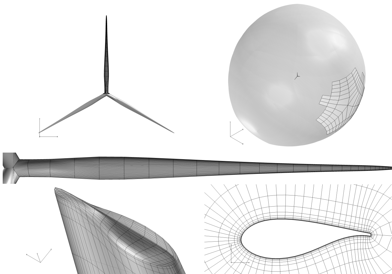
Figure 3. Surface (upper, left) and volume (upper, right) where a close-up one of the blade meshes is given below. Visualization of tip cap mesh (lower, left) and a view of the airfoil discretization is also offered (lower, right). Notice, that for clarity only 1 out of 4 mesh lines is shown. Inflow (transparent gray) and outflow (gray with black mesh lines) zones are visualized in the upper right plot.
