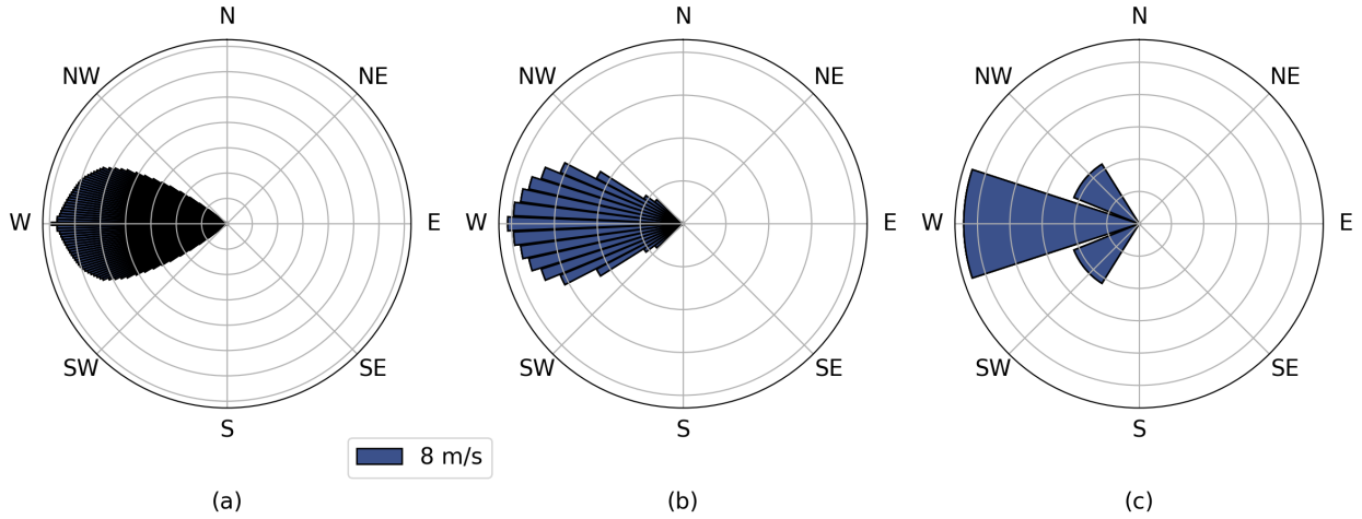
Figure 8. The wind rose used for the layout optimization studies performed in Section 4. The resolution of the wind direction bins varies from 1° (left) to 5° (center) to 40° (right). The wind speed is a constant 8 m/s.
