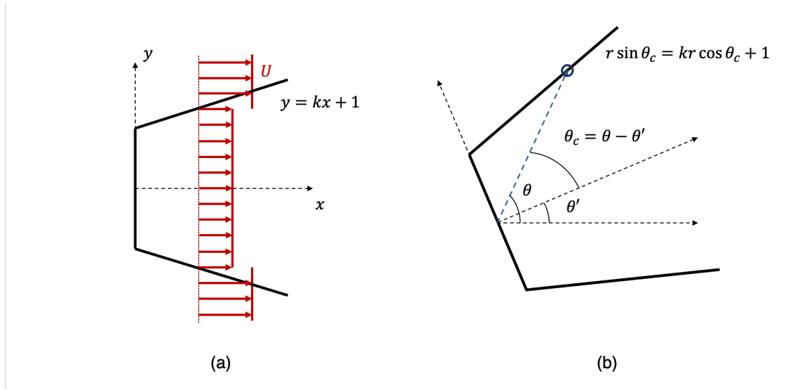
Figure 2. Left: a schematic of the top-hat wake model in Cartesian coordinates with the wind aligned with the x-direction. Right: the wake region in polar coordinates, rotated by a wind direction \theta' , with the wake boundary defined by the angle \theta_c .
