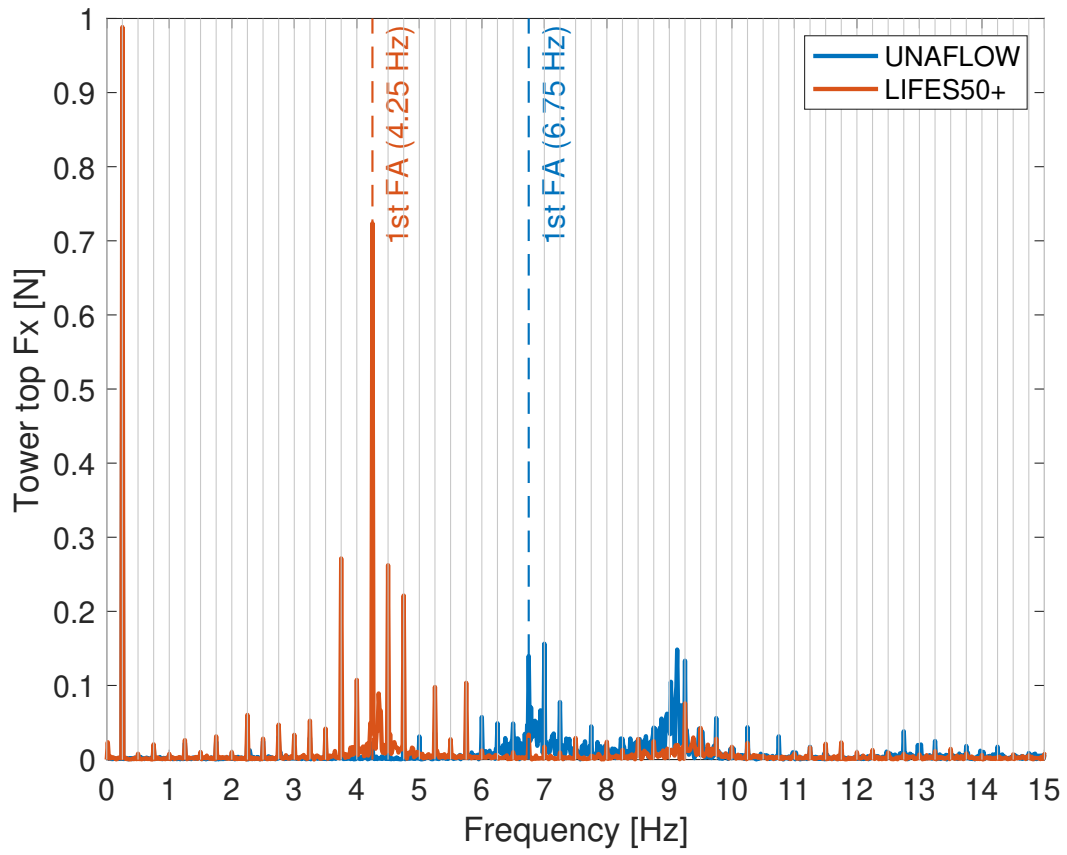
Figure 1: Spectrum of the tower-top FA shear-force for the same surge-motion ( A = 0.1\text{m} , f = 0.25\text{Hz} ) and no wind measured in the LIFES50+ and UNAFLOW experiments. The vertical lines mark the integer multiples of the surge-motion frequency.
