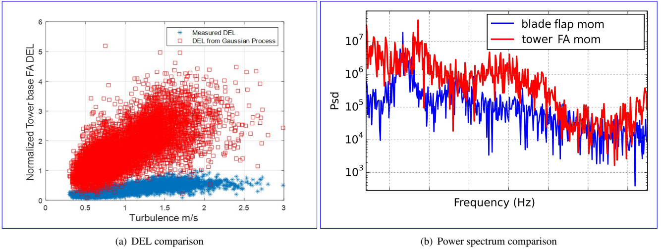
Figure 9. a) Comparison of the 10-minute Tower base fore-aft damage equivalent moment with measurements at 7 m/s using the Gaussian process method without Vanmarcke correction. b) Comparison of the power spectrum of the tower base moment showing the small increase in energy in its first peak with the corresponding much larger peak in the blade root flap moment
