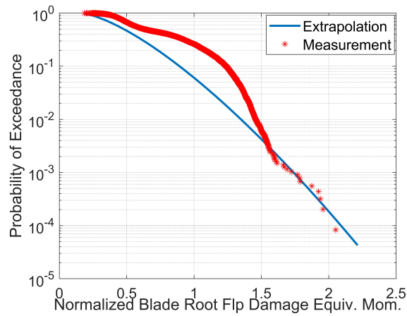
(a) 7 m/s
