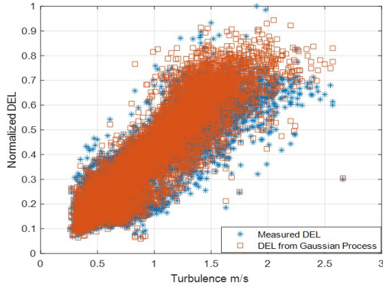
(a) 7 m/s wind speed
