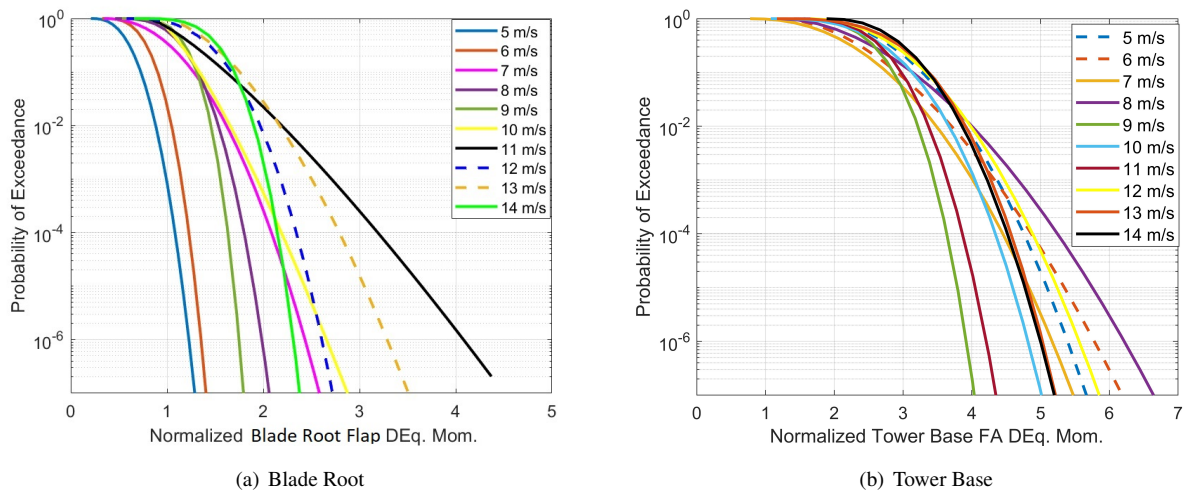
Figure 7. Comparison of the 10-minute extrapolated blade root flap bending damage equivalent moments and the extrapolated tower base fore-aft damage equivalent moment using simulations.
