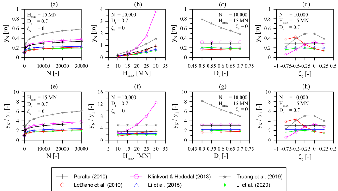
280 Figure 2: Results of the parameter study on the pile head displacement accumulation and the influence of different input variables – comparison of the prediction models given in Table 1.
