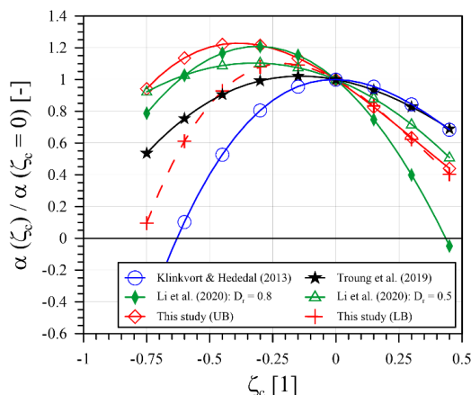
620 Figure 9: Normalized accumulation parameter ( \alpha ) with cyclic load ratio ( \zeta_c ) for different approaches and comparison with the proposed lower bound (LB) and upper bound (UB) curves.
