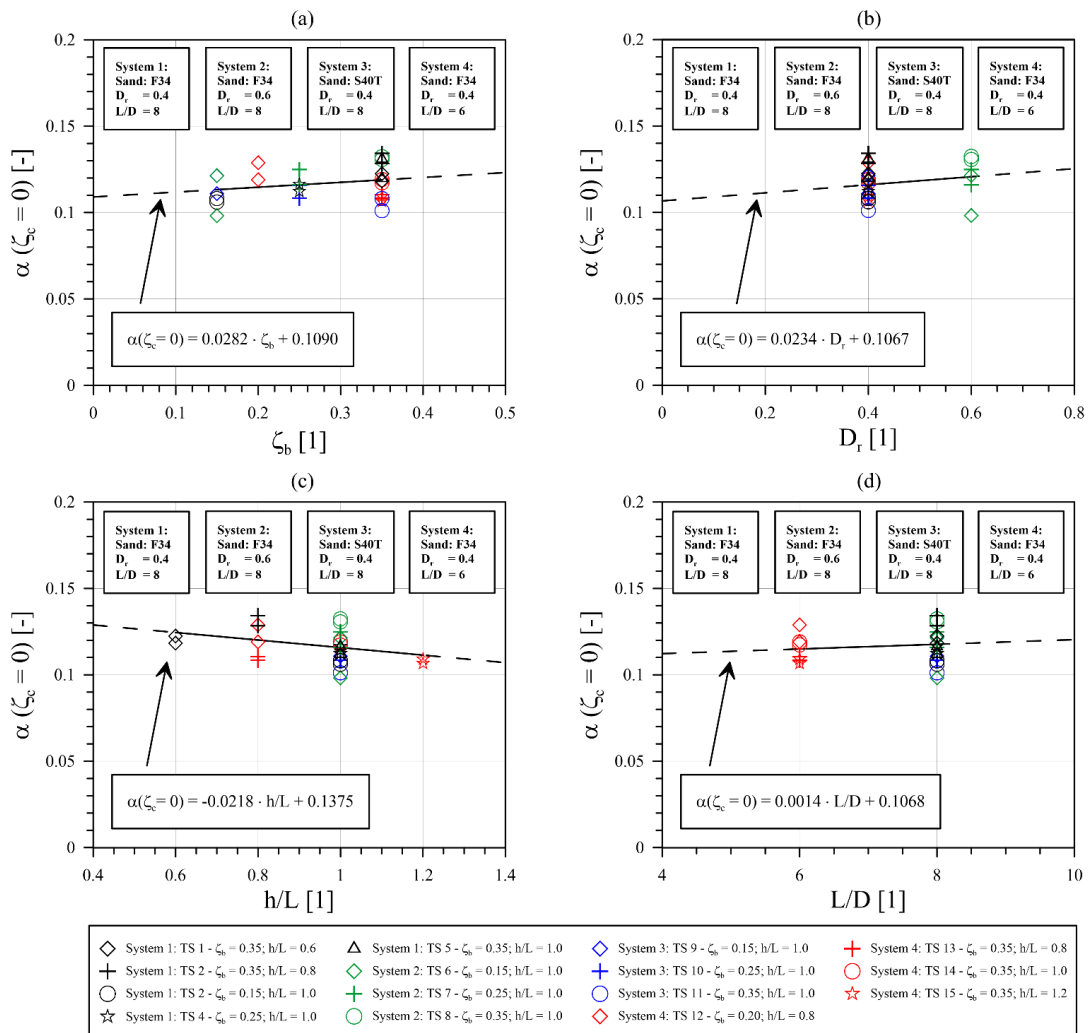
Figure 7: Evaluation of cyclic test results – Relationship of the accumulation parameter \alpha for \zeta_c = 0 with (a) load magnitude \zeta_b , (b) soil relative density D_r , (c) normalized load eccentricity h/L and (d) normalized embedment length L/D .
