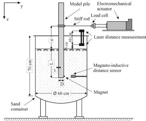
Figure 3: Schematic of experimental test set-up.
