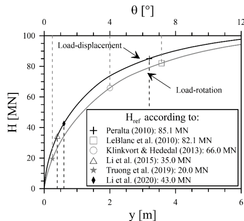
250 Figure 1: Monotonic load-deformation response of a horizontally loaded pile ( D = 8 \text{ m} , t = 0.08 \text{ m} , L = 32 \text{ m} , h = 32 \text{ m} ) in dense sand calculated with the p-y method according to Thieken et al. (2015) and reference loads ( H_{ref} ) defined by different criteria (see Table 2).
