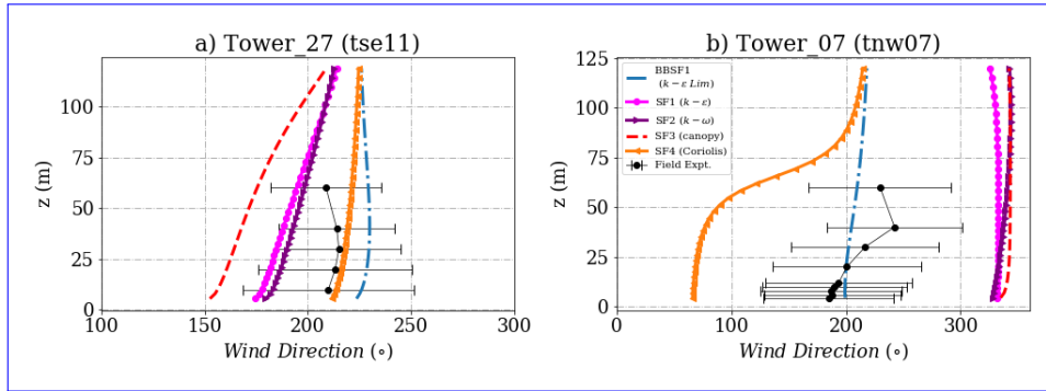
Figure 14. Simulation results and experimental data for wind direction inside the valley for a) Tower 27 (tse11) b) Tower 7 (tnw07). The locations of the masts are given in Fig. 2.
