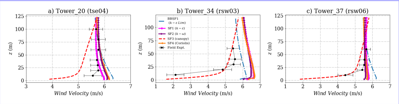
Figure 6. Simulation results and experimental data for wind velocity on the Southwest ridge for a) Tower 20 (tse04) b) Tower 34 (rsw03) c) Tower 37 (rsw06). The locations of the masts are given in Fig 2.
