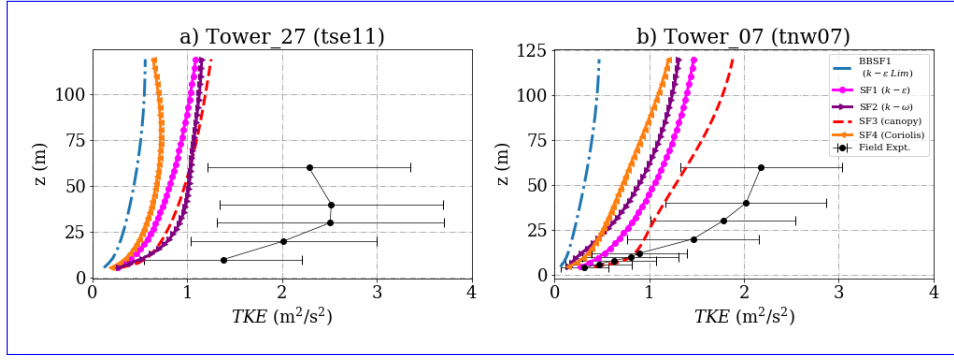
Figure 12. Simulation results and experimental data for turbulent kinetic energy inside the valley for a) Tower 27 (tse11) b) Tower 7 (tnw07). The locations of the masts are given in Fig. 2.
