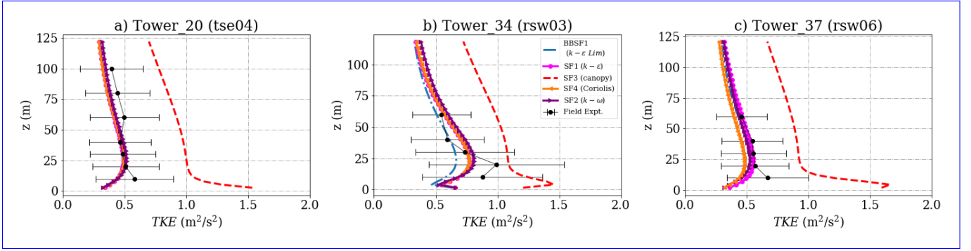
Figure 7. Simulation results and experimental data for turbulent kinetic energy on the Southwest ridge for a) Tower 20 (tse04) b) Tower 34 (rsw03) c) Tower 37 (rsw06). The locations of the masts are given in Fig 2.
