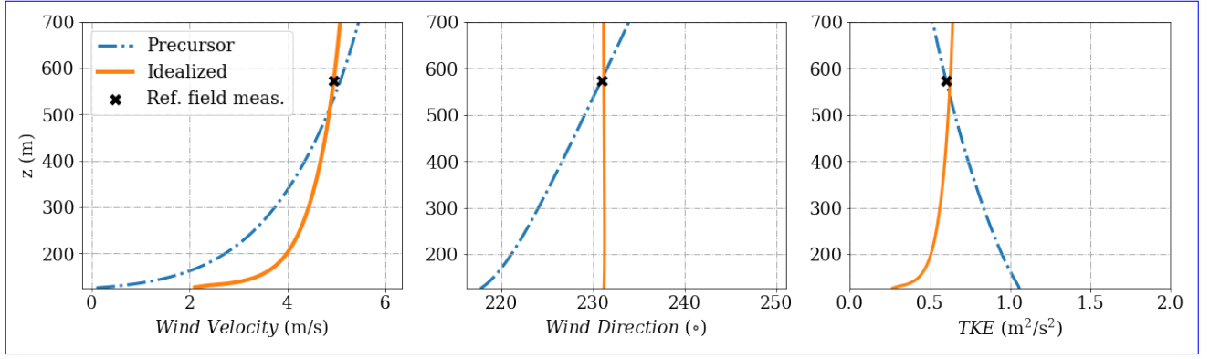
Figure 26. Idealized and Precursor (developed) input profiles for a) Wind velocity magnitude b) Wind direction c) Turbulent kinetic energy tuned to reach calibration at height 573 m corresponding to 100 m at Tower 20 (tse04)
