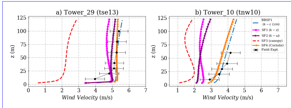
Figure 16. Simulation results and experimental data for wind velocity on the Northeast ridge for a) Tower 29 (tse13) b) Tower 10 (tnw10). The locations of the masts are given in Fig. 2.
