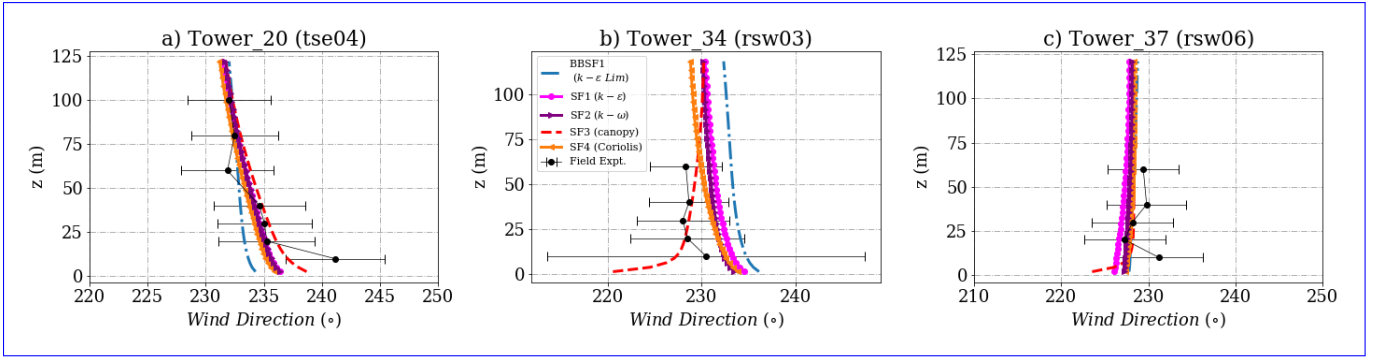
Figure 8. Simulation results and experimental data for wind direction on the Southwest ridge for a) Tower 20 (tse04) b) Tower 34 (rsw03) c) Tower 37 (rsw06). The locations of the masts are given in Fig 2.
