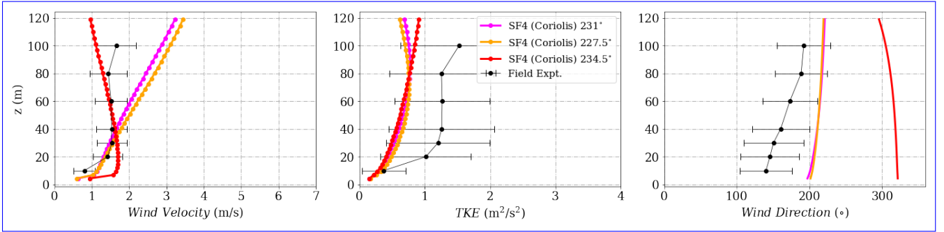
Figure 34. a) Wind velocity magnitude b) Wind direction c) Turbulent kinetic energy at Tower 25 (tse09) for the SF4 (Coriolis) model.
