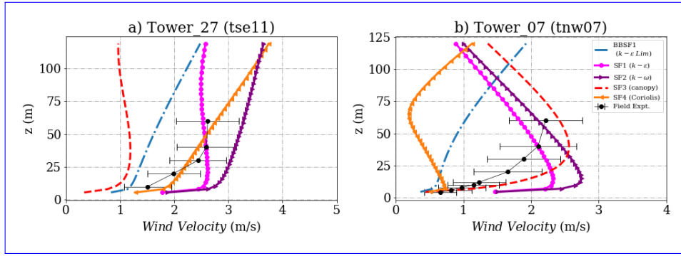
Figure 10. Simulation results and experimental data for wind velocity inside the valley for a) Tower 27 (tse11) b) Tower 7 (tnw07). The locations of the masts are given in Fig. 2.
