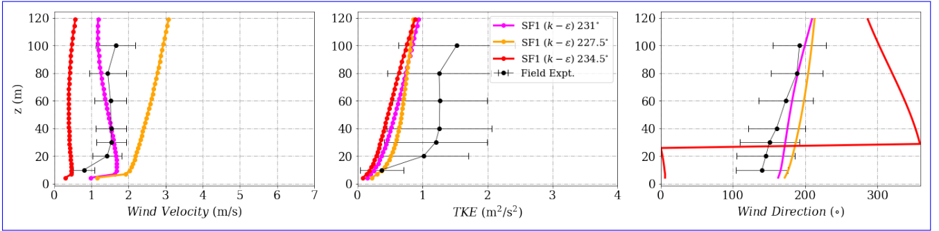
Figure 20. Simulation results and experimental data wind velocity inside the valley Tower 25 (tse09).
