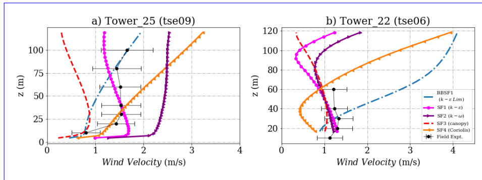
Figure 9. Simulation results and experimental data wind velocity inside the valley for a) Tower 25 (tse09) b) Tower 22 (tse06). The locations of the masts are given in Fig. 2.
