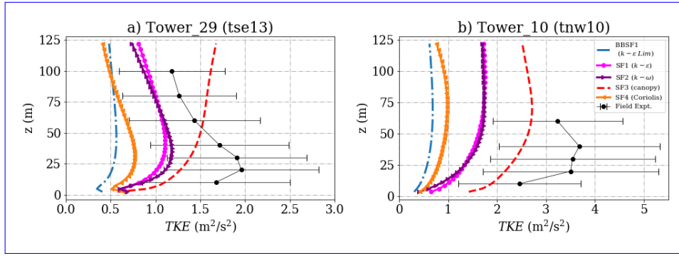
Figure 17. Simulation results and experimental data for turbulent kinetic energy on the Northeast ridge for a) Tower 29 (tse13) b) Tower 10 (tnw10). The locations of the masts are given in Fig. 2.
