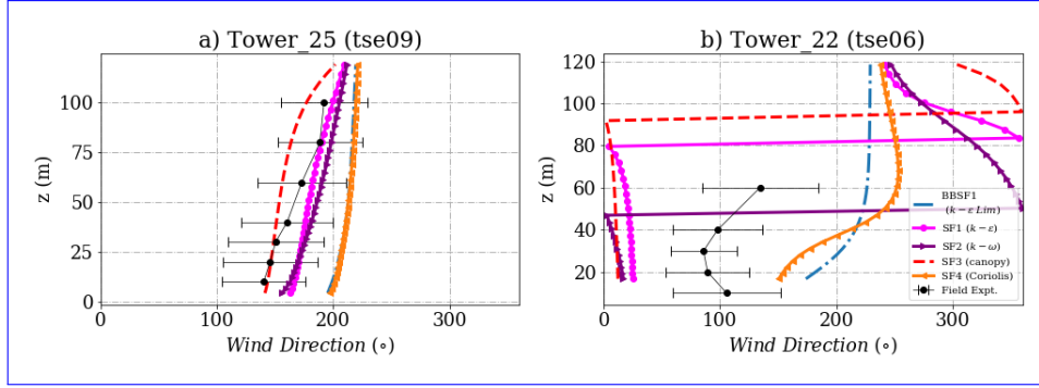
Figure 13. Simulation results and experimental data for wind direction inside the valley for a) Tower 25 (tse09) b) Tower 22 (tse06). The locations of the masts are given in Fig. 2.
