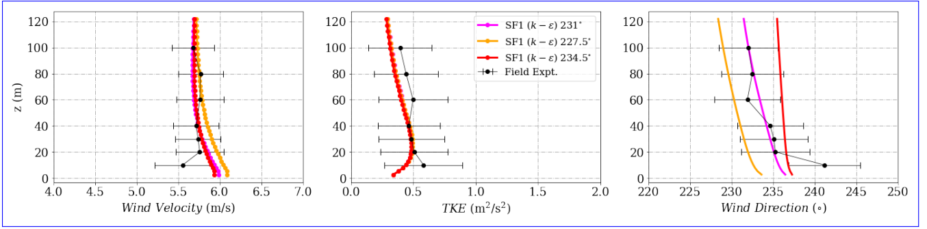
Figure 19. Simulation results and experimental data for wind velocity on the Southwest ridge for a) Tower 20 (tse04). The locations of the masts are given in Fig 2.
