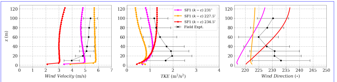
Figure 21. Simulation results and experimental data for wind velocity on the Northeast ridge for Tower 29 (tse13).
