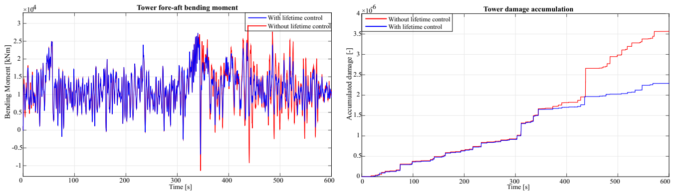
Figure 13. Tower fatigue load mitigation for 14 m/s wind
