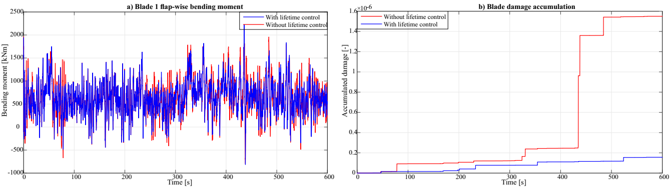
Figure 7. Blade fatigue load mitigation
