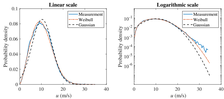
Figure 4. Marginal distribution of u with Weibull fitting
