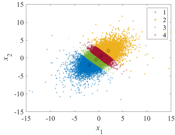
Figure 1. k -means clustering of t distribution sample
