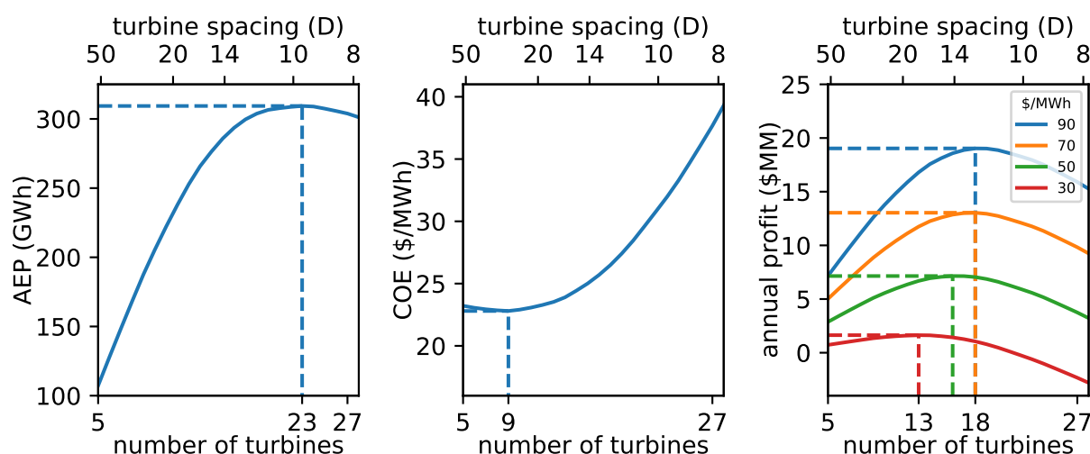
Figure 5. Different objectives as a function of the number of turbines in the wind power plant. For this example, the turbines are in line with the wind direction and are equally spaced in a wind power plant with a fixed length. From left to right, the objectives represented here are annual energy production (AEP), cost of energy (COE), and annual profit.
