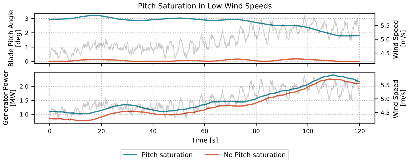
Figure 10. A sample 2-minute time series from a 10-minute turbulent simulation of the IEA 15-MW wind turbine showing how increased blade pitch angles can increase power output at low wind speed. The rotor-averaged wind speeds are plotted in grey in the background.
