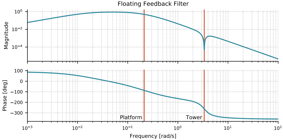
Figure 11. A Bode plot showing the filter used for the tower-top motion feedback signal for the IEA 15-MW turbine on the UMaine semisubmersible platform. The first platform and tower fore-aft natural frequencies are shown in red and labeled accordingly. These natural frequencies are inputs to the ROSCO tuning process to shape this filter.
