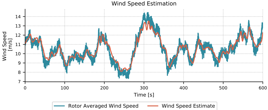
Figure 5. Wind speed estimator results for the NREL 5-MW wind turbine with 10 minutes of simulation time and an average wind speed of 11 m/s.
