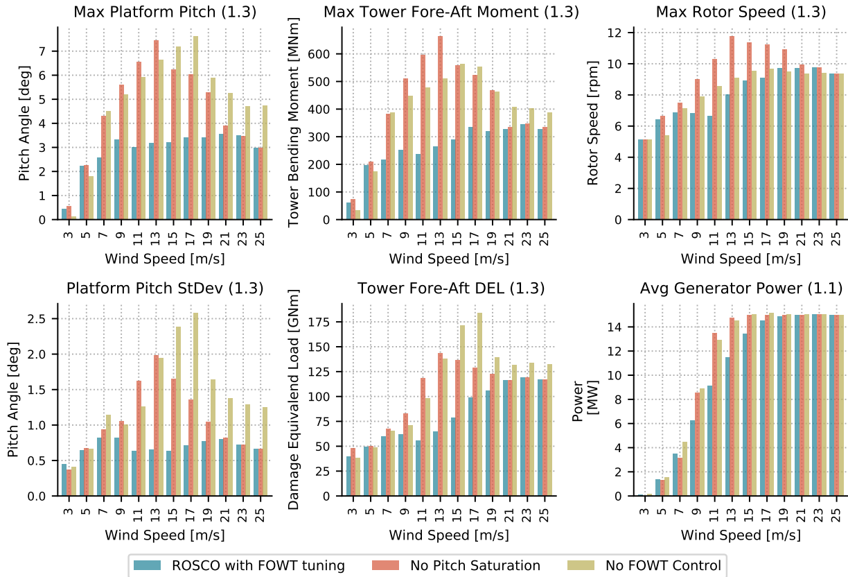
Figure 13. Results from DLC 1.1 and 1.3 simulations for the IEA 15-MW wind turbine on the UMaine semisubmersible platform. Output statistics from the platform pitch angles, tower base fore-aft bending moments, rotor speed, and generator power are shown. Simulations using the FOWT feedback loop ( \beta_{float} ) and pitch saturation are compared to those with the pitch saturation or FOWT feedback modules turned off.
