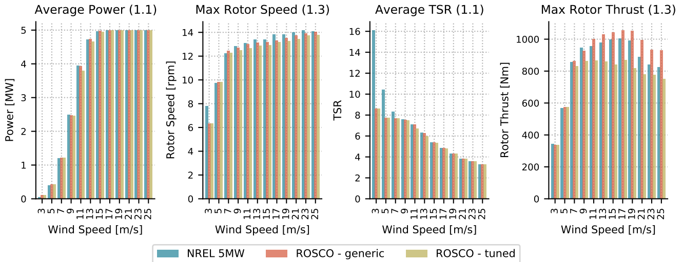
Figure 12. Results from simulations of the NREL 5-MW land-based wind turbine. Average power, maximum rotor speeds, average TSRs, and maximum rotor thrusts are shown for DLCs 1.1 and 1.3. The dynamic results from the ROSCO controller are comparable to those from the NREL 5-MW reference controller. “ROSCO - generic” refers to ROSCO with the most generic tuning methods, and “ROSCO - tuned” refers to ROSCO with tuned set point smoother gains and peak shaving implemented.
