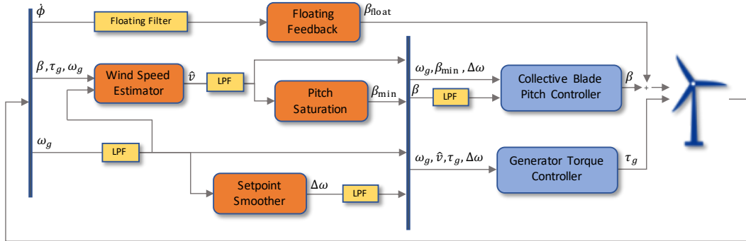
Figure 3. A block diagram showing the general controller logic in ROSCO. The generator torque and collective blade pitch controllers described in sections 3 and 4, respectively, are shown in blue. The orange squares denote the various controller modules that are described in Section 5. The yellow squares are filters. The details of the floating filter are described in Section 5.5, and the standard low-pass filter implementations are provided in Appendix A. For the feedback signals, \phi is the tower-top pitch angle, \beta is the collective blade pitch angle, \omega_g is the generator speed, and \tau_g is the generator torque. For outputs from the controller modules, \beta_{float} is the floating controller’s contribution to the blade pitch angle (see Section 5.5), \beta_{min} is the minimum blade pitch angle (see Section 5.3), \hat{v} is the estimated wind speed (see Section 5.1), and \Delta\omega is a controller reference set point shifting term from the setpoint smoother (see Section 5.2).
