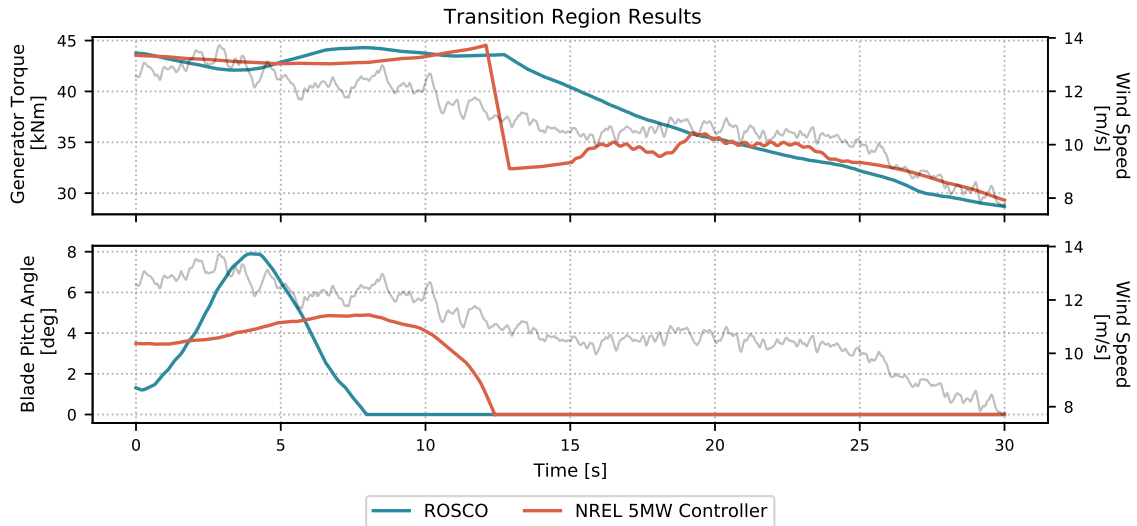
Figure 7. Time-domain simulation results from the NREL 5-MW wind turbine near rated wind speeds. The rotor-averaged wind speed is plotted in the background as grey curves in each plot.
