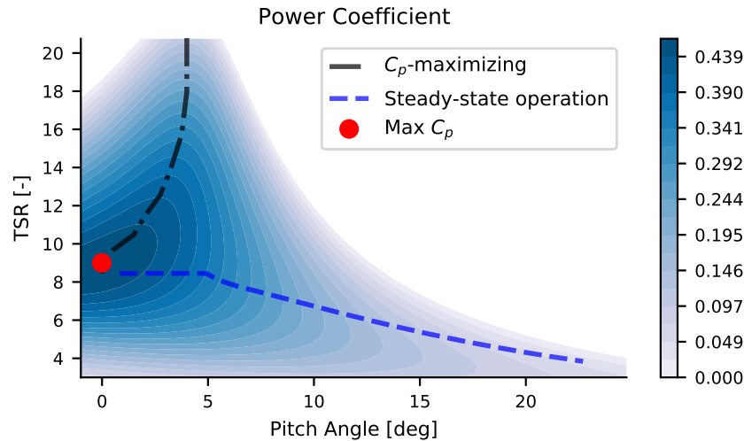
Figure 4. C_p surface for the IEA 15-MW wind turbine. The dash-dotted black line shows the below-rated steady-state operating points that result from a C_p -maximizing minimum pitch schedule at low wind speeds when the turbine has a minimum rotor speed constraint. The dashed blue line shows the expected steady-state operation points that are used to calculate the controller gain schedules.
