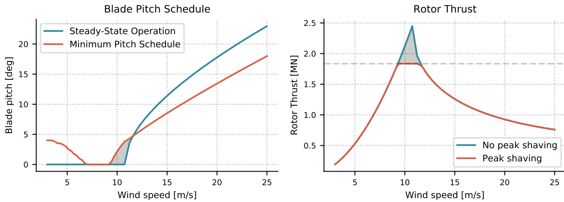
Figure 8. Expected steady-state pitch saturation for the IEA 15-MW wind turbine, based on the C_t surface calculated with cc-blade. The blade pitch schedule (left) shows the expected steady-state value of the pitch angle along with the imposed minimum pitch angles with pitch saturation for both peak shaving and power maximization in low wind speeds. The righthand plot shows the expected rotor thrust with and without peak shaving. The grey region in the blade pitch schedule corresponds to the pitch angles that result in a rotor thrust above the maximum allowable thrust, shown as the grey region in the righthand plot.
