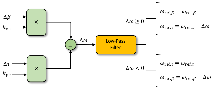
Figure 6. A block diagram of the set point smoother logic defined in (43)–(44) is shown here. The term \Delta\omega shifts the blade pitch or generator torque controller to help avoid unwanted controller interactions.
