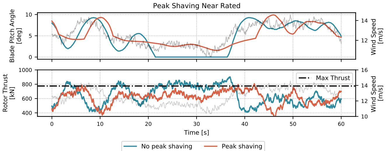
Figure 9. A sample 1-minute time series from a 10-minute turbulent simulation of the NREL 5-MW wind turbine to showcase the peak shaving routine in ROSCO. The peak shaving percentage was tuned to 20% for this simulation. The wind speed is shown in the background of each plot, and the maximum allowable thrust is denoted by the dash-dotted black line in the lower plot.
