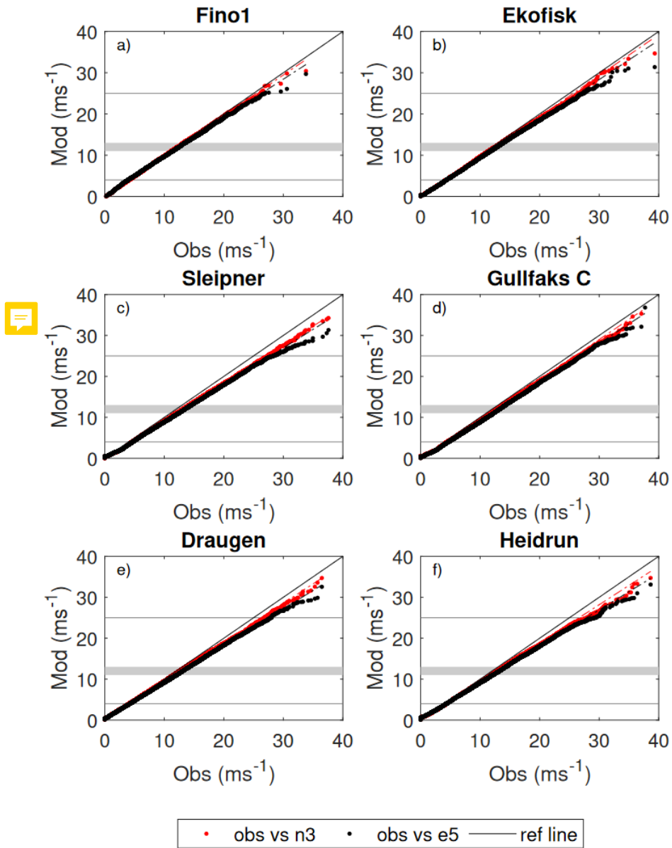
Figure 2. Quantile-quantile plot between the observed wind speed (obs) and the modeled (mod) wind speed; NORA3 (red) and ERA5 (black), for all the six offshore sites.
