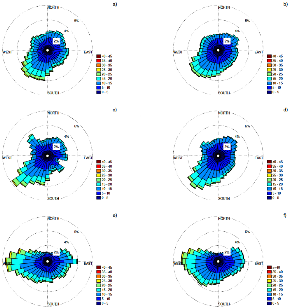
Figure A1. Observed (left column) and modeled (right column) wind roses for the five oil- and gas platforms. The colorbar show the wind speed intervals in meters per second. a-b) Heidrun; c-d) Draugen; e-f) Gullfaks C; g-h) Sleipner; i-j) Ekofisk
