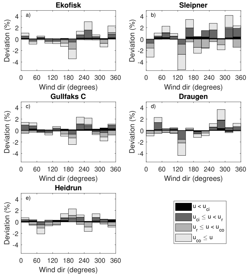
Figure 5. Difference in the occurrence (%) of wind events categorized in different wind direction-intervals ( 30^\circ -intervals) between NORA3 and observations (model-obs) for a) Ekofisk; b) Sleipner; c) Gullfaks C; d) Draugen; e) Heidrun. For each wind direction interval the wind events are divided into four different wind speed categories, the first one corresponds to u < u_{ci} , the second is the wind speed interval where the wind power is a function of the wind speed cubed ( u_{ci} \leq u < u_r ), the third interval contain the wind speeds corresponding to rated wind power production ( u_r \leq u < u_{co} ), and the last interval is where the wind speeds are too strong resulting in a terminated wind power production ( u_{co} \leq u ).
