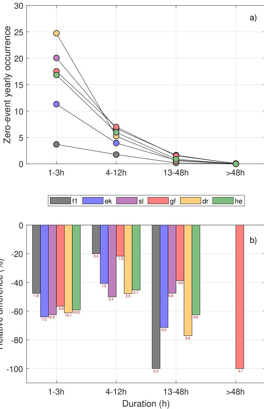
Figure 10. a) Yearly occurrence and corresponding duration of observation-based zero-events caused by to wind speeds higher than cut-out wind speed ( u \geq u_{co} ). b) The differences between model-based (n3) and observation-based (obs) zero-event occurrences divided by the total number of observed occurrences of “too high” wind speeds. Values over or under each bar correspond to the differences (n3-obs) in the number of yearly occurrences between the model and observations. Abbreviations: f1: Fino1; ek: Ekofisk; sl: Sleipner; gf: Gullfaks C; dr: Draugen; he: Heidrun.
