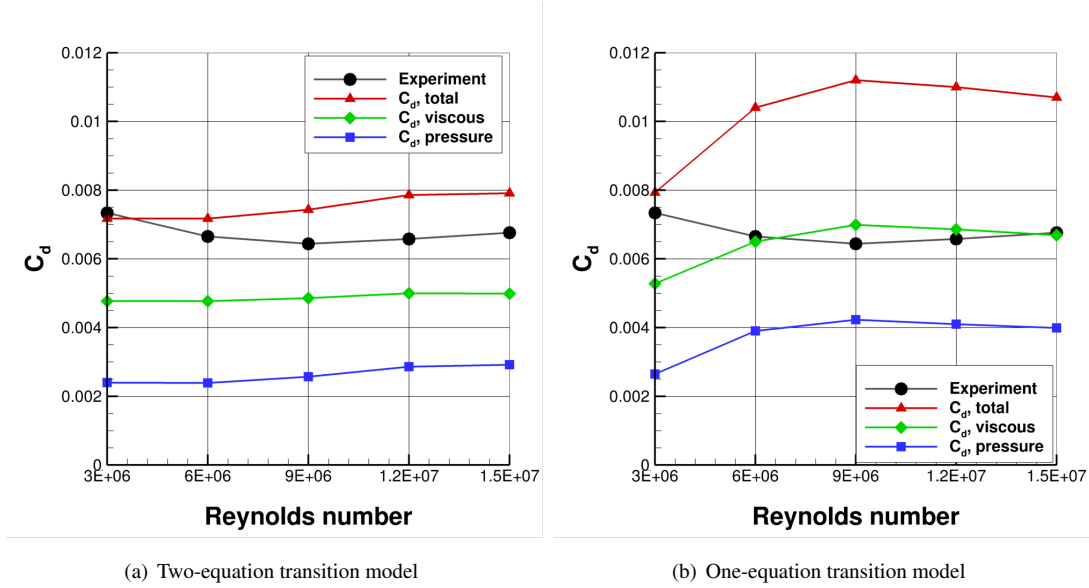
Figure 8. Drag coefficient breakdown for DU00-W-12 airfoil and comparison with experiment at 4^\circ angle of attack and various Reynolds number
