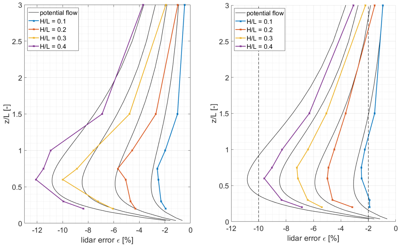
Figure 6: Lidar error \varepsilon in dependence of the ratio H/L between z/L ratios from 0 to 3 for a roughness length of z_0 of 0.005 m. Left: Based on results from WASP Engineering. Right: Based on results from Meteodyn WT. The black lines show results from the potential flow model.
