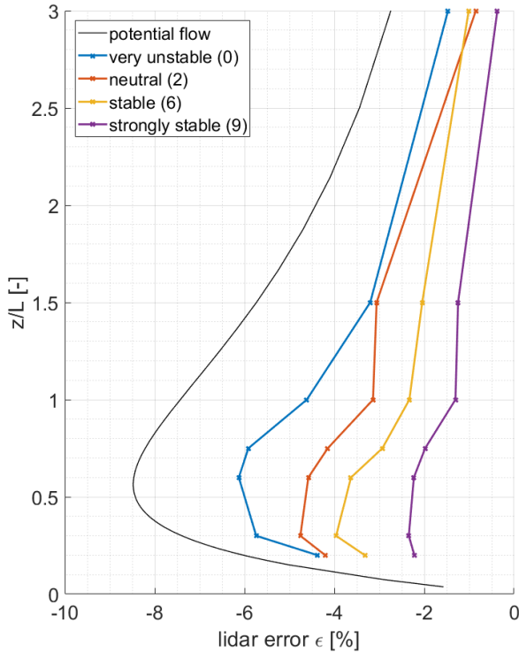
Figure 12: Lidar error \epsilon in dependence of atmospheric stability between z/L ratios from 0 to 3. Results are based on Meteodyn WT (colored) and the potential flow model (black) for an H/L ratio of 0.3. Results are shown for the forested case with a tree height h_t = 20\text{ m} and medium forest density.
