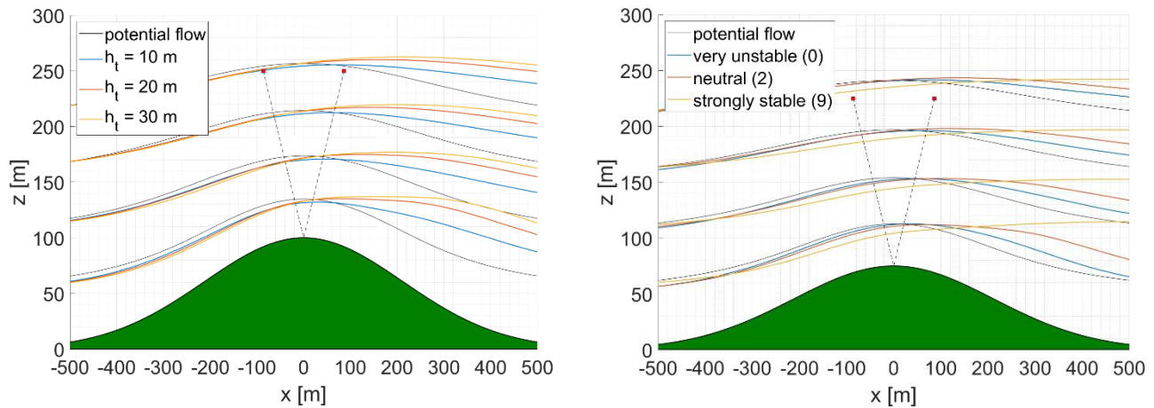
Figure 13: Streamlines in dependence of tree height h_t (left) and atmospheric stability class (right) for an H/L ratio of 0.3. Streamlines from Meteodyn WT (coloured) and from the potential flow model (black) are starting at z of 50, 100, 150 and 200 m in front of the hill. Lidar measurement points at 150 m measurement height with a \phi of 30^\circ are marked in red.
