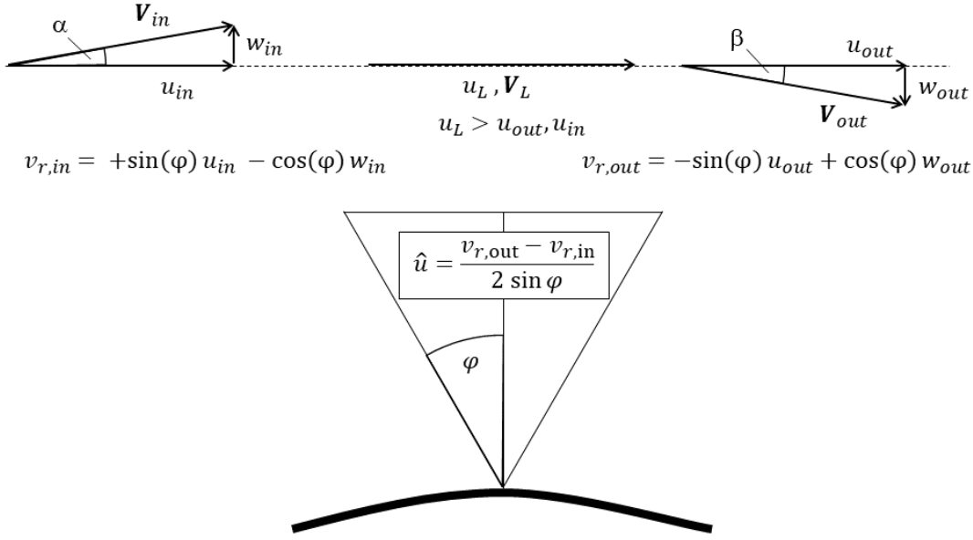
305 Figure 4: Generic flow case with a lidar placed on a hill-top. As a typical complex terrain example, this case shows a lidar placed on top of a hill within symmetric flow conditions. The changing vertical wind speed component introduces a lidar error. Additionally, there is a speed-up effect on the horizontal component, which causes a part of the total lidar error.
