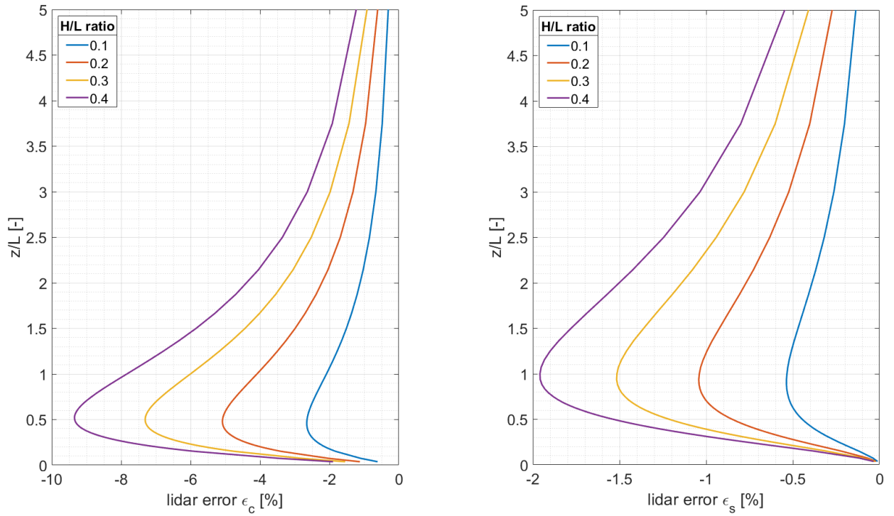
Figure 7: Lidar error \epsilon_c (left) and \epsilon_s (right) in dependence of the ratio H/L between z/L ratios from 0 to 5. Results are based on the potential flow model. Note the different scaling of the x-axes.
