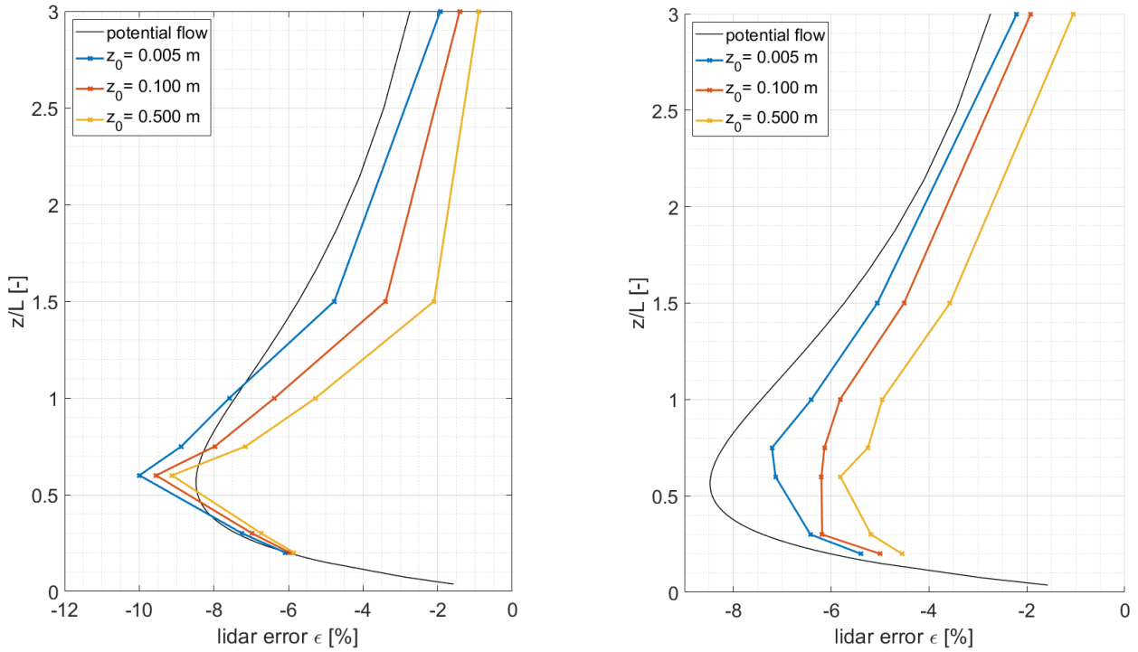
450 Figure 10: Model comparison between WAsP Engineering (left) and Meteodyn WT (right) for different roughness lengths for a H/L ratio of 0.3. Lidar error \varepsilon in dependence of the roughness length z_0 between z/L ratios from 0 to 3. Results from the potential flow model (black) are shown as a reference.
