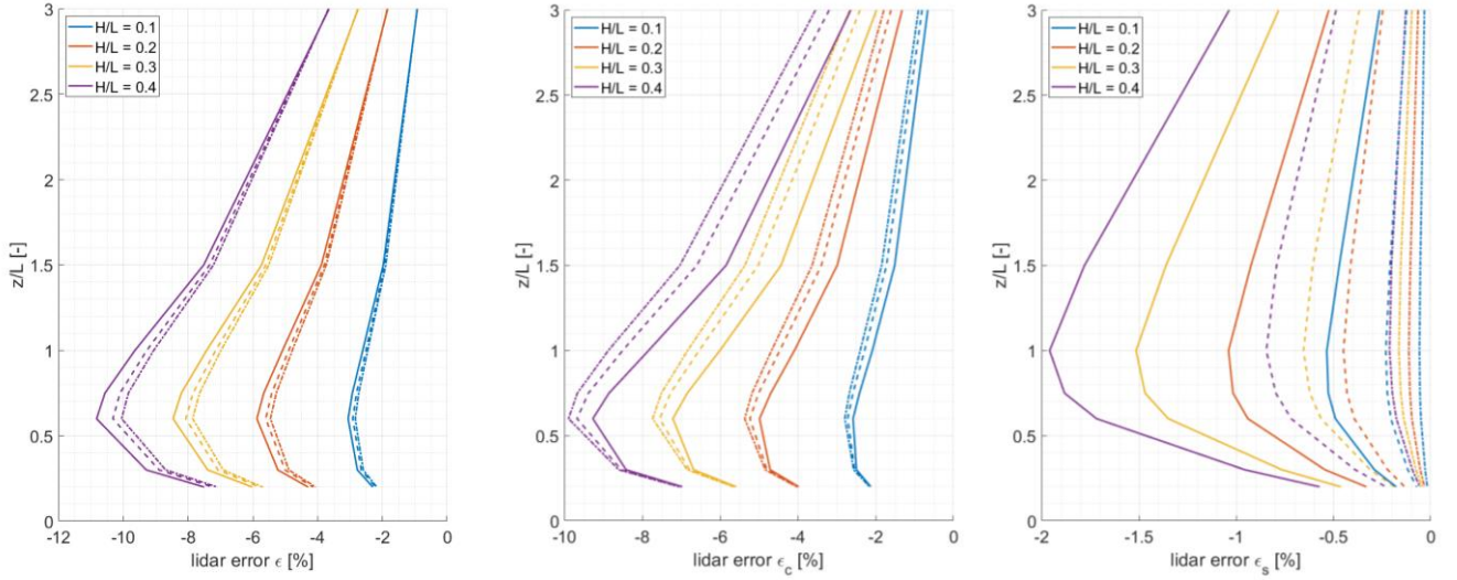
Figure 8: Lidar error \varepsilon (left), \varepsilon_c (middle) and \varepsilon_s (right) in dependence of the H/L ratio for the half-cone opening angles \varphi of 30^\circ (solid lines), 20^\circ (dashed lines) and 10^\circ (dot-dashed lines) between z/L ratios from 0 to 3 (left). Results are based on the potential flow model.
