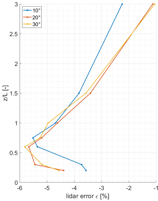
Figure 9: Lidar error \varepsilon for an H/L ratio of 0.3 for the three different half-cone angles \varphi of 30^\circ , 20^\circ and 10^\circ between z/L ratios from 0 to 3 (left). Results are based on Meteodyn WT for a roughness length z_0 of 0.5 m.
