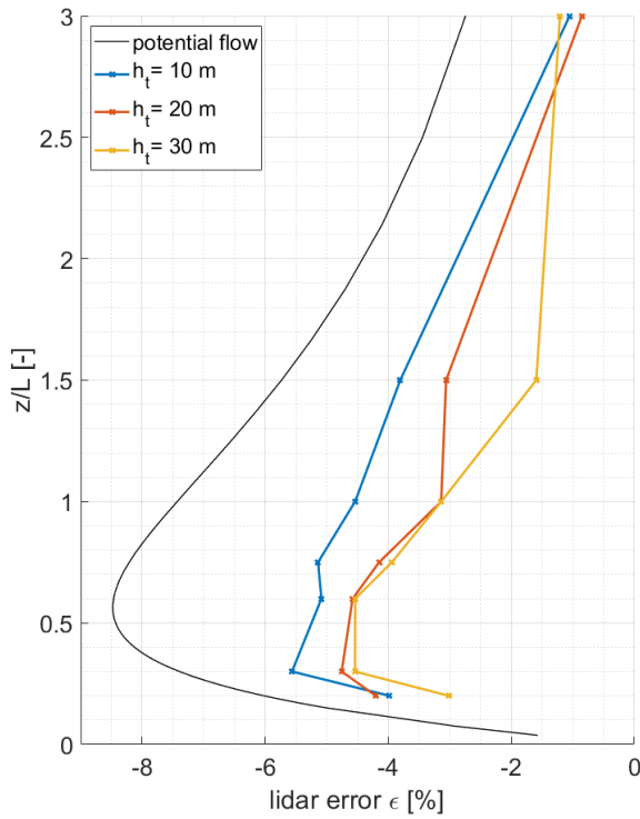
Figure 11: Lidar error \varepsilon in dependence of tree heights h_t between z/L ratios from 0 to 3. Results are based on Meteodyn WT (colored) for medium forest density and the potential flow model (black) for an H/L ratio of 0.3. .
