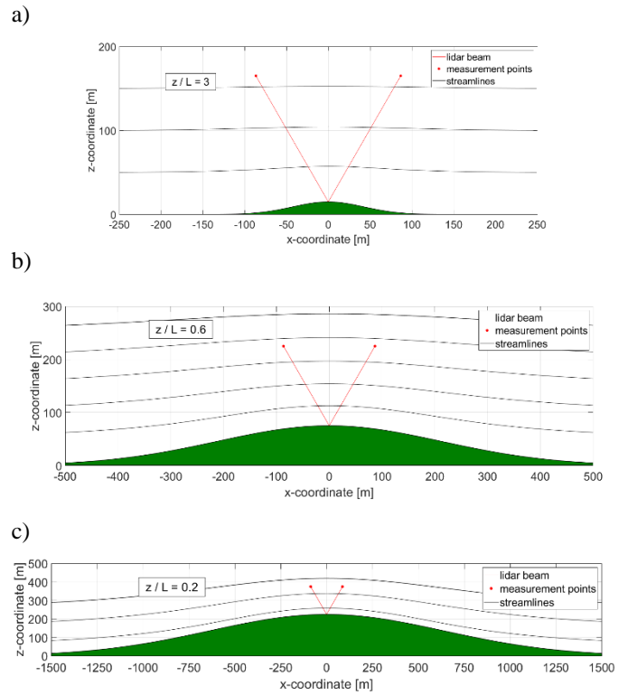
Figure 5: Left: Lidar error \varepsilon in dependence of the ratio H/L between z/L ratios from 0 to 5. Results are based on the potential flow model. Right: Results from the potential flow model for L=50 m (a), 250 m (b) and 750 m (c) for an H/L ratio of 0.3 . The lidar position is marked at the top of the hills and the beams are tilted by a half-cone opening angle \varphi=30^\circ . The measurement points are located at z=150 m above the lidar. The points, therefore, are equal to z/L ratios of 3 (a), 0.6 (b) and 0.2 (c).
