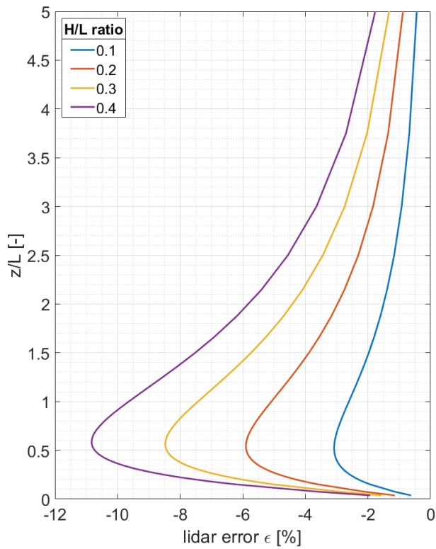
Figure 5: Left: Lidar error \varepsilon in dependence of the ratio H/L between z/L ratios from 0 to 5. Results are based on the potential flow model. Right: Results from the potential flow model for L=50 m (a), 250 m (b) and 750 m (c) for an H/L ratio of 0.3 . The lidar position is marked at the top of the hills and the beams are tilted by a half-cone opening angle \varphi=30^\circ . The measurement points are located at z=150 m above the lidar. The points, therefore, are equal to z/L ratios of 3 (a), 0.6 (b) and 0.2 (c).
