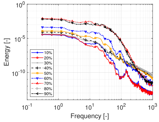
(b) PSD at TI = 1.4\% .
