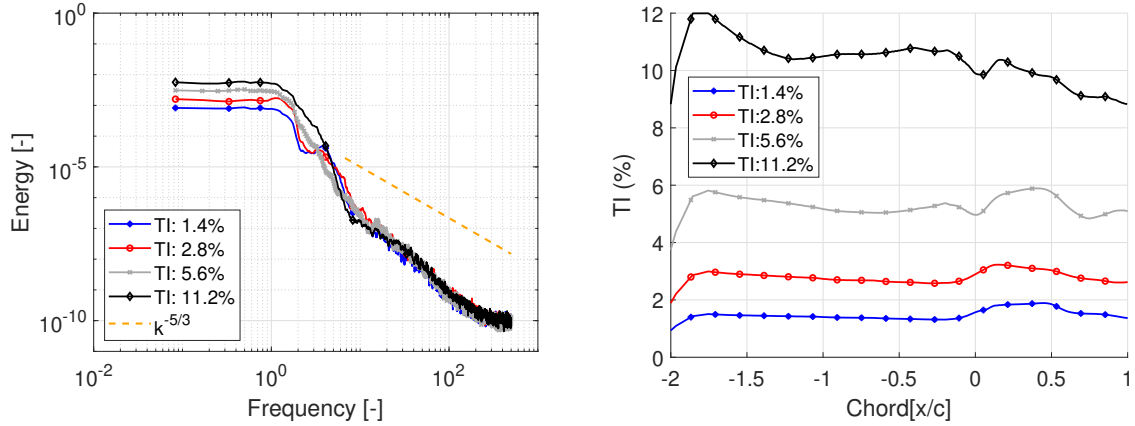
(a) Turbulent kinetic energy spectra of generated inflow turbulence. (b) Turbulence intensity development with downstream distance measured at a constant wall-normal distance corresponding to the boundary layer thickness at 50 % chord.
