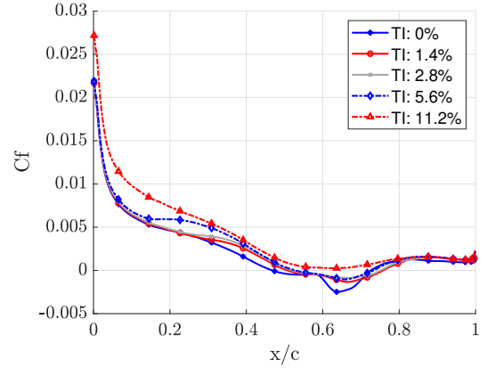
(b) Suction side friction coefficient based on the mean flow.
