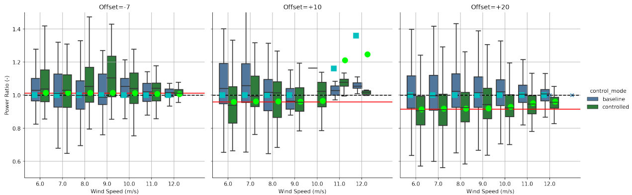
Figure 5. A comparison of power ratios of the controlled wind turbine (T5) with respect to the reference turbine (T4) for different target offsets. The power ratios are binned by wind speed and the results for baseline (blue) and controlled operation are compared. The circles indicate the expectations from the FLORIS model, whereas the red horizontal line is assuming a fixed cosine-squared loss.
