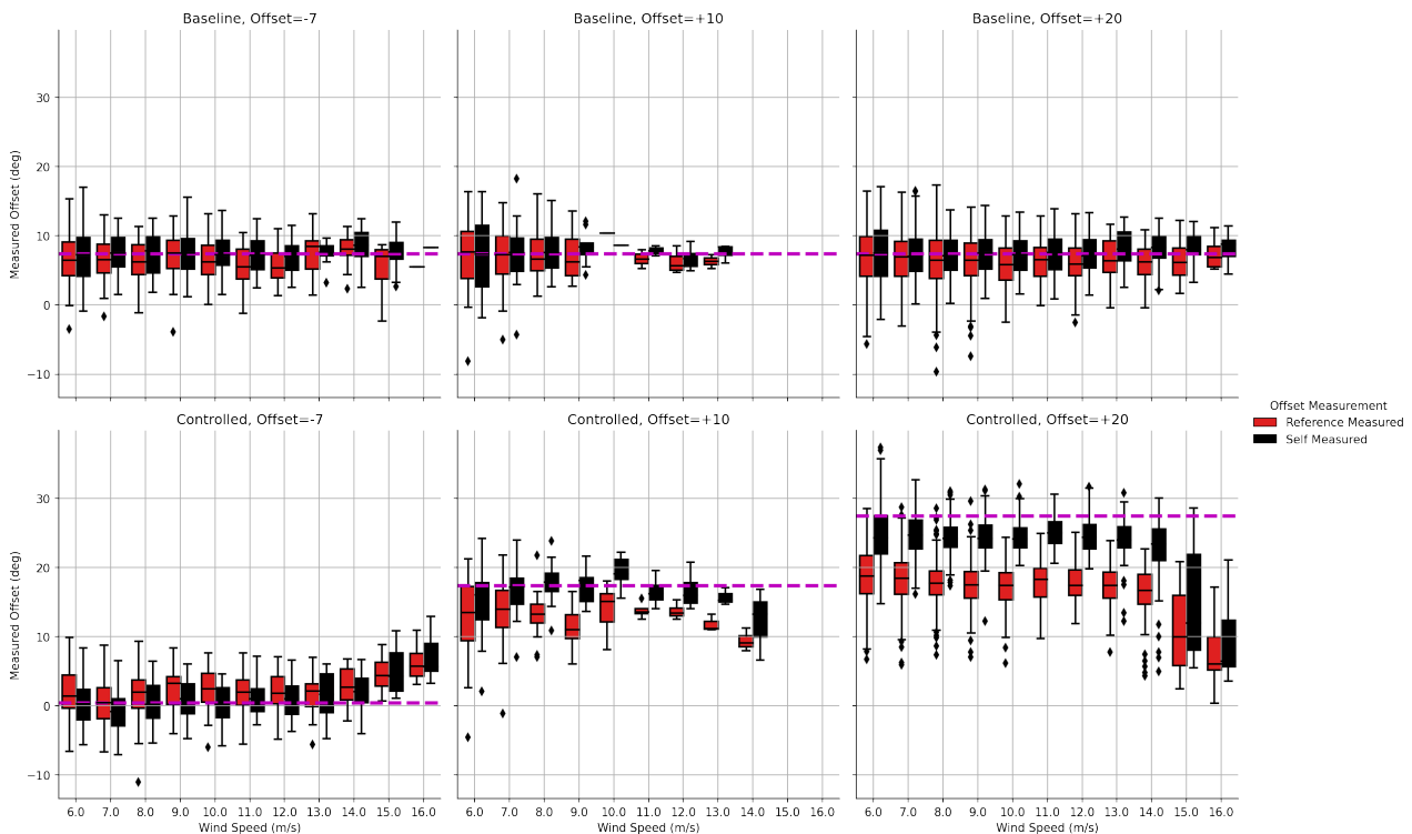
Figure 4. Boxplots, binned by wind speed, of the offset of the controlled wind turbine, as measured by its own vane (black) or in comparison to a reference wind direction (red). The targeted offset is indicated in each case with a magenta dashed line.
