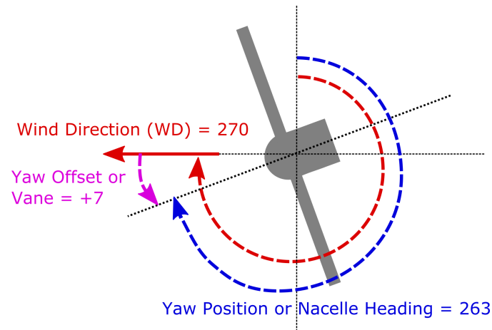
Figure 2. Illustration of conventions for the name and sign of certain direction signals. The figure illustrates what is meant by a +7-deg yaw offset.
