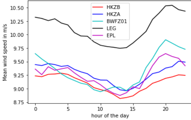
Figure 3: Intraday variability of mean wind speed at 120 m for each Lidar. The time is given in UTC, which is close to local time since Zone 1 and Zone 2 are located near the Greenwich meridian (LEG curve is higher because the campaign was performed during winter).
