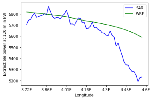
Figure 12: Extractable wind power coastal gradient at 120 m on a horizontal line at the top of Zone 2, estimated by the WRF and by SAR satellites.
