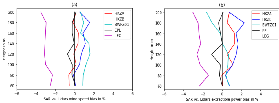
Figure 9: Biases of SAR extrapolated wind speed (a) and extractable wind power (b) versus each Lidar as a percentage. The results with Lidar LEG are less accurate due to its low number of collocated SAR samples.
