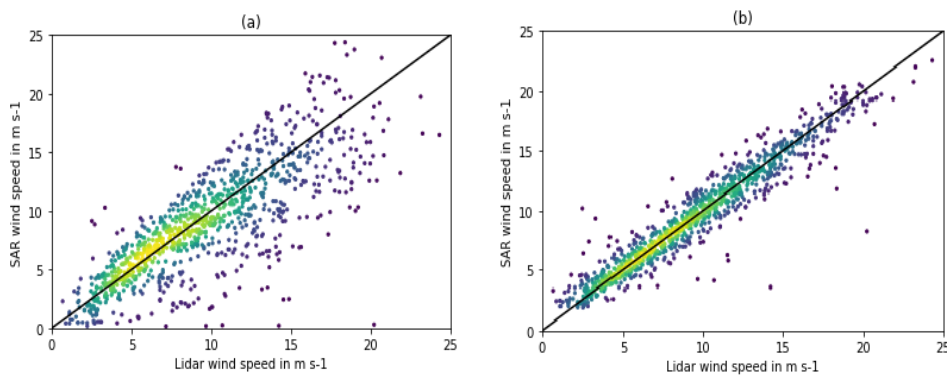
Figure 8: Scatterplots between SAR and Lidar wind speeds at 120 m above sea level when the extrapolation is performed with a classical power law (a) or with machine learning (b). The colours represent the density of points and the black curve is the identity line.
