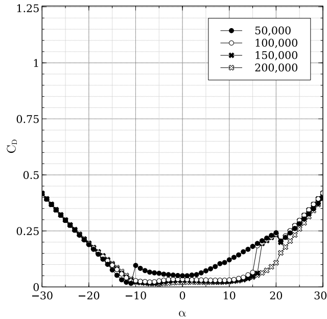
Figure 3. Drag polar for the DU06W200 airfoil at different Re .
