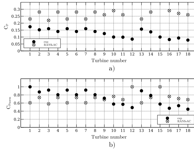
Figure 12. Power coefficients of the eighteen-turbine array.
