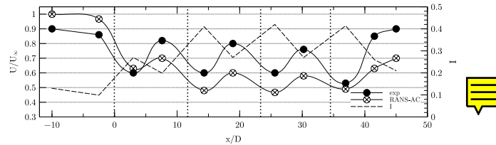
Figure 11. Wake across the turbine array. The axis for I is located at the right side of the plot. Vertical dotted lines signify the locations of each turbine.
