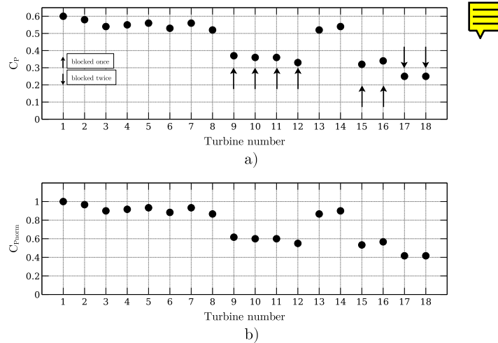
Figure 16. Wind farm array of 18 turbines using the 25 m-radius turbine from (Shamsoddin and Porté-Agel, 2016). a) shows the current C_P and b) shows the normalized C_P . Arrows pointing upwards denote turbines that are blocked by only one turbine, whereas arrows that point downwards denote turbines that have been blocked by two turbines.
