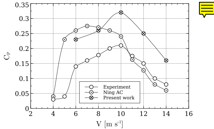
Figure 4. 1.2 kW Windspire turbine validation and comparison. \lambda is kept at 2.3 up until 10 \text{ ms}^{-1} .
