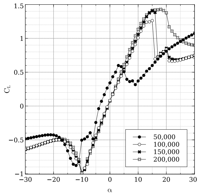
Figure 2. Lift polar for the DU06W200 airfoil at different Re .
