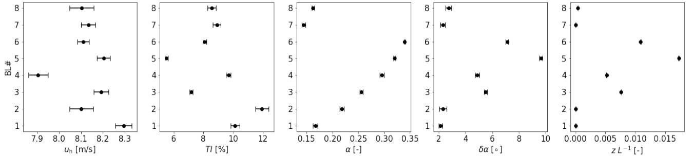
Figure 1. Summary of inflow parameters (60 min averages), given as mean (dots) and standard deviation (whiskers) over the 15 main simulations performed in each BL (5 yaw angles times 3 pitch angles). Considered are wind speed ( u_h ) and turbulence intensity at hub height ( TI ), wind shear ( \alpha ) and veer ( \delta\alpha ) over the rotor area and the Obukhov stability parameter ( z L^{-1} ) at z = 2.5 m. Equations for these variables can be found in Table 3.
