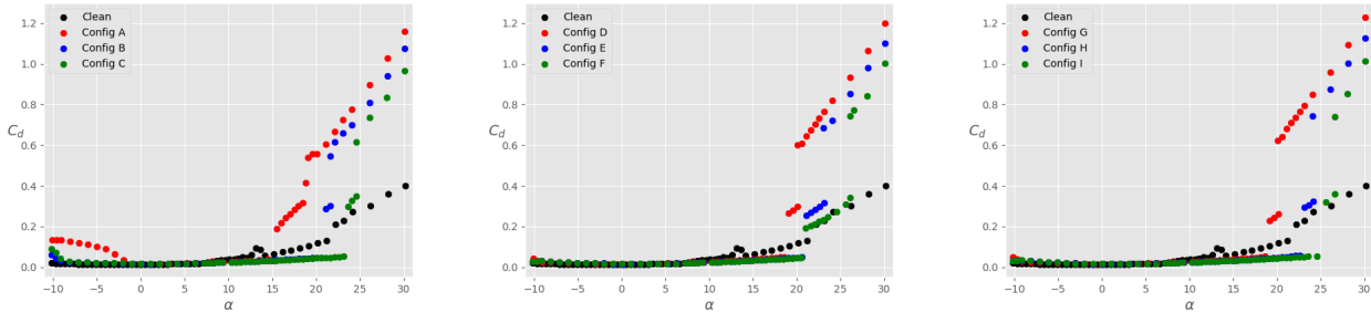
Figure 6. Total drag coefficient C_d on the ensemble airfoil+slat as a function of the angle of attack \alpha , for different slat configurations, a clean main airfoil, and Re = 1.5 \cdot 10^6 : h_{slat}/c_{main} = 0.02 (left), h_{slat}/c_{main} = 0.03 (center), h_{slat}/c_{main} = 0.04 (right). The black data are taken without slat, while the coloured data is in the presence of a slat with \beta_{slat} = 16.4^\circ (red), \beta_{slat} = 21.4^\circ (blue), \beta_{slat} = 26.4^\circ (green).
