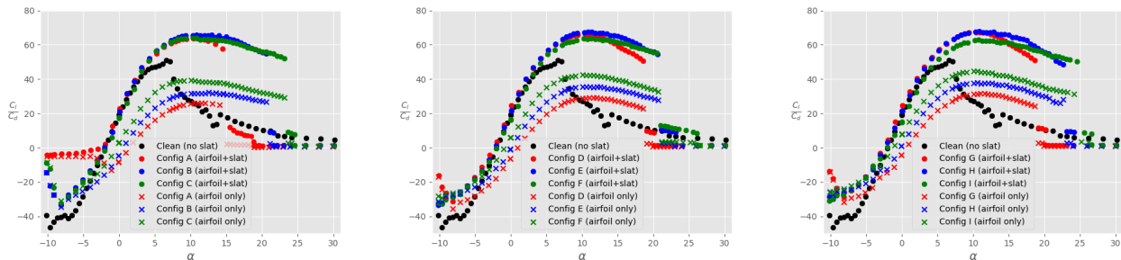
Figure 7. Lift-to-drag ratio C_l/C_d as a function of the angle of attack \alpha for different slat configurations, a clean main airfoil, and Re = 1.5 \cdot 10^6 : h_{slat}/c_{main} = 0.02 (left), h_{slat}/c_{main} = 0.03 (center), h_{slat}/c_{main} = 0.04 (right). The black data are taken without slat, while the coloured data is in the presence of a slat with \beta_{slat} = 16.4^\circ (red), \beta_{slat} = 21.4^\circ (blue), \beta_{slat} = 26.4^\circ (green). Furthermore, dots represent the total lift coefficient (main airfoil + slat), whilst the crosses show the lift force on the main airfoil only.
