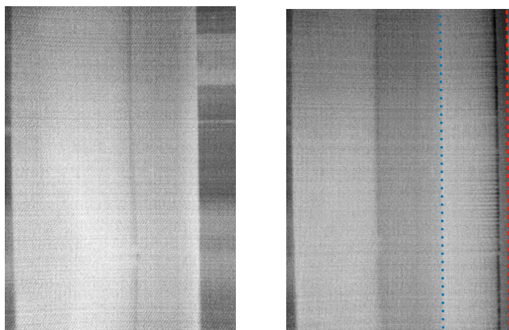
Figure 10. Infrared images of the suction side of the clean main airfoil at an angle of attack \alpha = 10^\circ : without slat (left) and with slat under configuration A (right). In the right figure, the red dashed line indicates the slat leading edge, whilst the blue dotted line shows the slat trailing edge. Flow is going from right to left.
