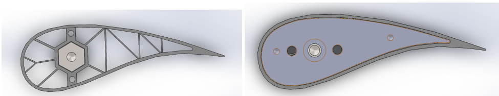
Figure 2. CAD design of the slat cross-section (left) and end plate (right).
