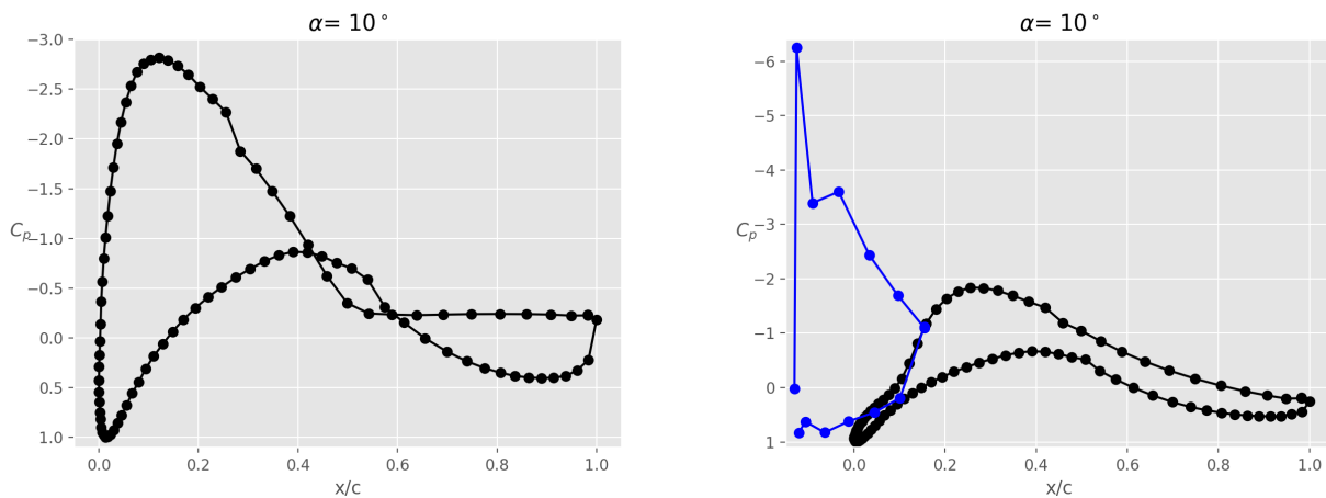
Figure 9. Pressure coefficient C_p at \alpha = 10^\circ for a clean main airfoil: main airfoil alone (left), main airfoil with slat in case A (right), where both the pressure distributions on the main airfoil (black) and slat (blue) are shown.
