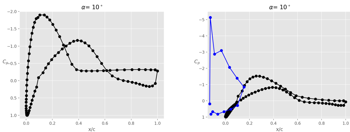
Figure 16. Pressure coefficient C_p at \alpha = 10^\circ for a tripped main airfoil: main airfoil alone (left), main airfoil with slat in case A (right), where both the pressure distributions on the main airfoil (black) and slat (blue) are shown.
