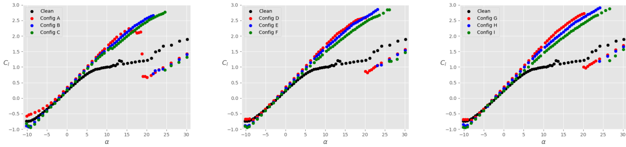
Figure 5. Total lift coefficient C_l on the ensemble airfoil+slat as a function of the angle of attack \alpha , for different slat configurations, a clean main airfoil, and Re = 1.5 \cdot 10^6 : h_{slat}/c_{main} = 0.02 (left), h_{slat}/c_{main} = 0.03 (center), h_{slat}/c_{main} = 0.04 (right). The black data are taken without slat, while the coloured data is in the presence of a slat with \beta_{slat} = 16.4^\circ (red), \beta_{slat} = 21.4^\circ (blue), \beta_{slat} = 26.4^\circ (green).
