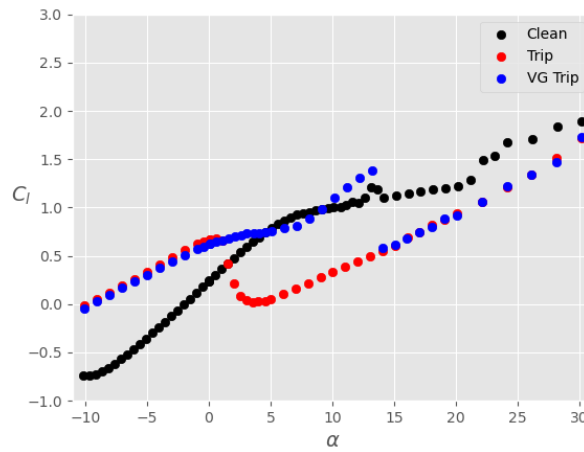
Figure 12. Lift coefficient C_l as a function of the angle of attack \alpha for a main element without slat: clean airfoil without VGs (black), tripped airfoil without VGs (red), tripped airfoil with VGs (blue).
