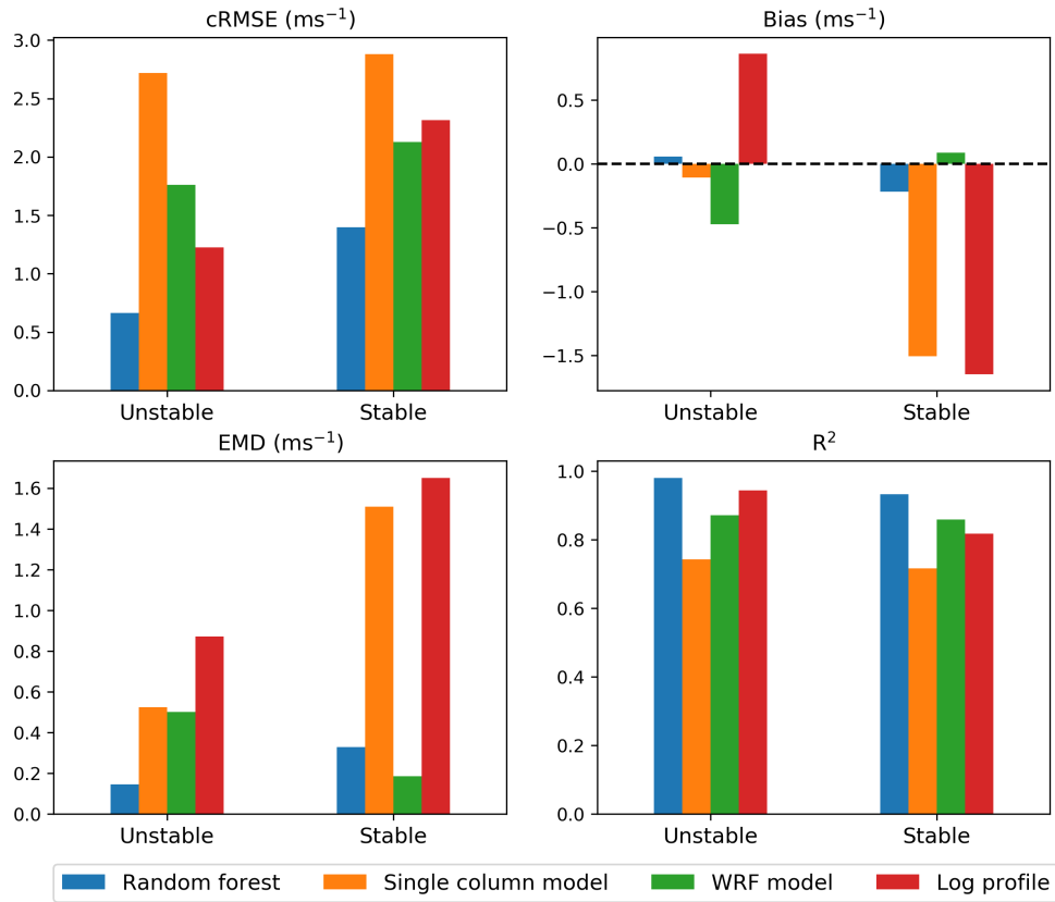
Figure 7. REWS performance metrics for the different vertical extrapolation models at NYSEERDA buoy E05 for unstable and stable conditions
