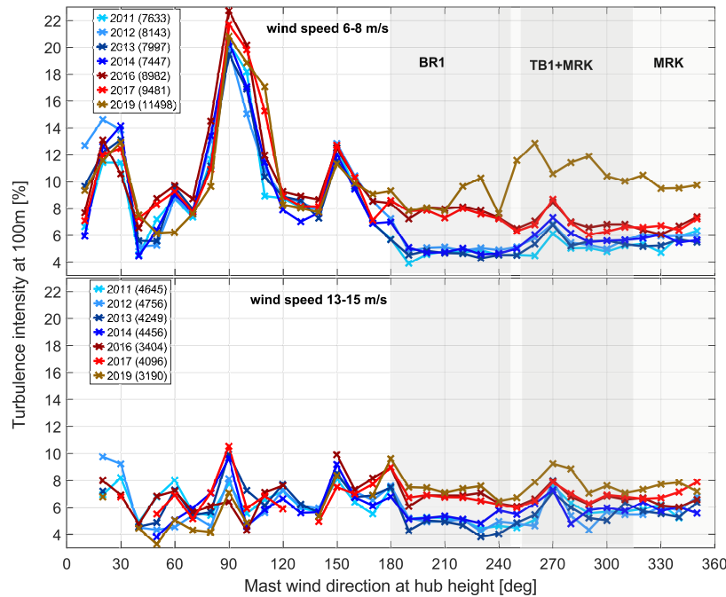
Figure 7. Turbulence intensity mean values per direction for the different years. The upper plot shows data for the 6-8 m/s wind speed bin and the lower for the 13-15 m/s bin. The shadowed areas indicate the azimuth sectors influenced by the denoted wind farms. The numbers in the legend indicate the amount of measurements used for each year
