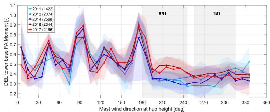
Figure 13. Mean value of damage equivalent loads at the tower bottom, for the fore-aft direction, per wind direction for the different years. Wind speed is 6-8 m/s. The band represents the 15 th and 85 th percentiles. The numbers in the legend indicate the amount of measurements used for each year. The shadowed areas indicate the azimuth sectors influenced by the denoted wind farms.
