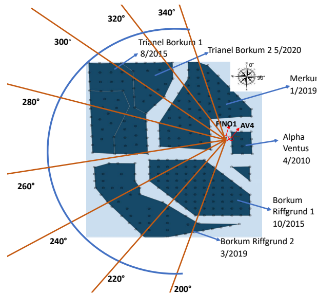
Figure 2. Azimuth sectors of focus and wind farms orientation layout. Background layer used with permission from 4C Offshore
