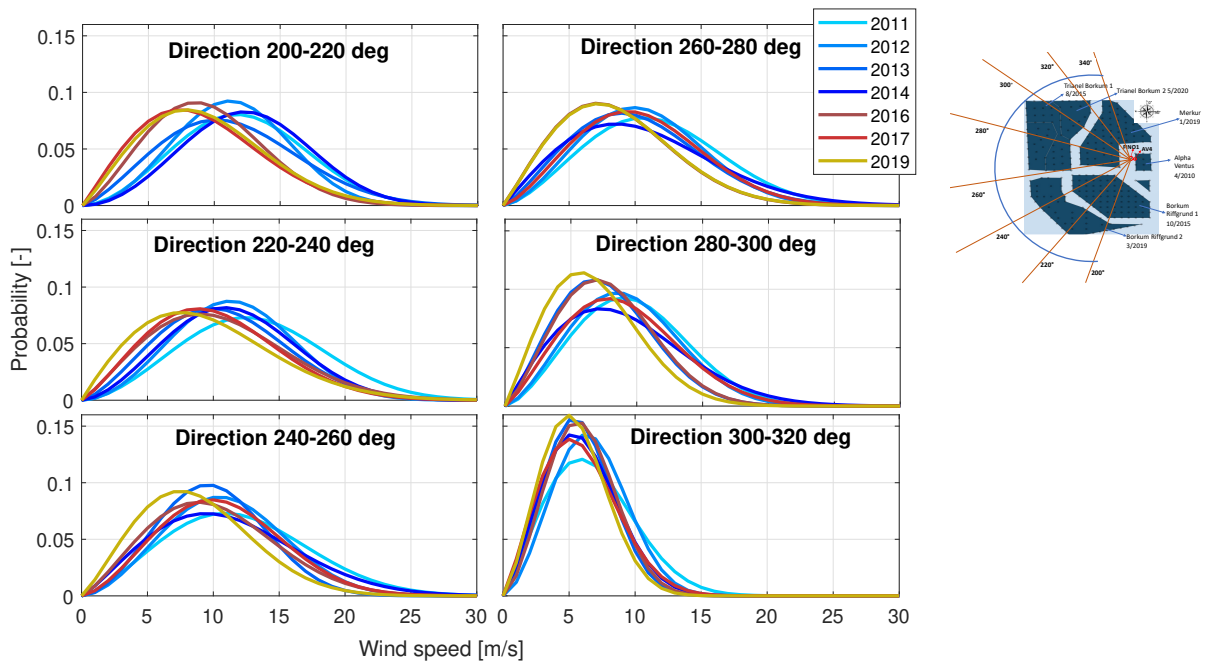
Figure 5. Fitted wind speed Weibull distributions per year and azimuth direction
