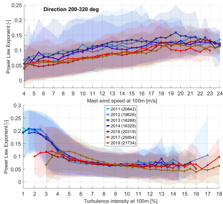
Figure 9. Fitted shear power law exponent at FINO1. Upper plot: Mean wind shear power law exponent versus wind speed, considering all levels of turbulence intensity. Lower plot: Mean wind shear power law exponent versus turbulence intensity including all wind speeds. The band represents the 15 th and 85 th percentiles. The numbers in the legend indicate the amount of measurements used for each year
